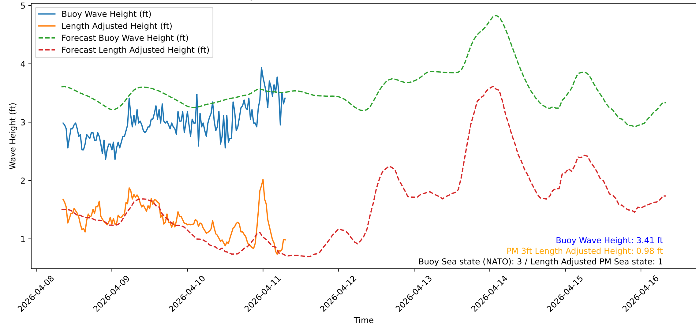
Wave Heights over Time for Green Beach at 2026-04-11 08:21:13
