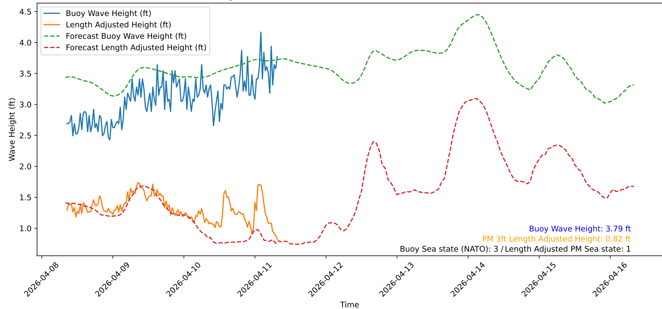
Wave Heights over Time for Oceanside Harbor at 2026-04-11 08:20:31
