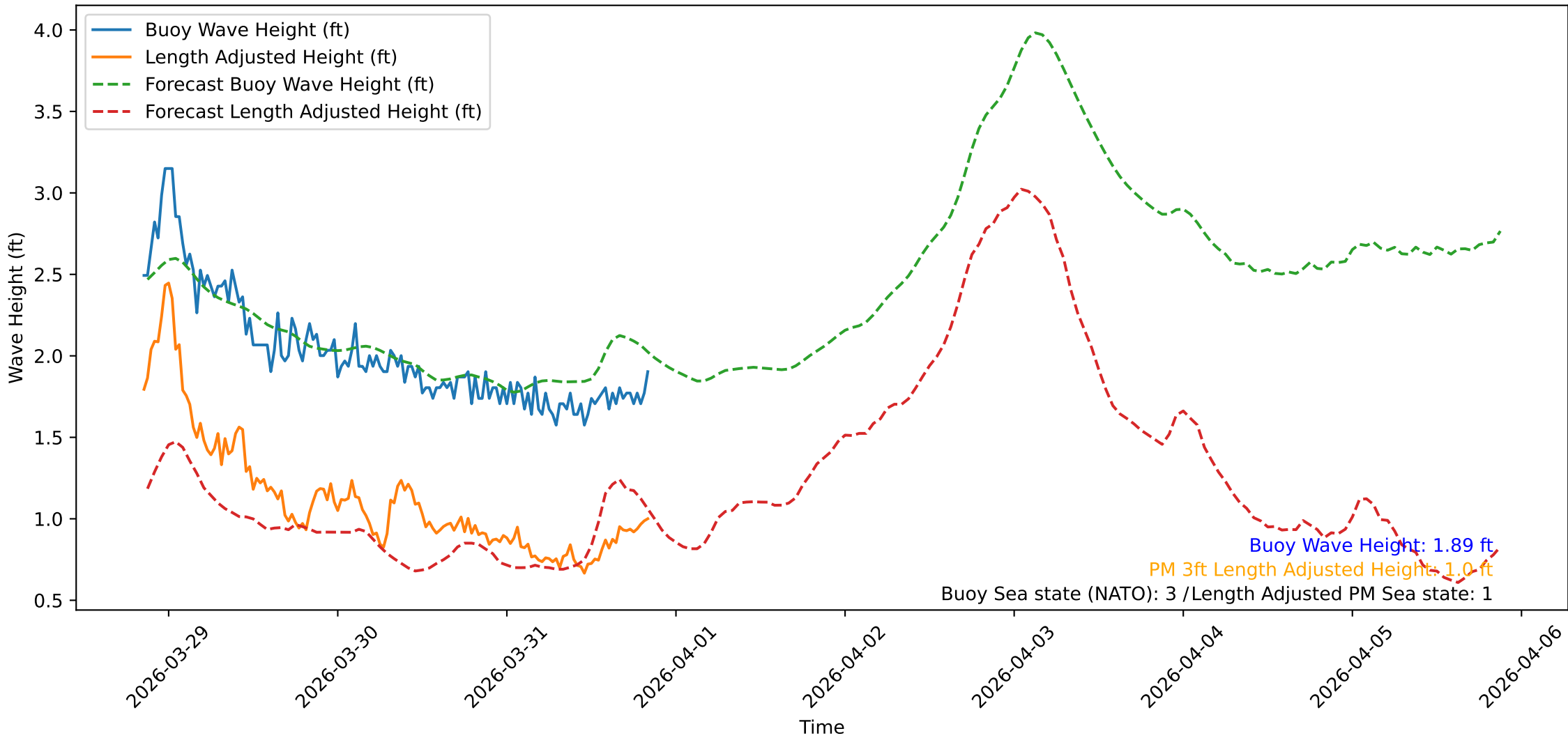
Wave Heights over Time for Oceanside Harbor at 2026-03-31 20:40:31
