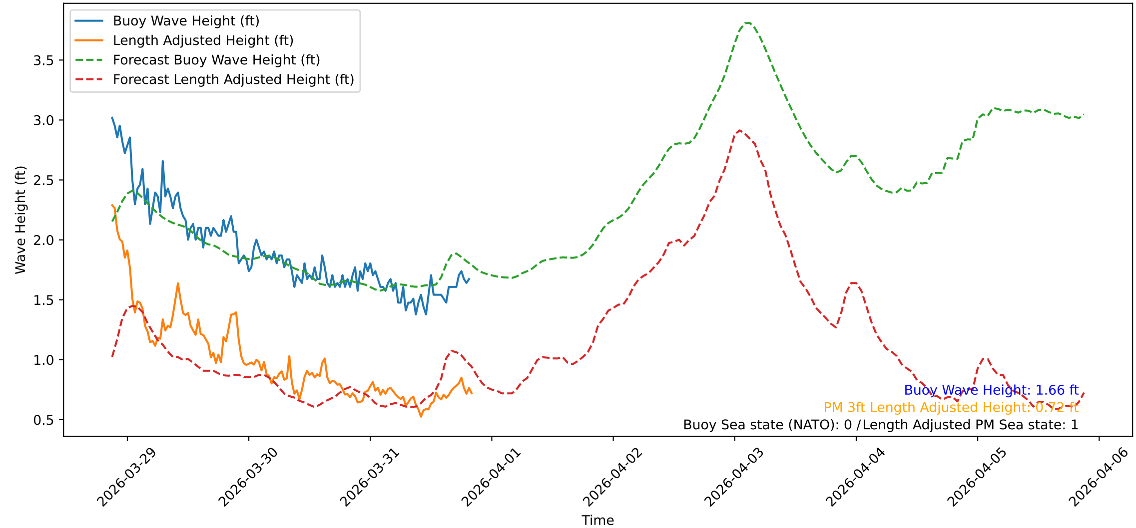
Wave Heights over Time for Red Beach at 2026-03-31 20:40:47
