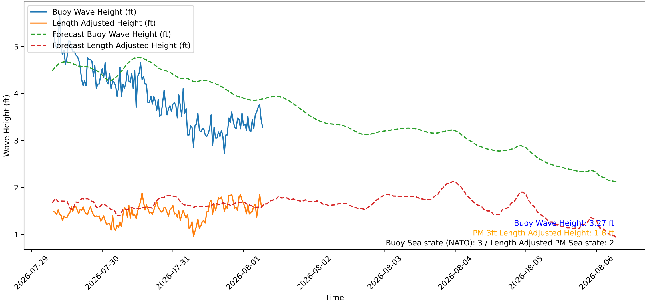
Wave Heights over Time for Oceanside Harbor at 2026-08-01 07:20:27
