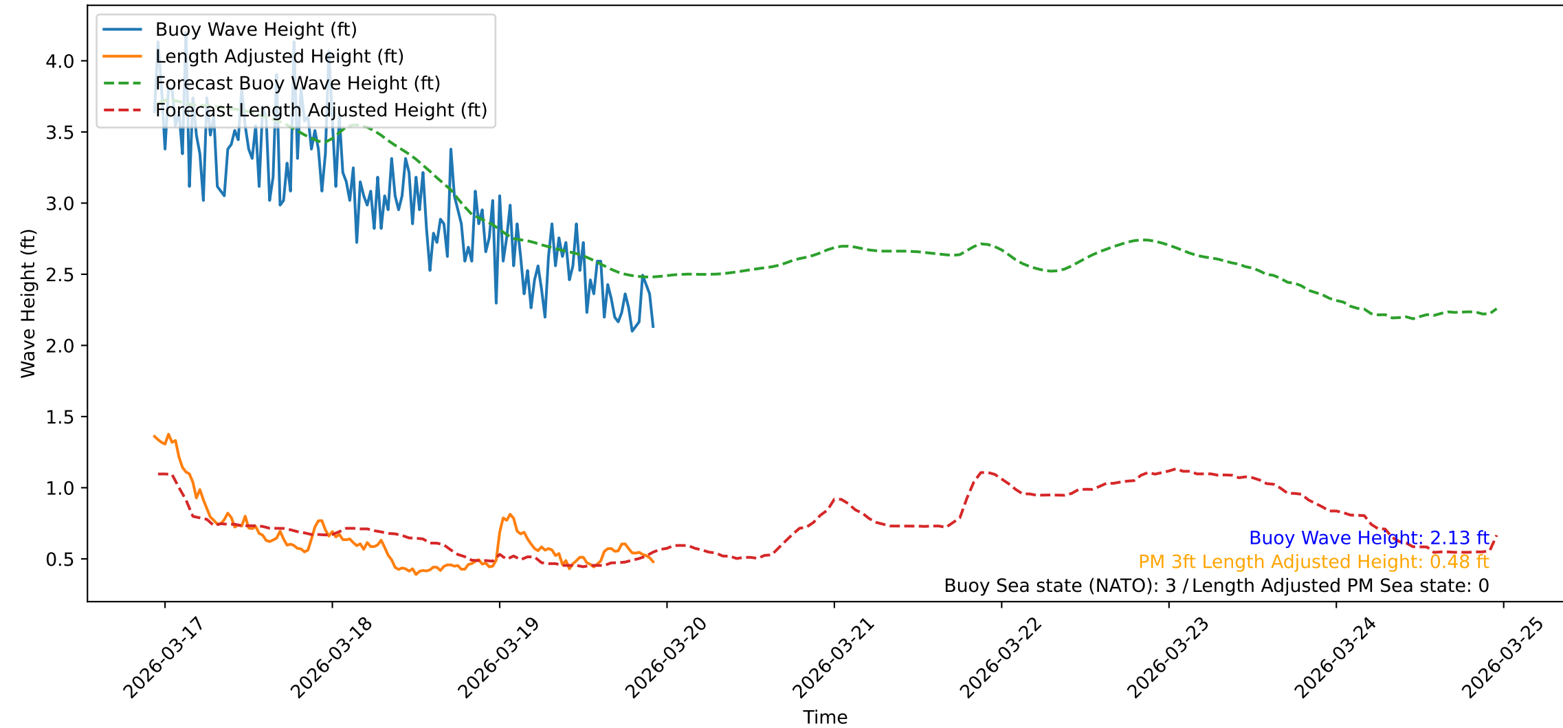
Wave Heights over Time for Green Beach at 2026-03-19 22:41:10
