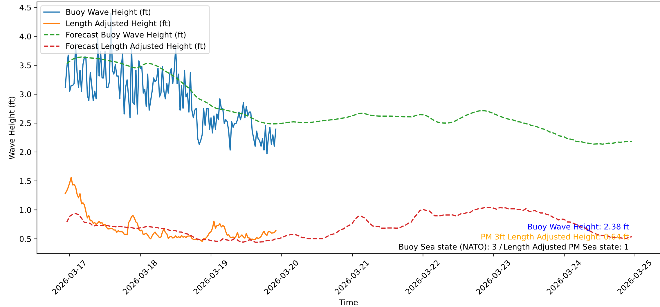
Wave Heights over Time for Oceanside Harbor at 2026-03-19 22:40:31
