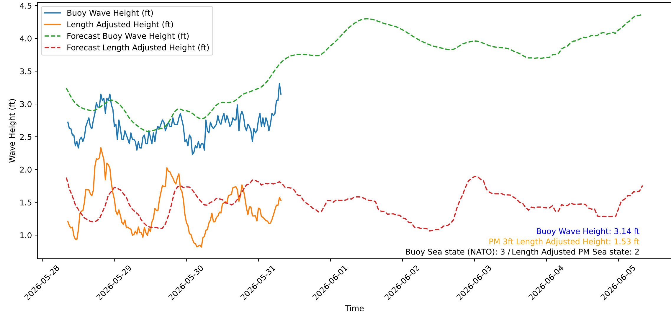
Wave Heights over Time for Red Beach at 2026-05-31 08:20:45
