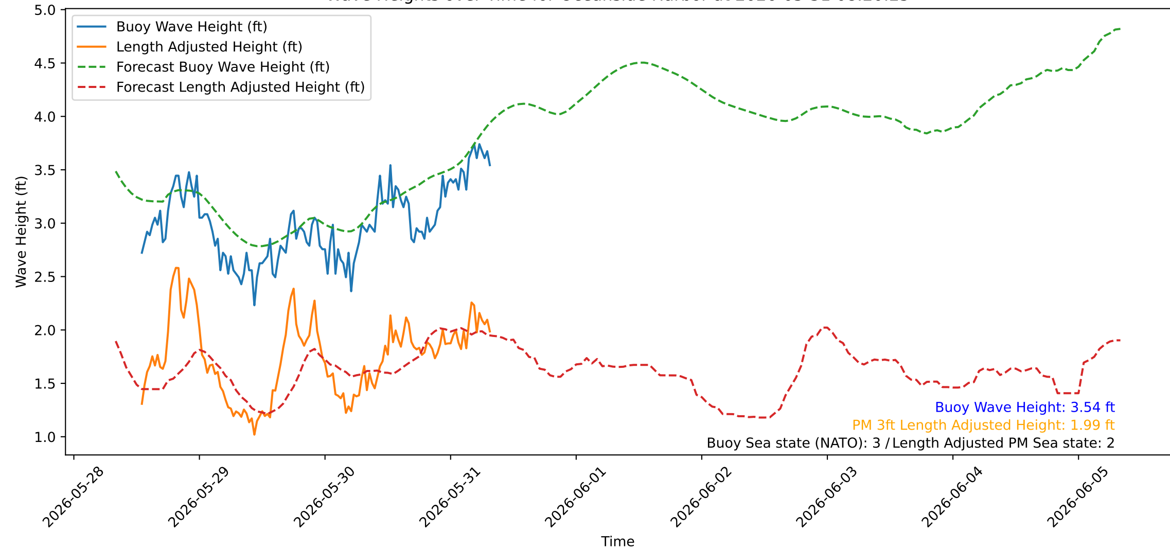
Wave Heights over Time for Oceanside Harbor at 2026-05-31 08:20:25
