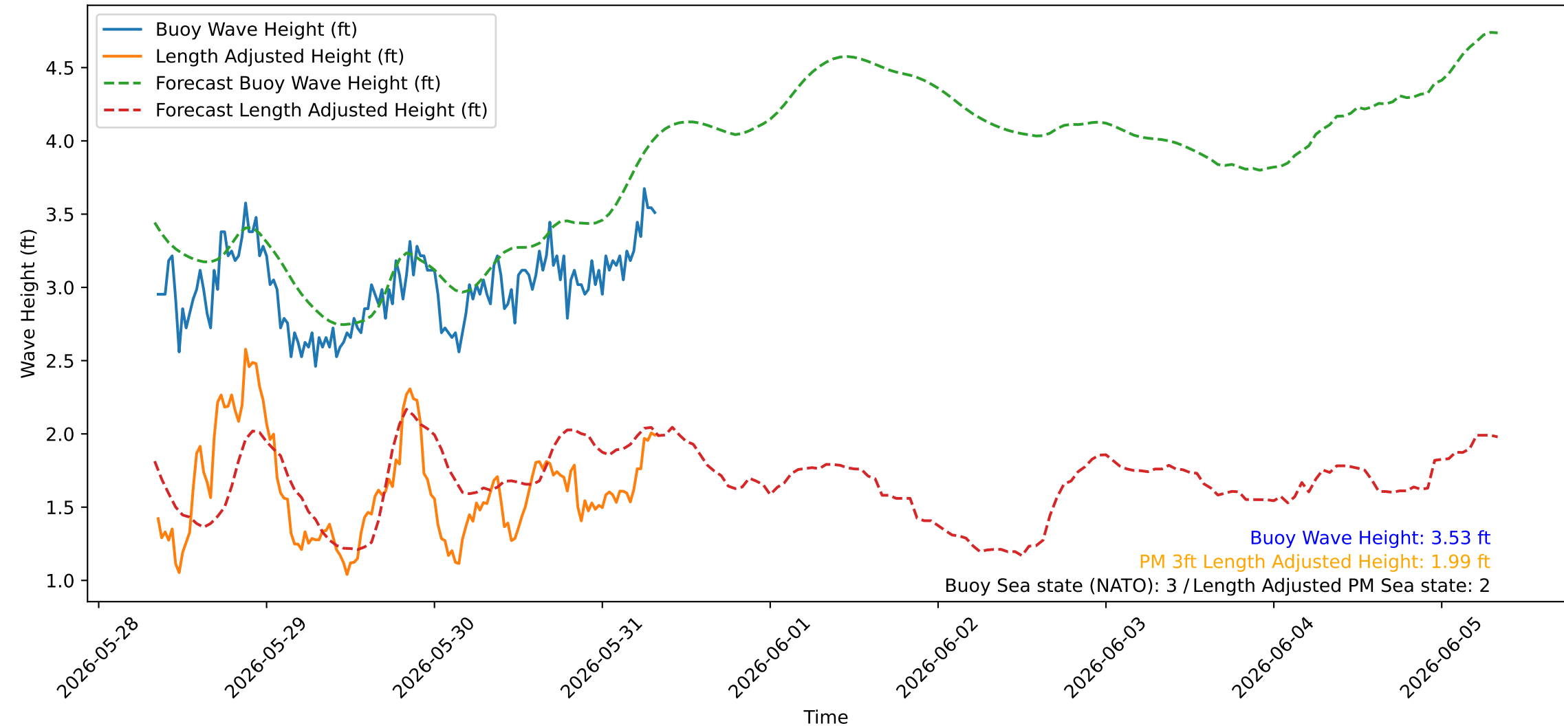
Wave Heights over Time for Green Beach at 2026-05-31 08:21:08
