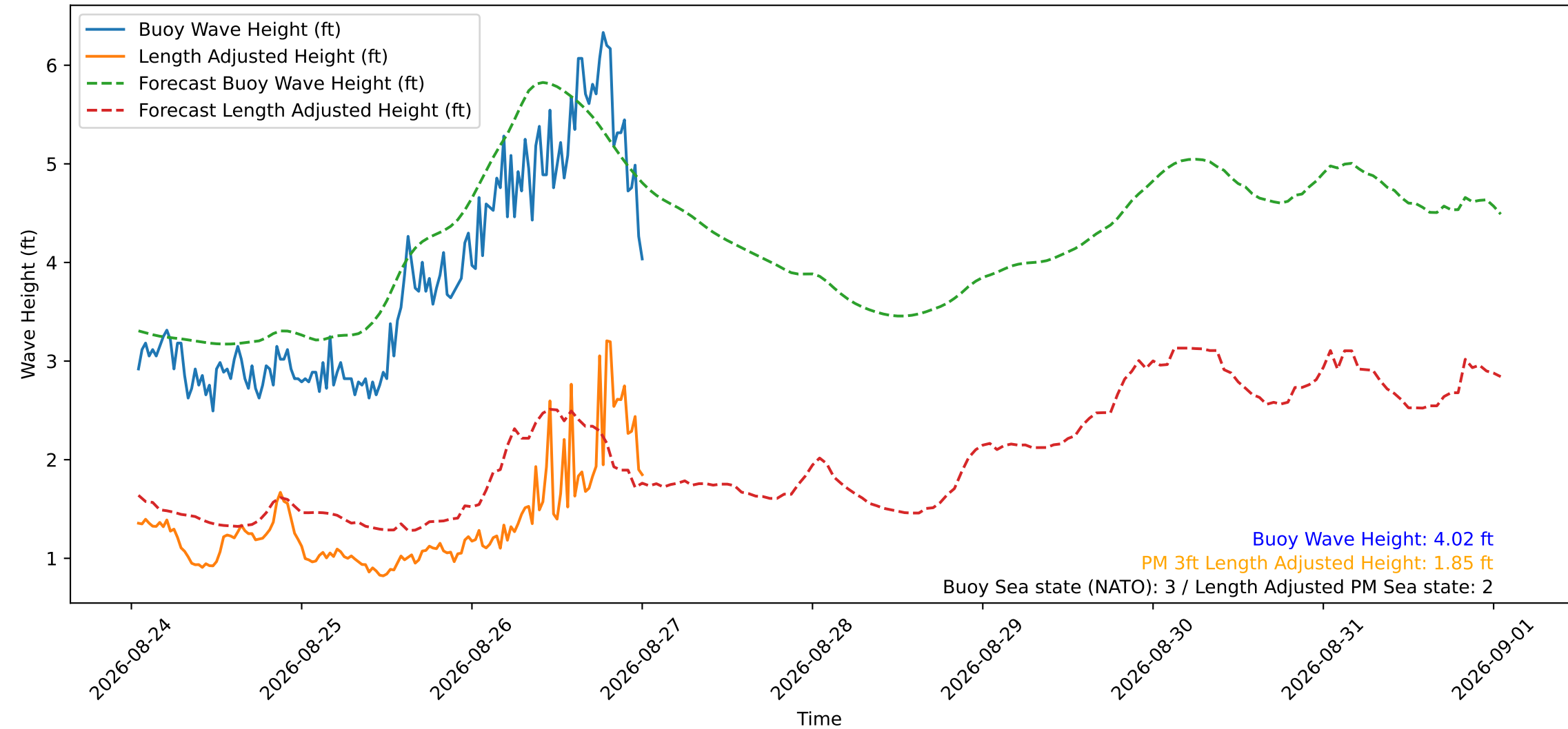
Wave Heights over Time for Green Beach at 2026-08-27 00:41:12
