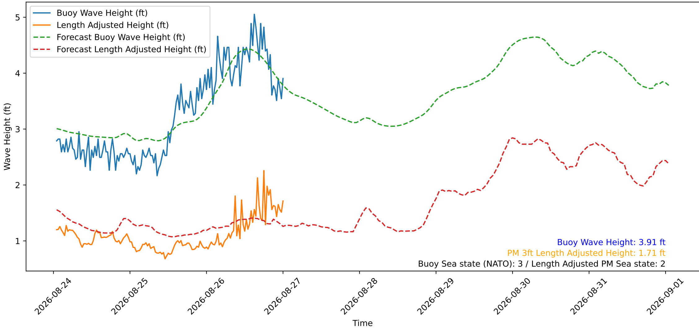
Wave Heights over Time for Red Beach at 2026-08-27 00:40:50
