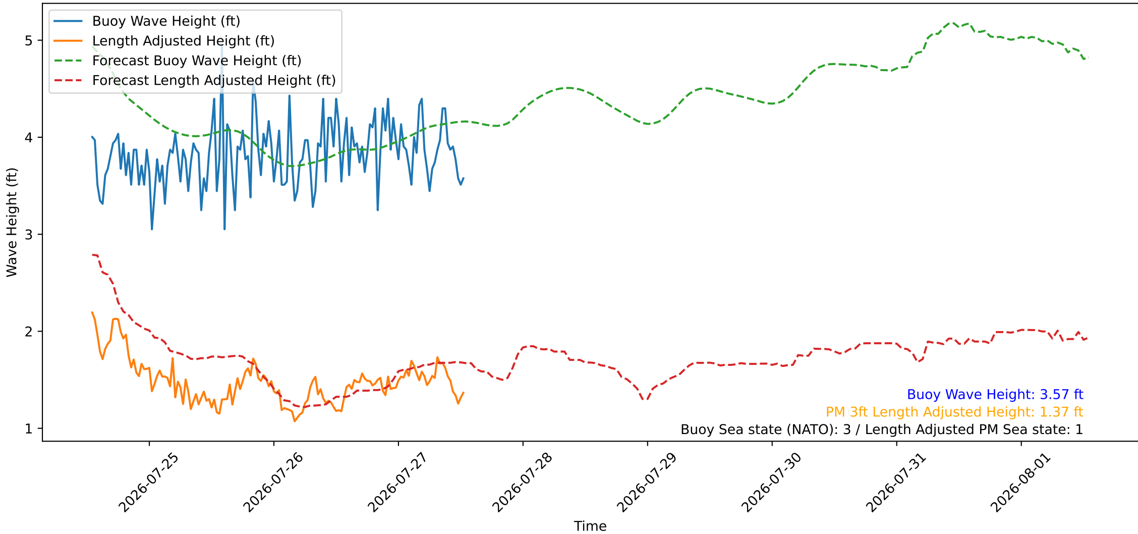
Wave Heights over Time for Oceanside Harbor at 2026-07-27 13:10:26
