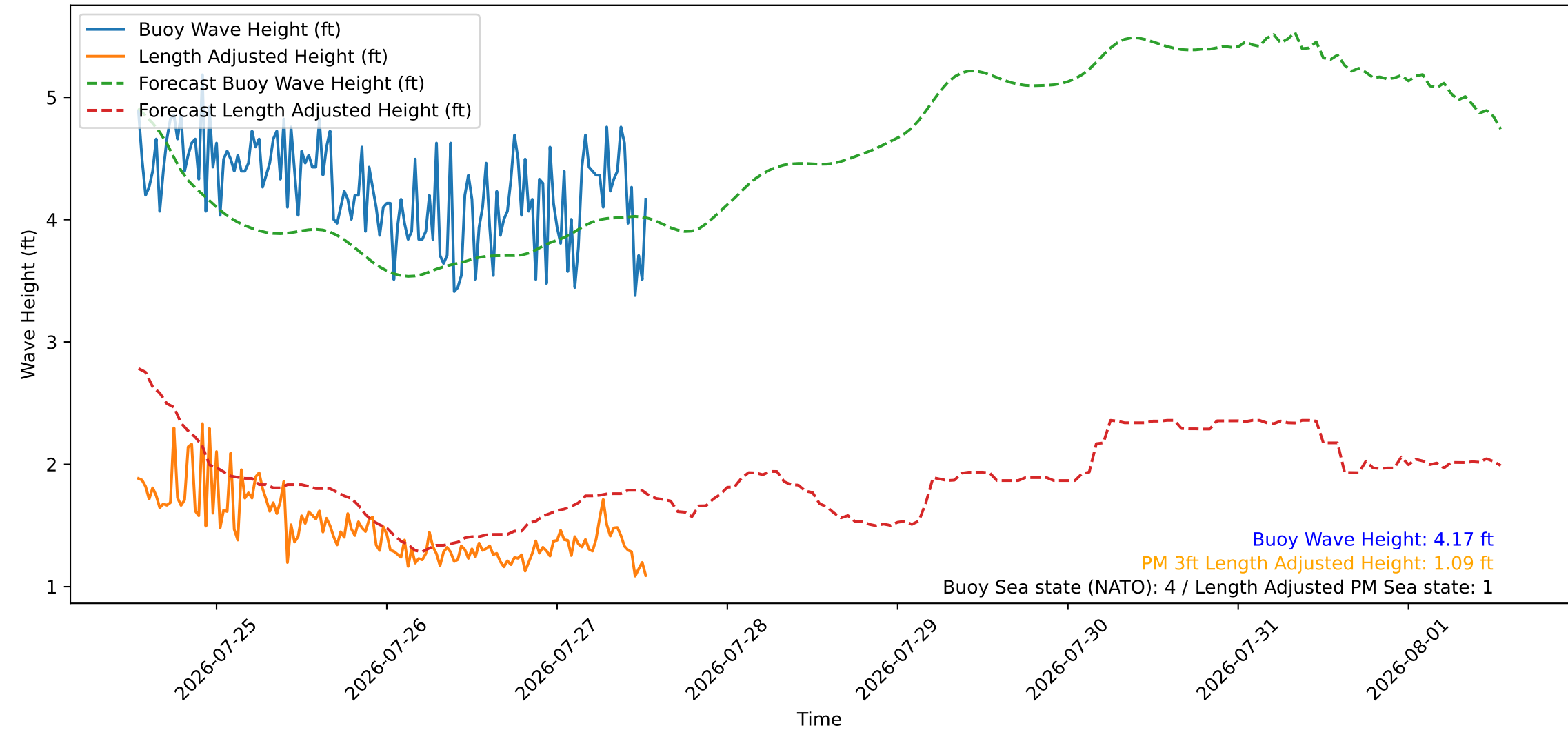
Wave Heights over Time for Green Beach at 2026-07-27 13:11:09
