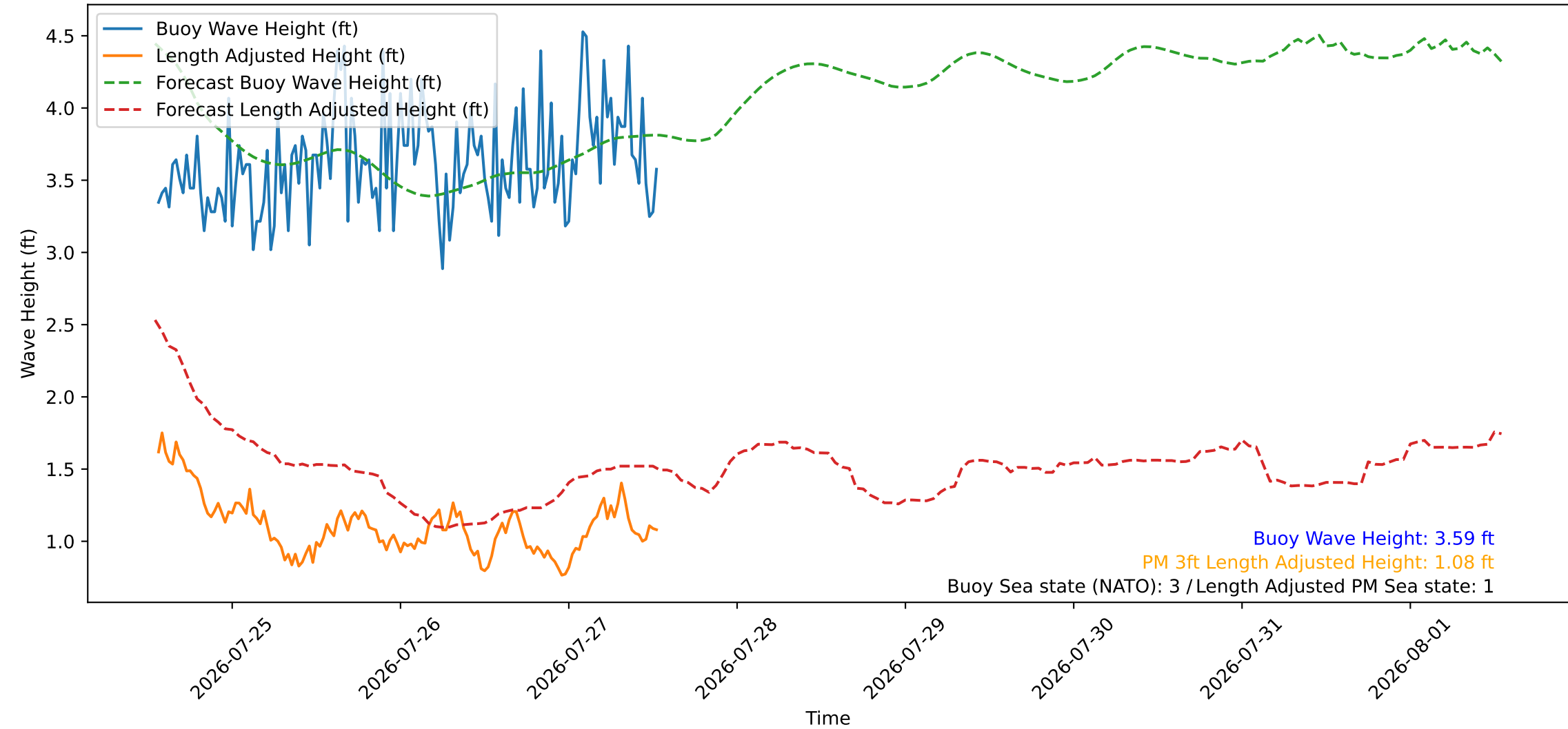
Wave Heights over Time for Red Beach at 2026-07-27 13:10:46
