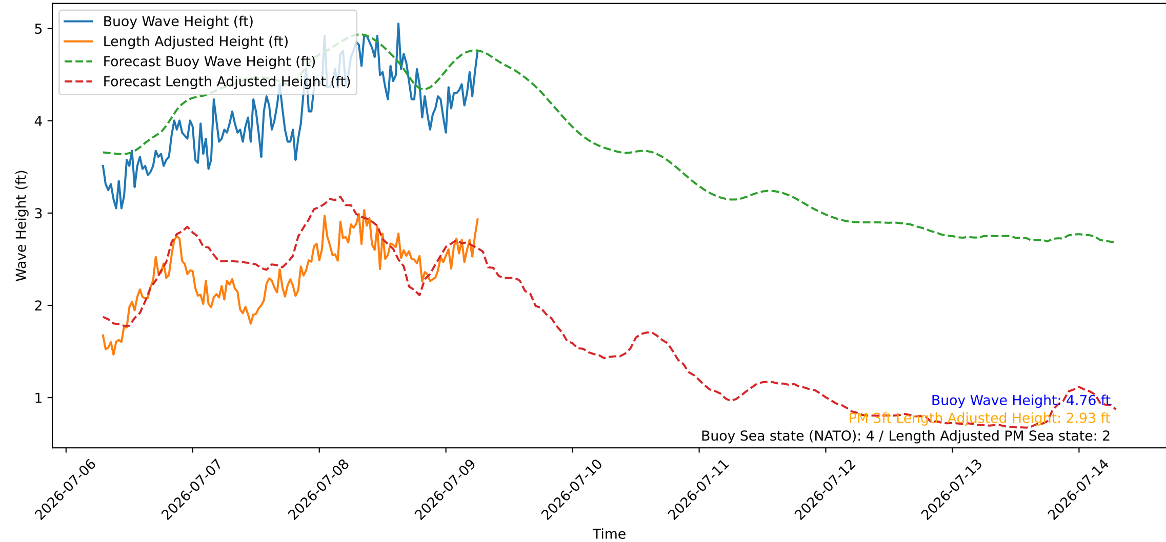
Wave Heights over Time for Oceanside Harbor at 2026-07-09 06:50:27
