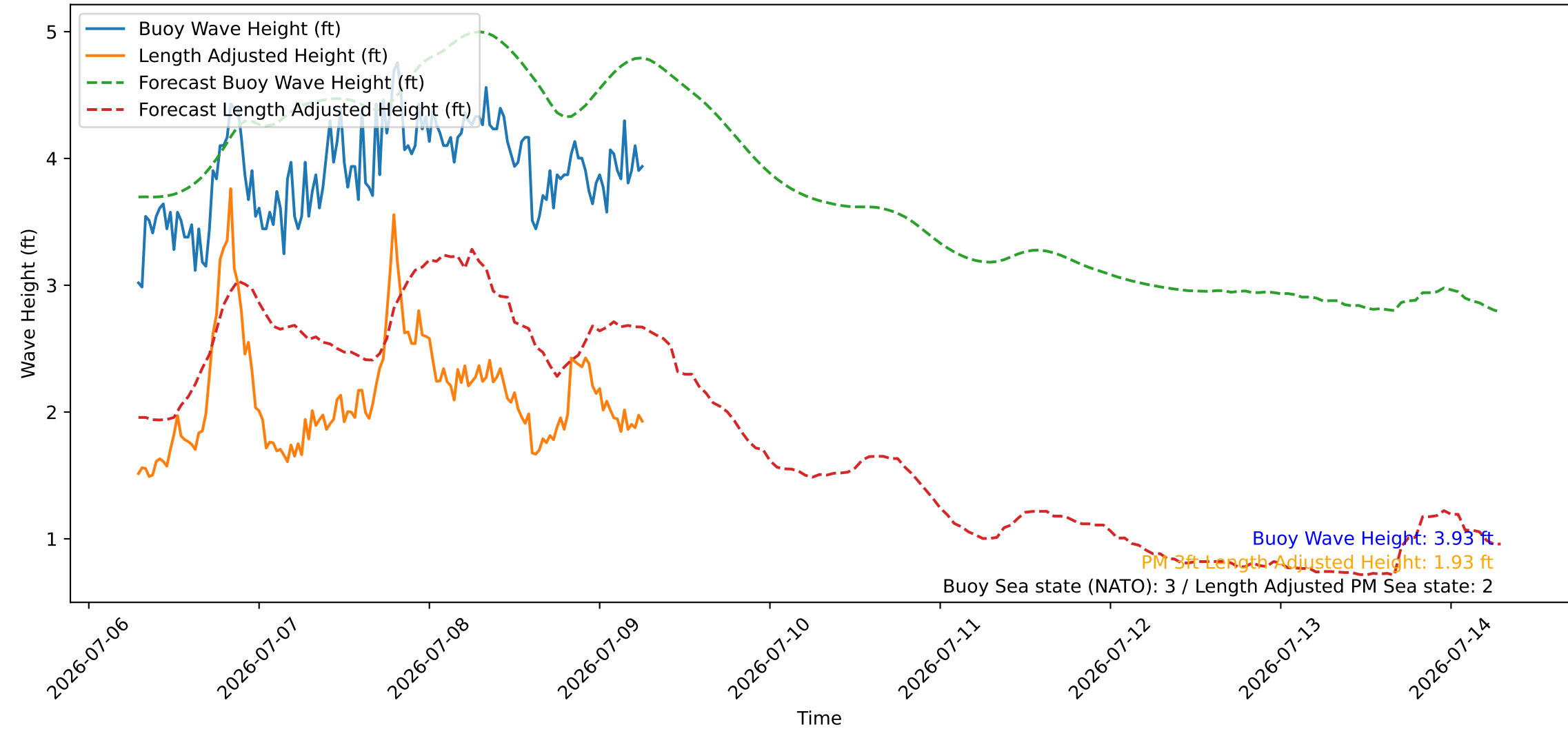
Wave Heights over Time for Green Beach at 2026-07-09 06:51:10
