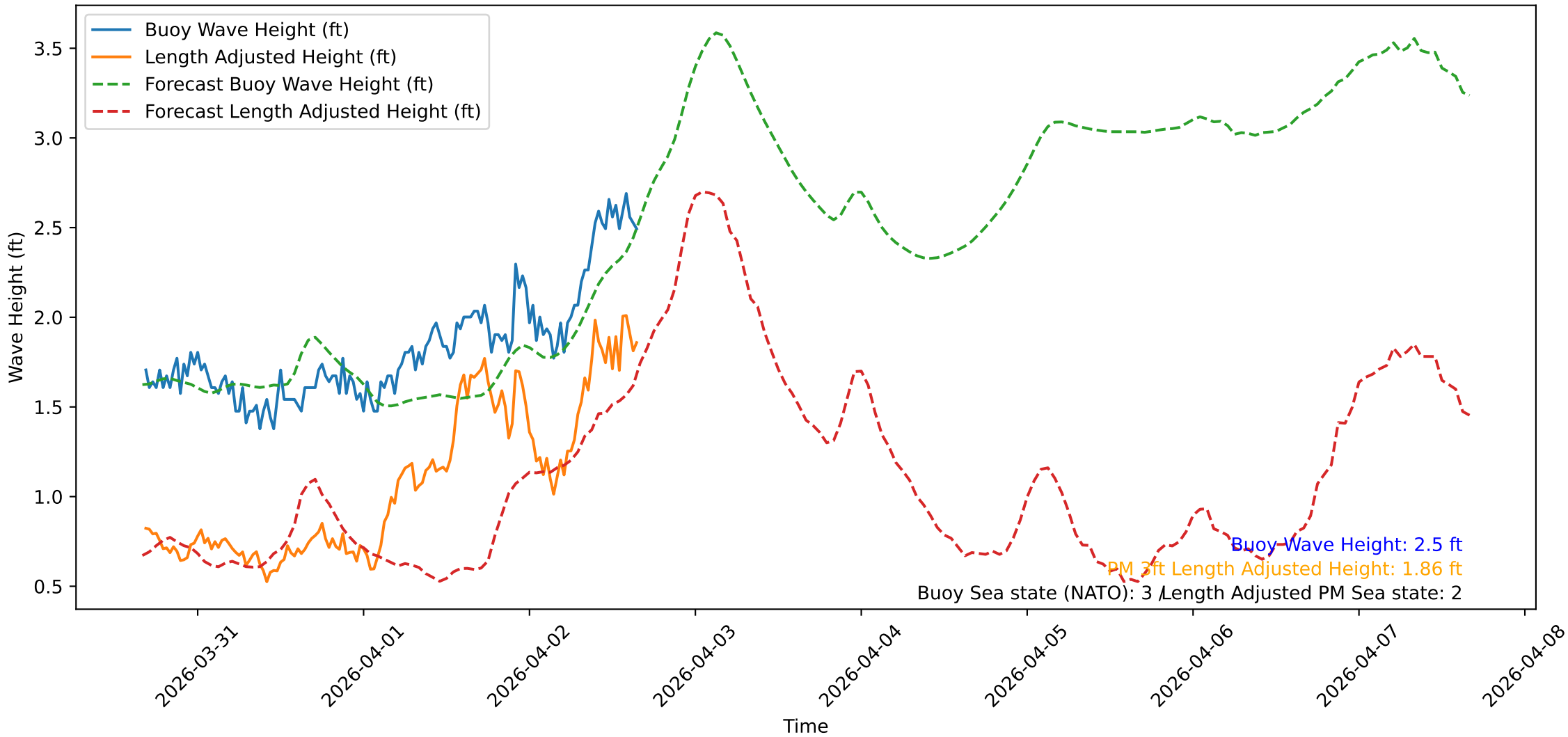
Wave Heights over Time for Red Beach at 2026-04-02 16:20:47
