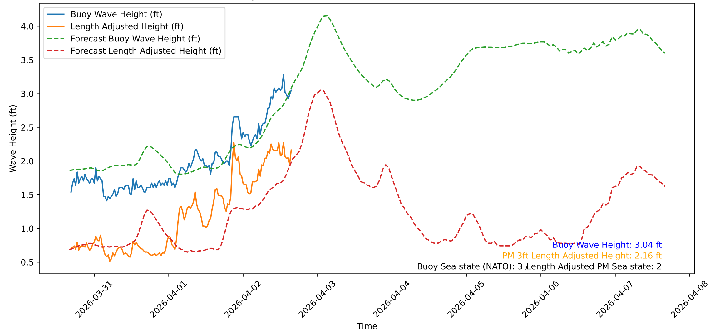
Wave Heights over Time for Green Beach at 2026-04-02 16:21:10
