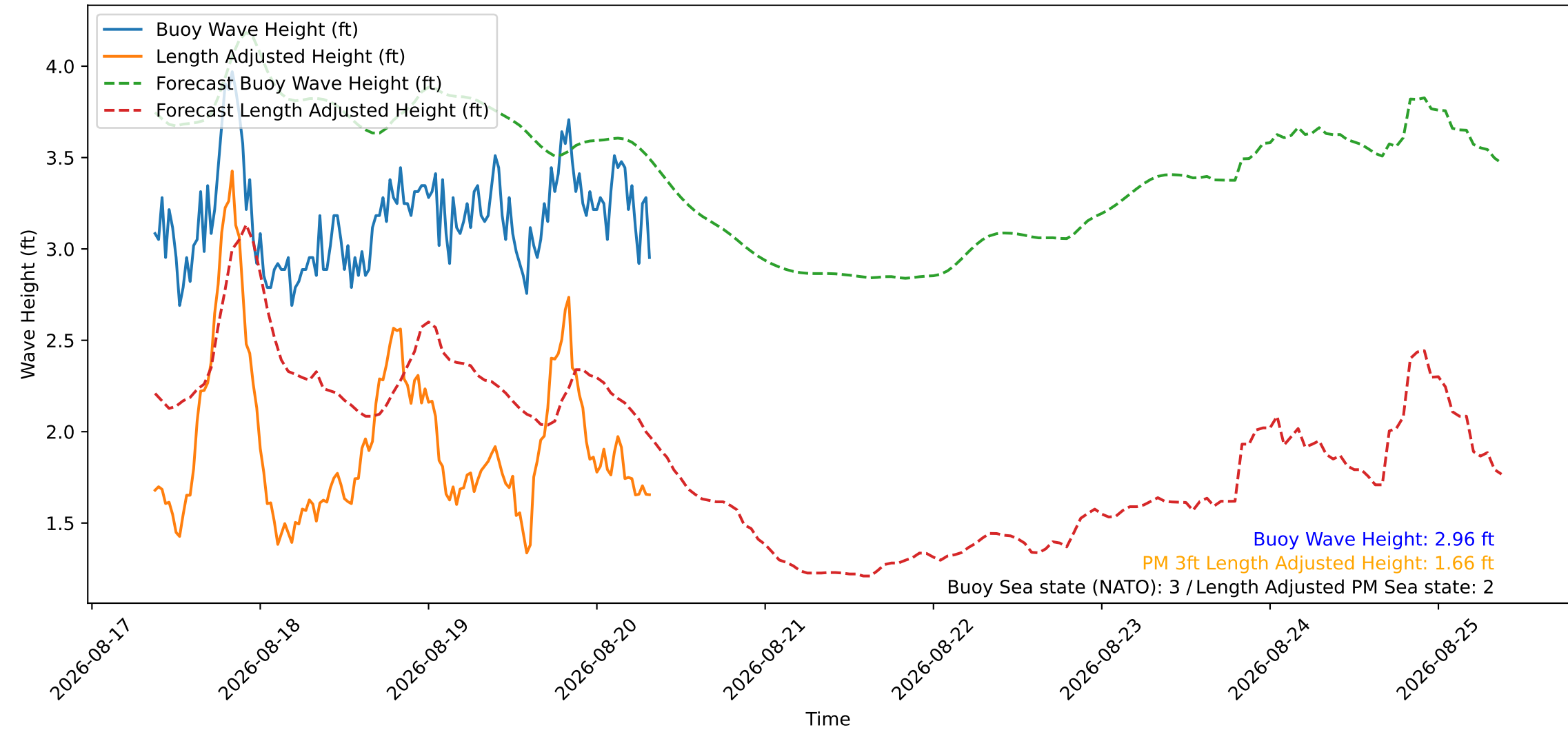
Wave Heights over Time for Green Beach at 2026-08-20 08:31:08
