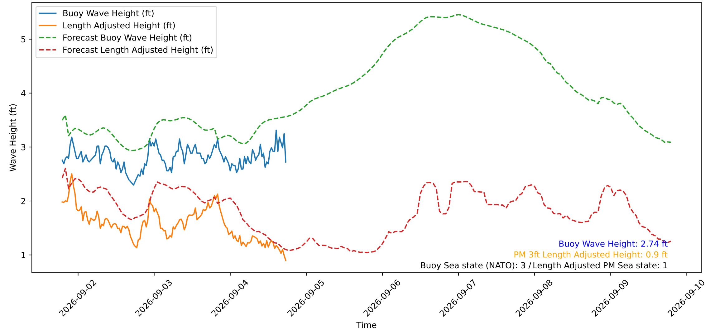
Wave Heights over Time for Red Beach at 2026-09-04 18:30:50
