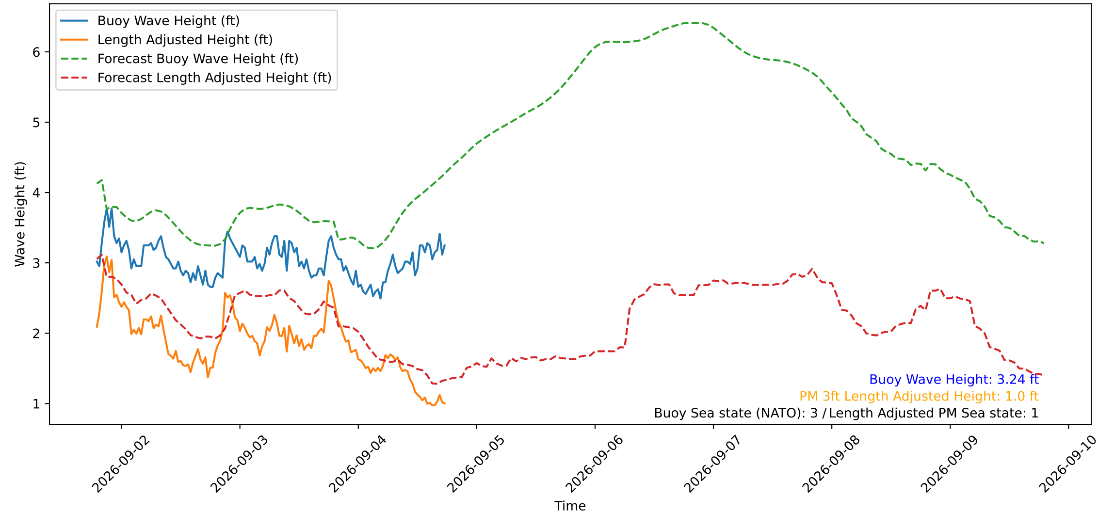
Wave Heights over Time for Green Beach at 2026-09-04 18:31:12
