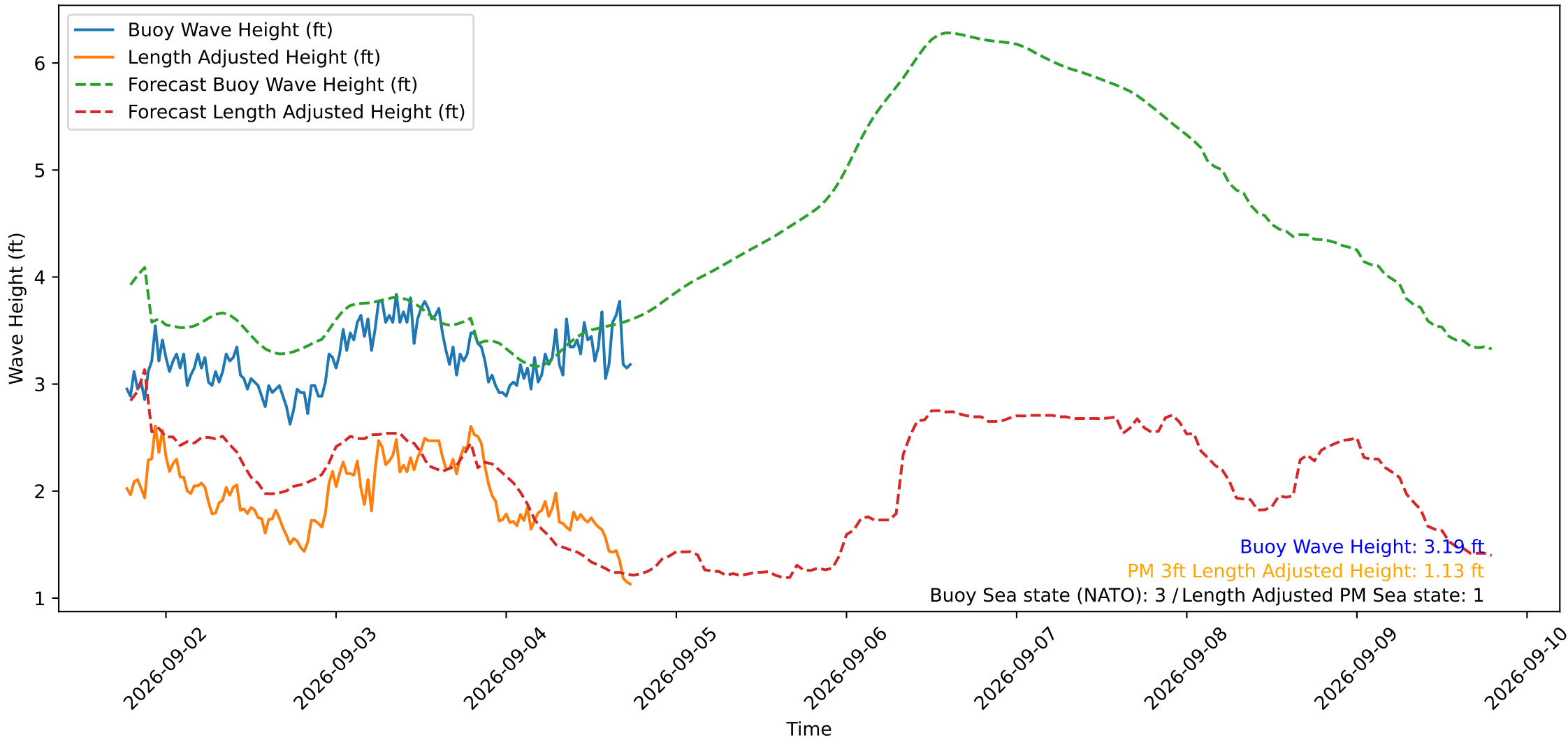
Wave Heights over Time for Oceanside Harbor at 2026-09-04 18:30:29
