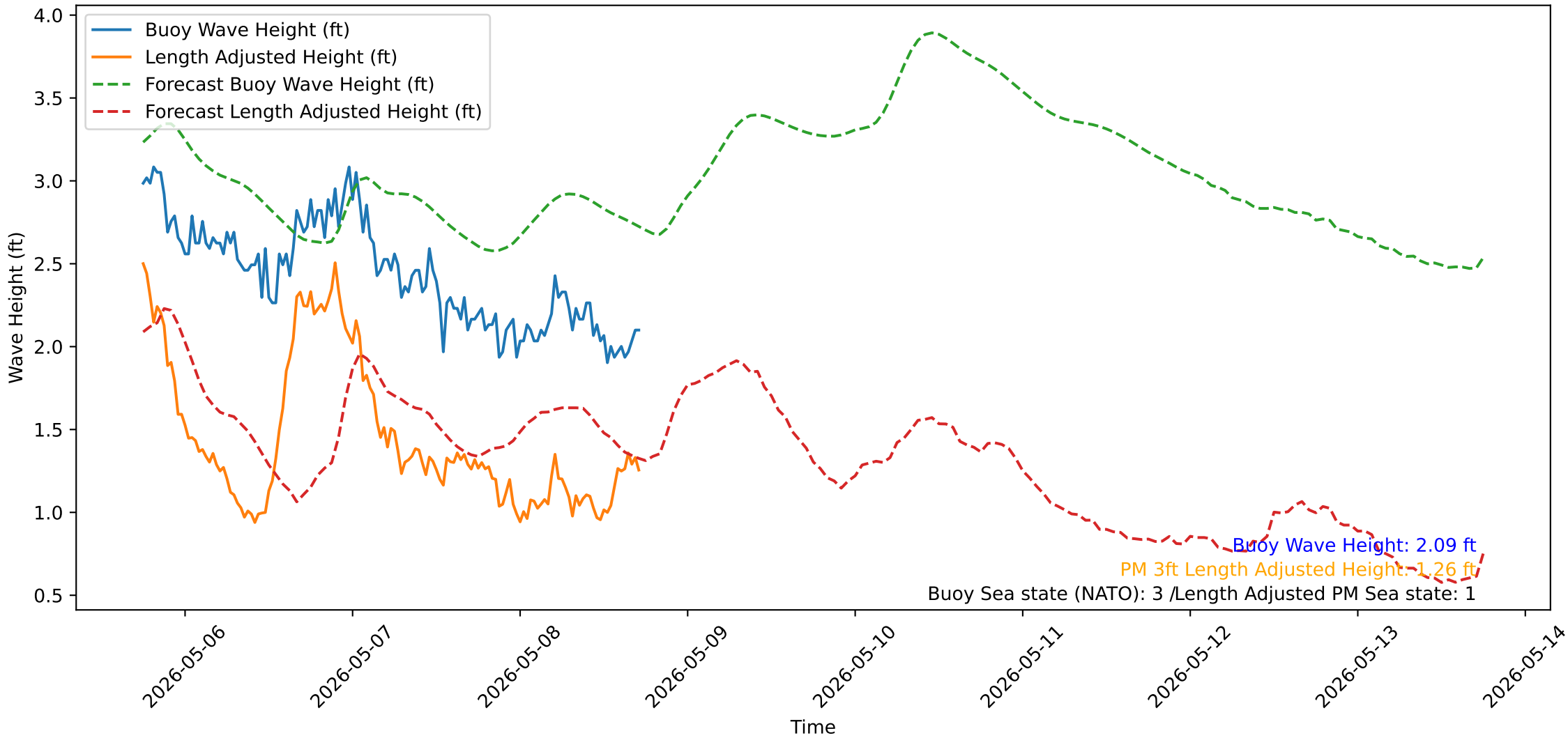
Wave Heights over Time for Red Beach at 2026-05-08 17:40:50
