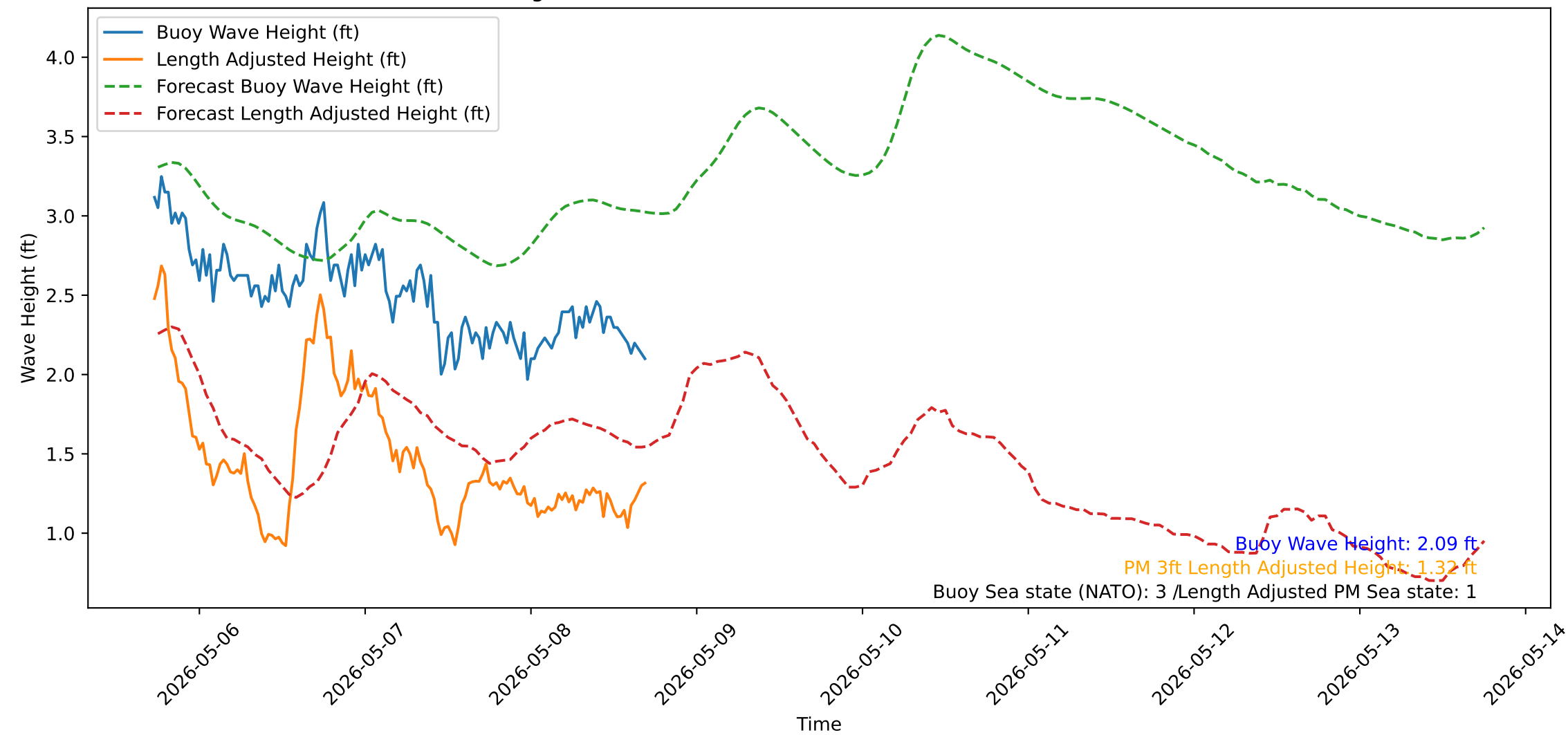
Wave Heights over Time for Oceanside Harbor at 2026-05-08 17:40:31
