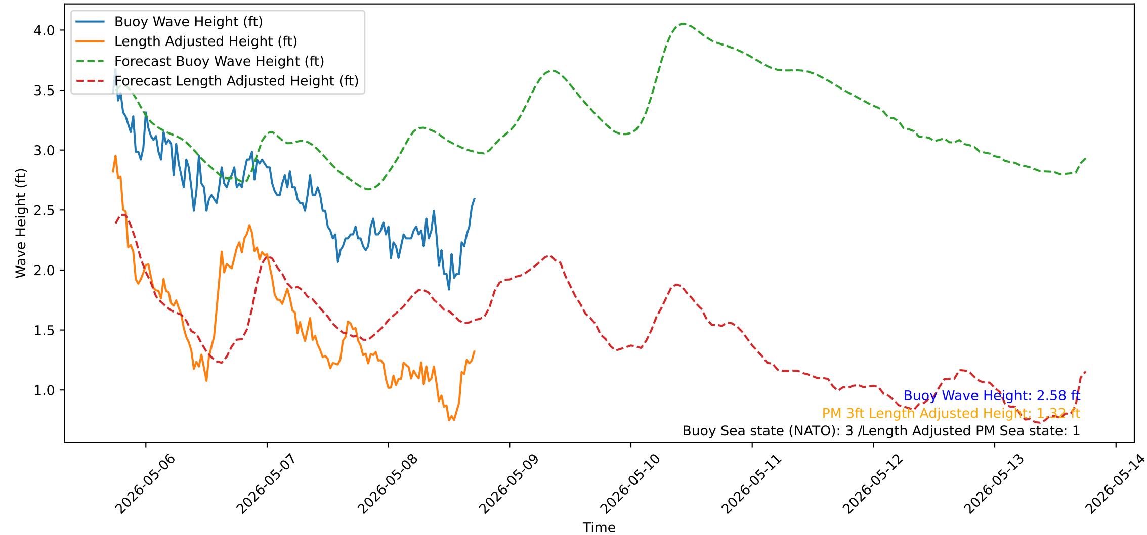
Wave Heights over Time for Green Beach at 2026-05-08 17:41:13
