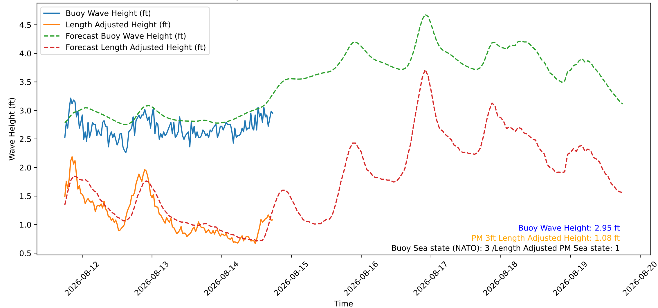
Wave Heights over Time for Green Beach at 2026-08-14 18:11:09
