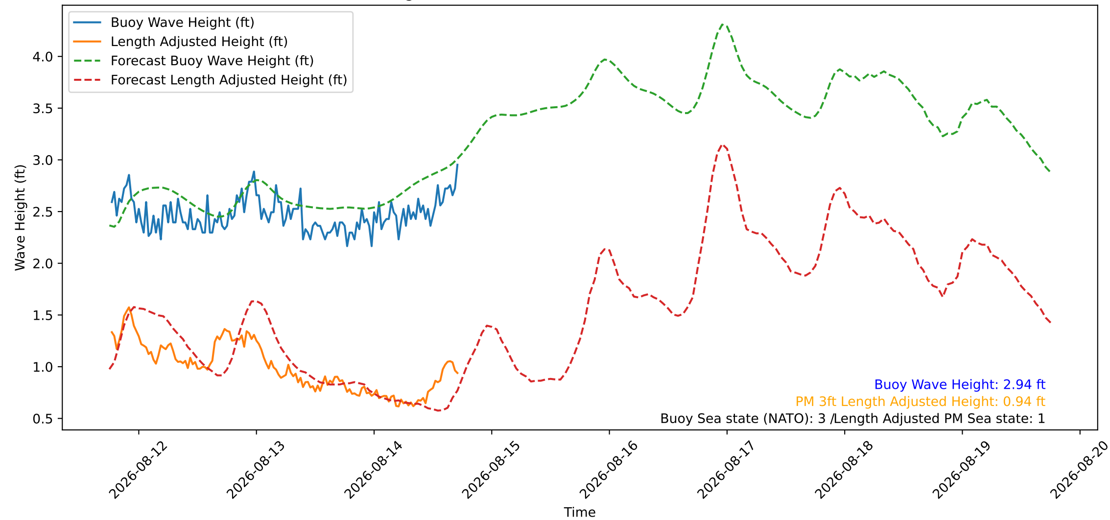
Wave Heights over Time for Red Beach at 2026-08-14 18:10:46
