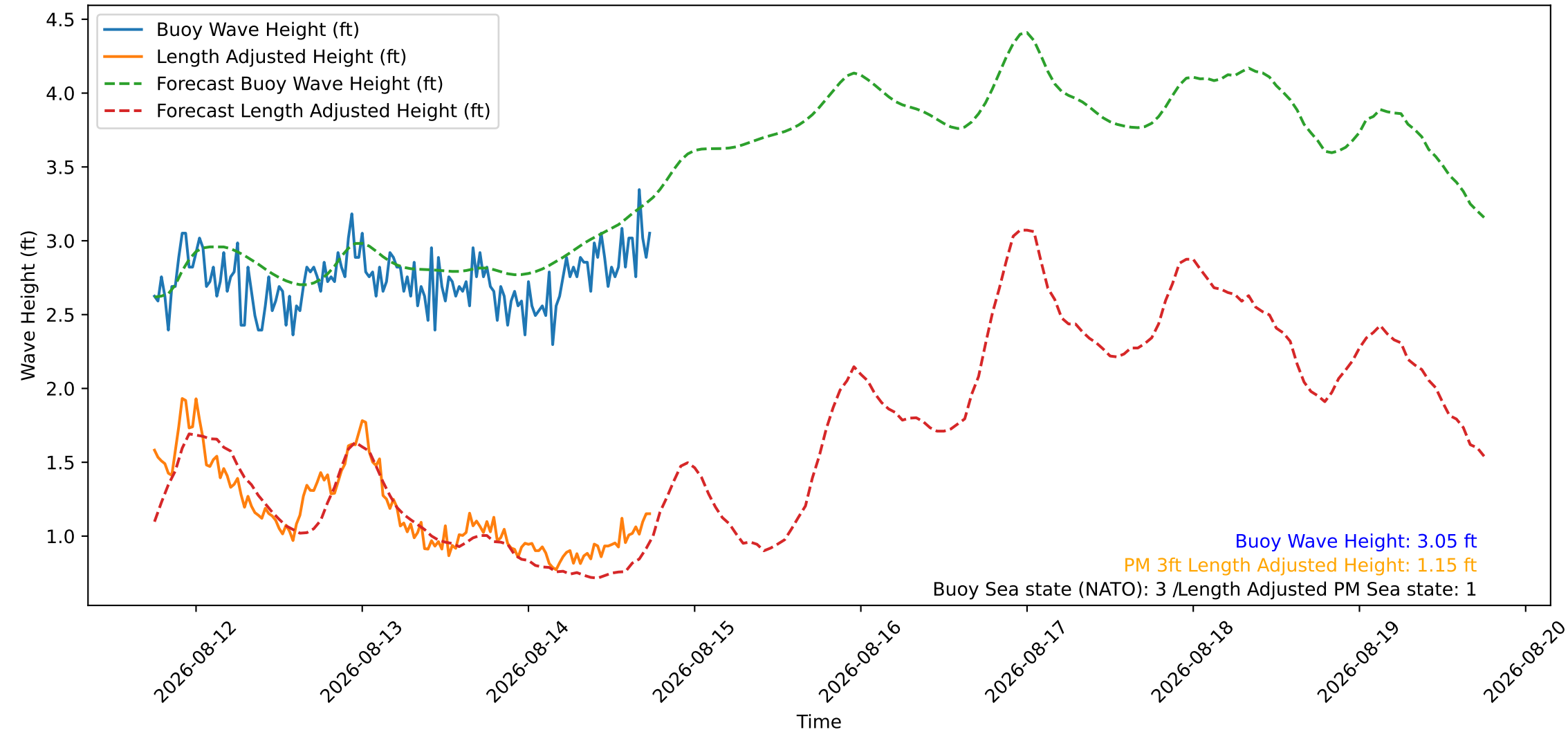
Wave Heights over Time for Oceanside Harbor at 2026-08-14 18:10:26
