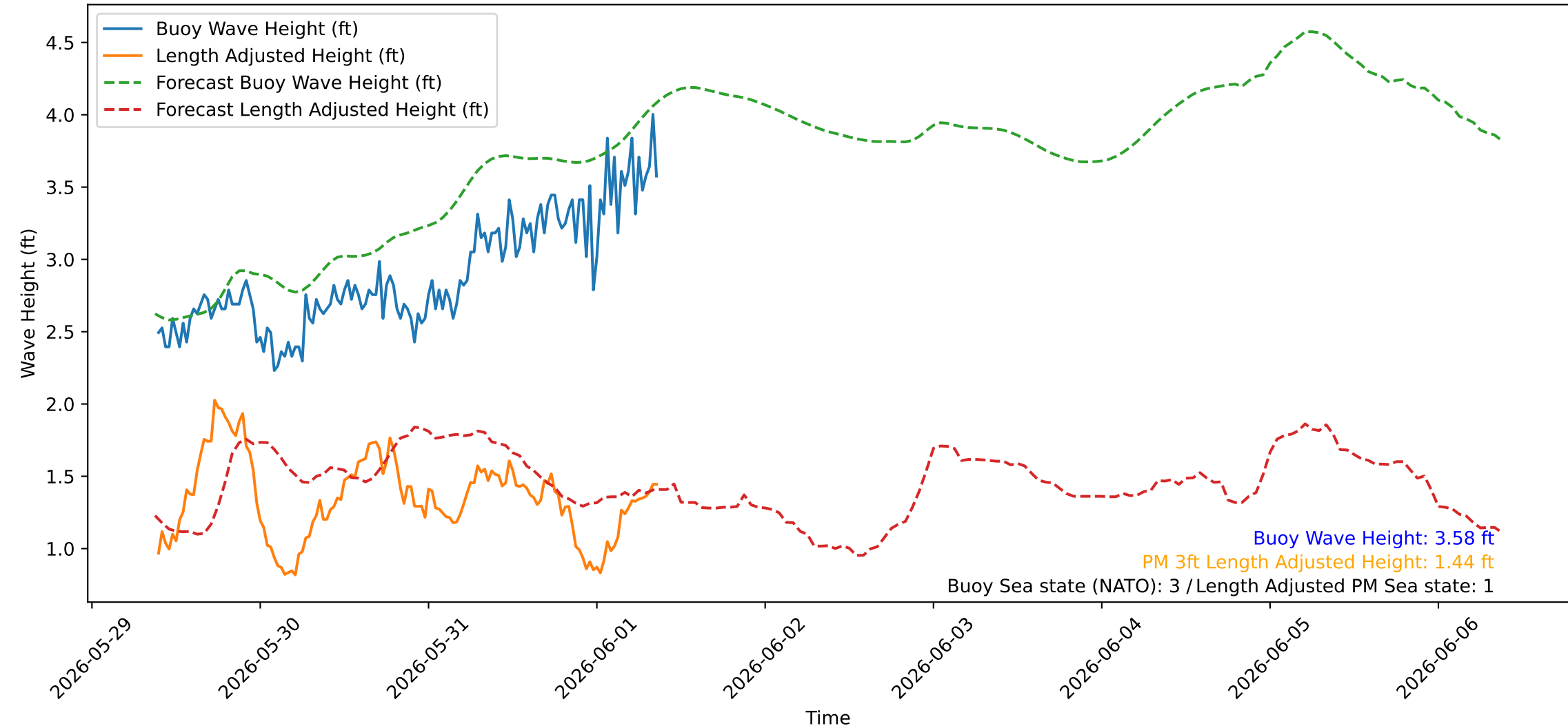
Wave Heights over Time for Red Beach at 2026-06-01 09:10:46
