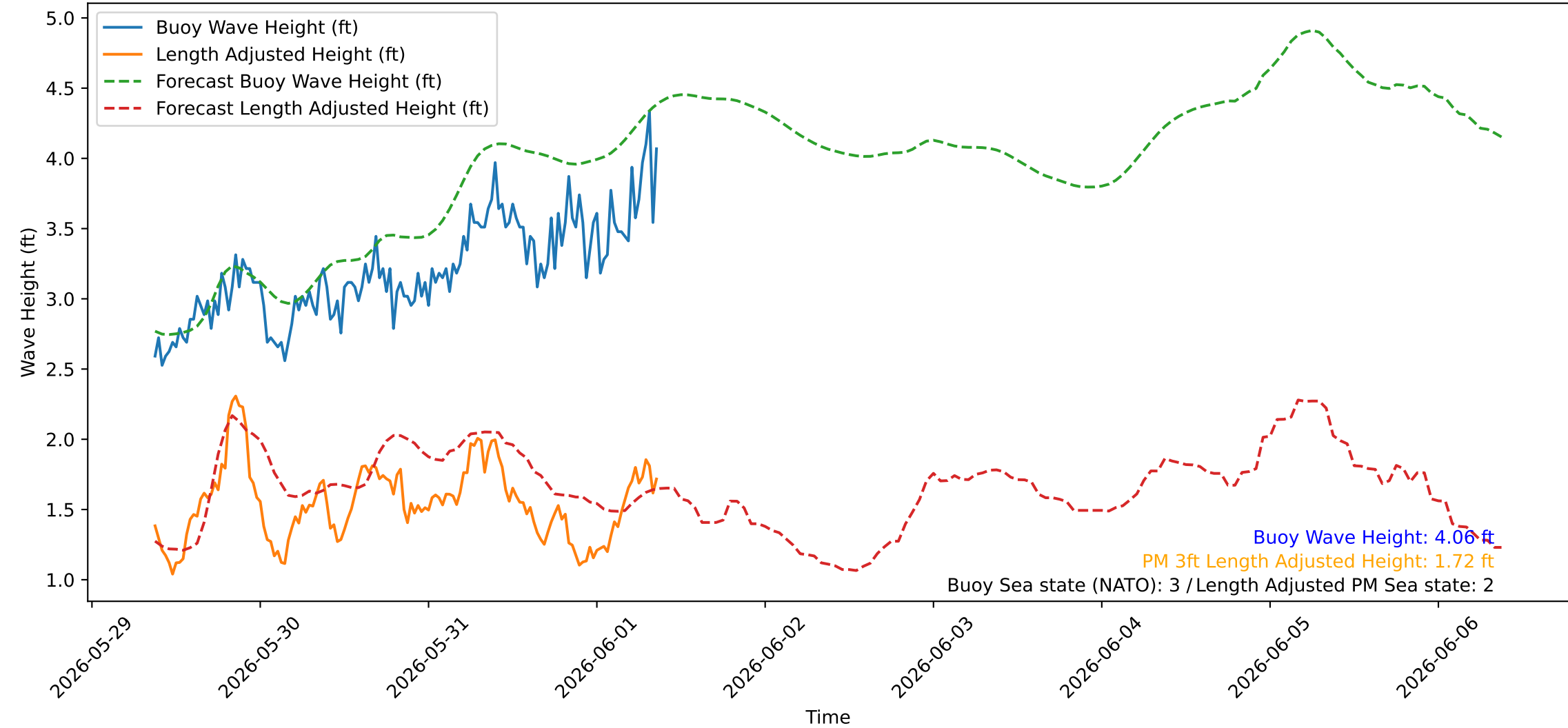
Wave Heights over Time for Green Beach at 2026-06-01 09:11:08
