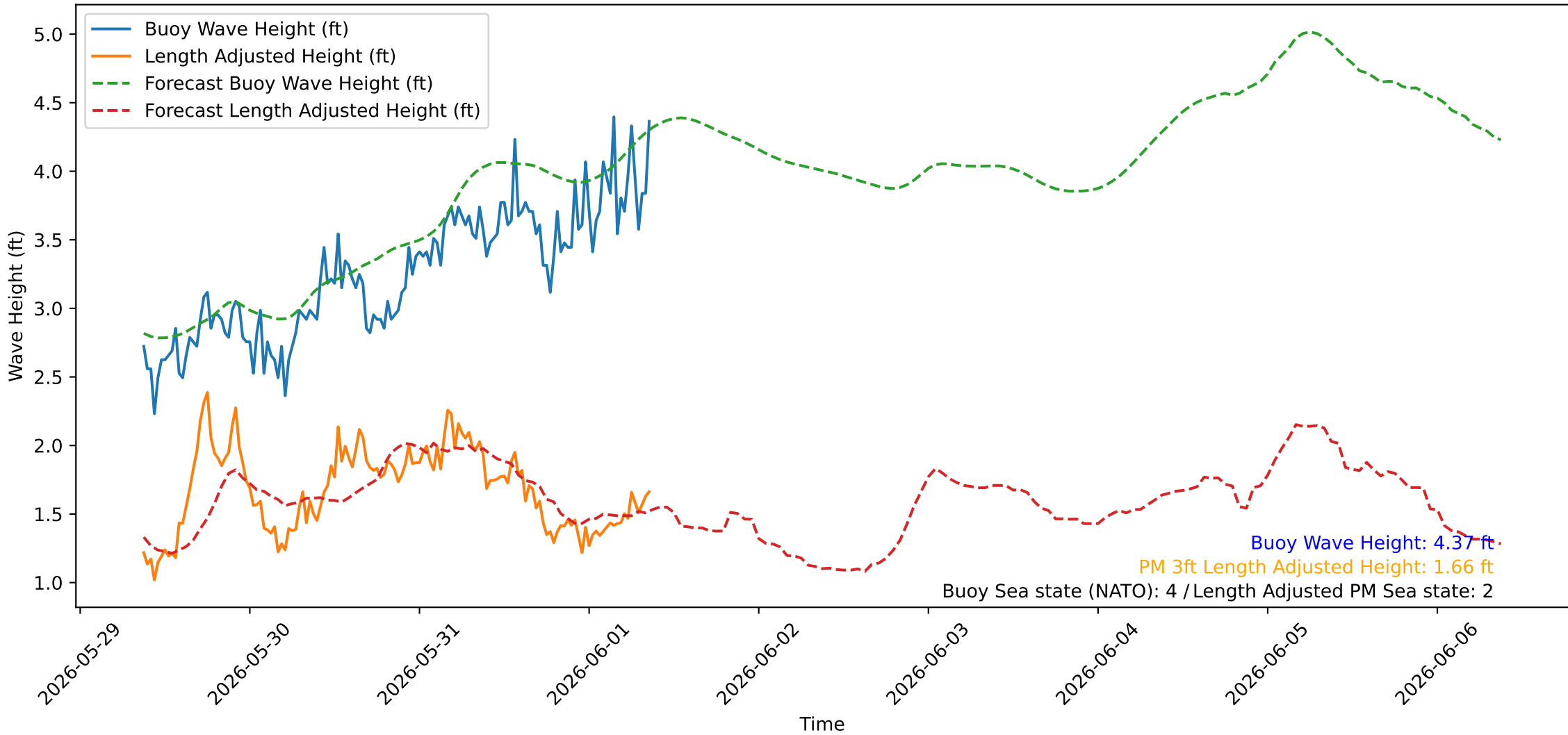
Wave Heights over Time for Oceanside Harbor at 2026-06-01 09:10:26
