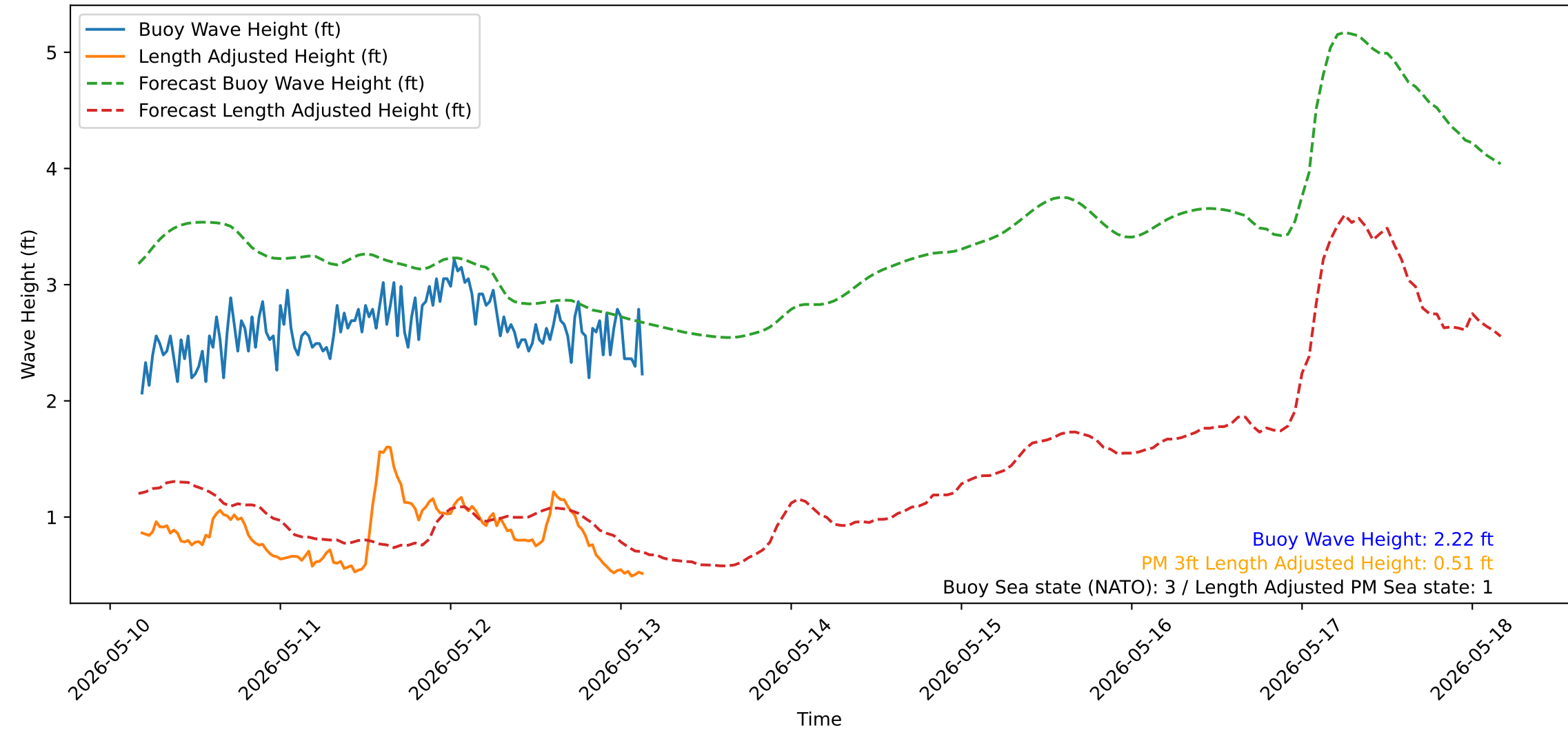
Wave Heights over Time for Red Beach at 2026-05-13 04:00:50
