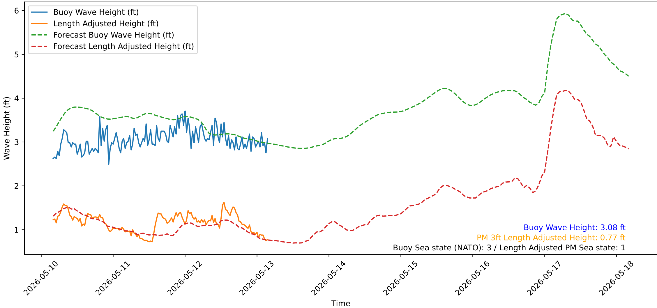
Wave Heights over Time for Oceanside Harbor at 2026-05-13 04:00:31
