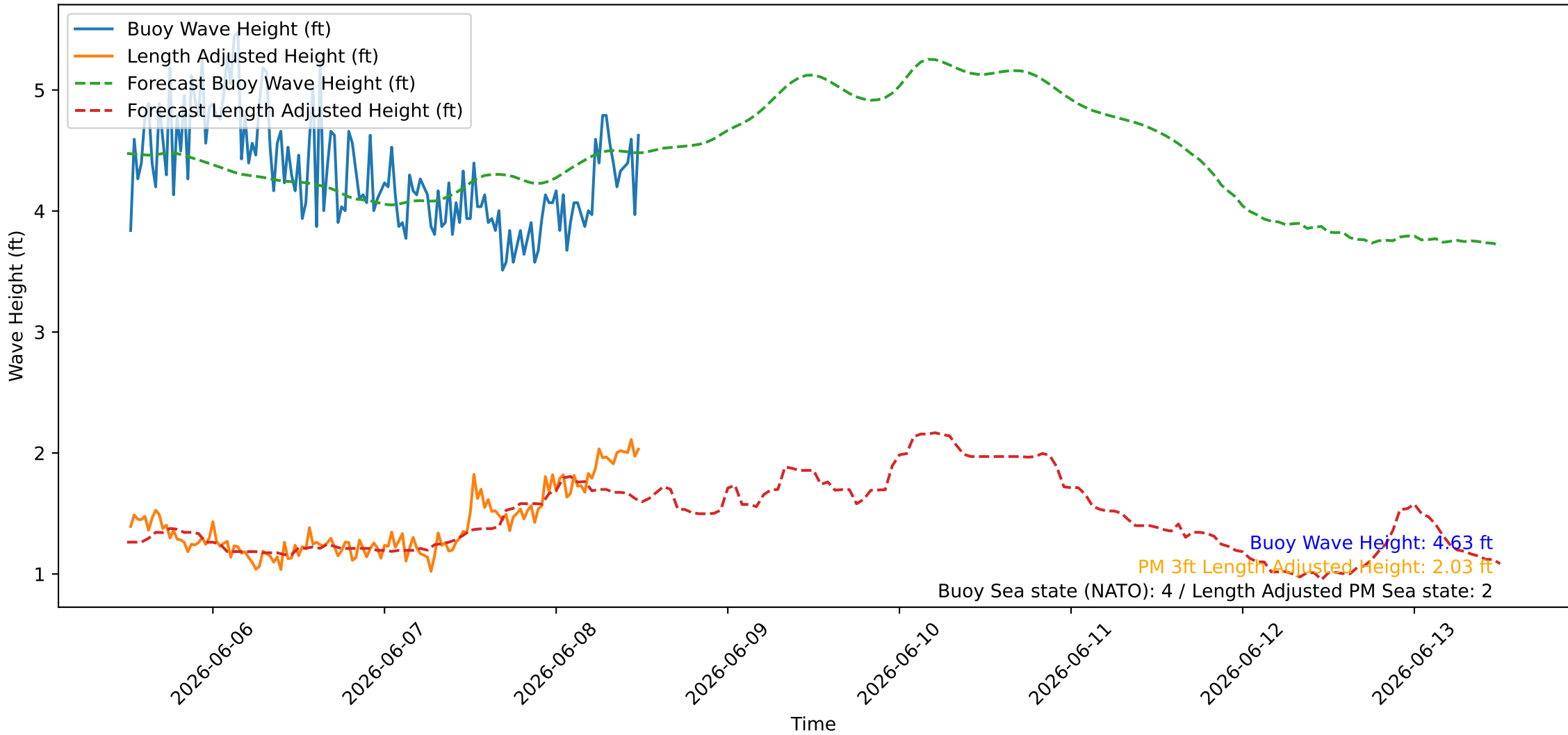
Wave Heights over Time for Oceanside Harbor at 2026-06-08 12:20:25
