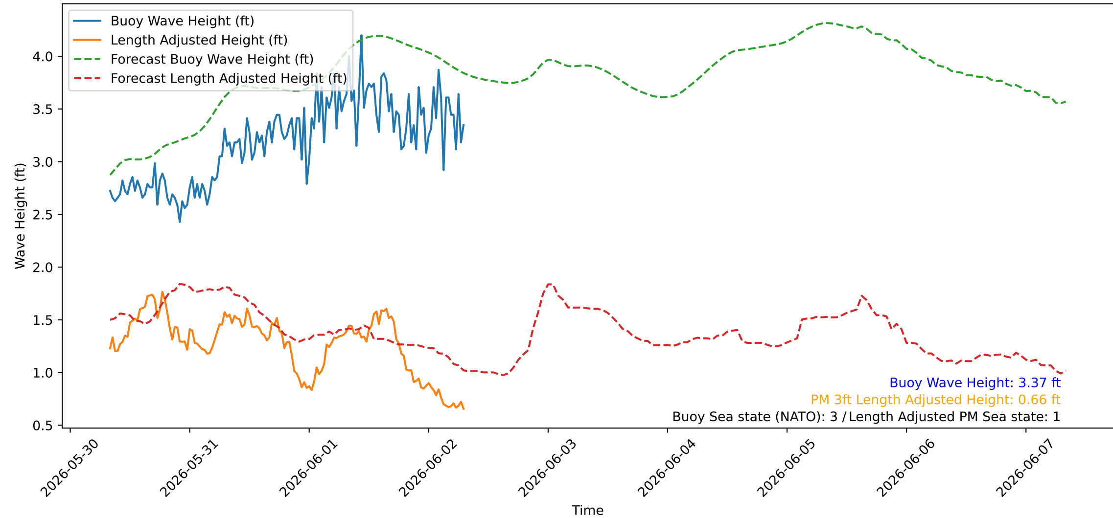
Wave Heights over Time for Red Beach at 2026-06-02 07:50:46
