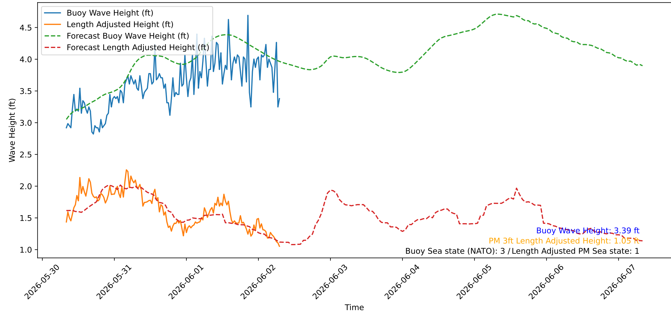
Wave Heights over Time for Oceanside Harbor at 2026-06-02 07:50:26
