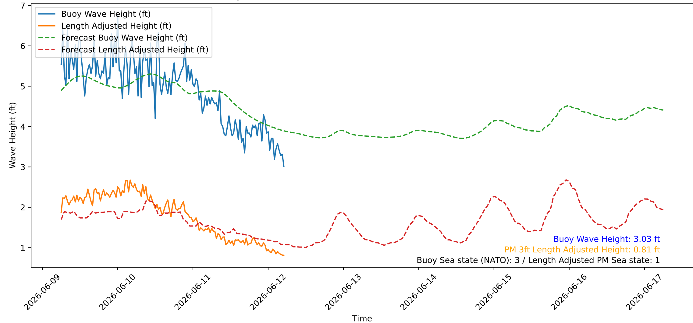
Wave Heights over Time for Oceanside Harbor at 2026-06-12 05:50:26
