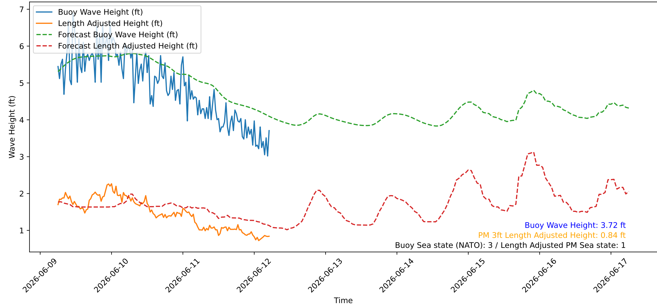
Wave Heights over Time for Green Beach at 2026-06-12 05:51:10
