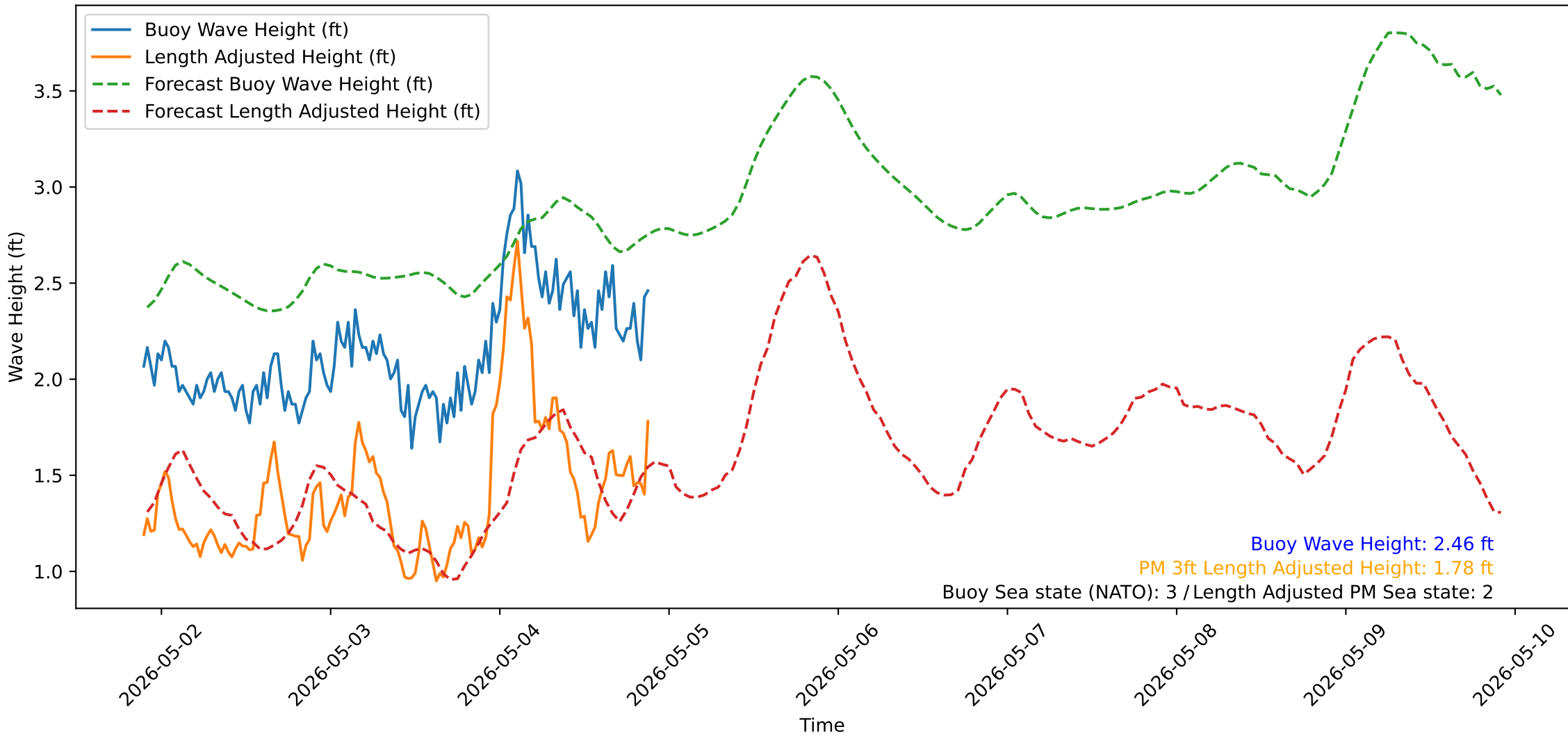
Wave Heights over Time for Oceanside Harbor at 2026-05-04 21:40:31
