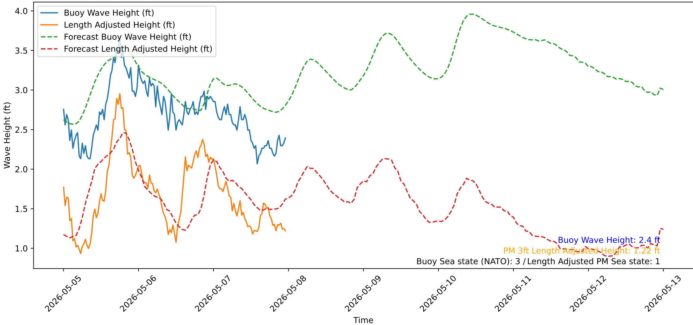
Wave Heights over Time for Green Beach at 2026-05-08 00:01:12
