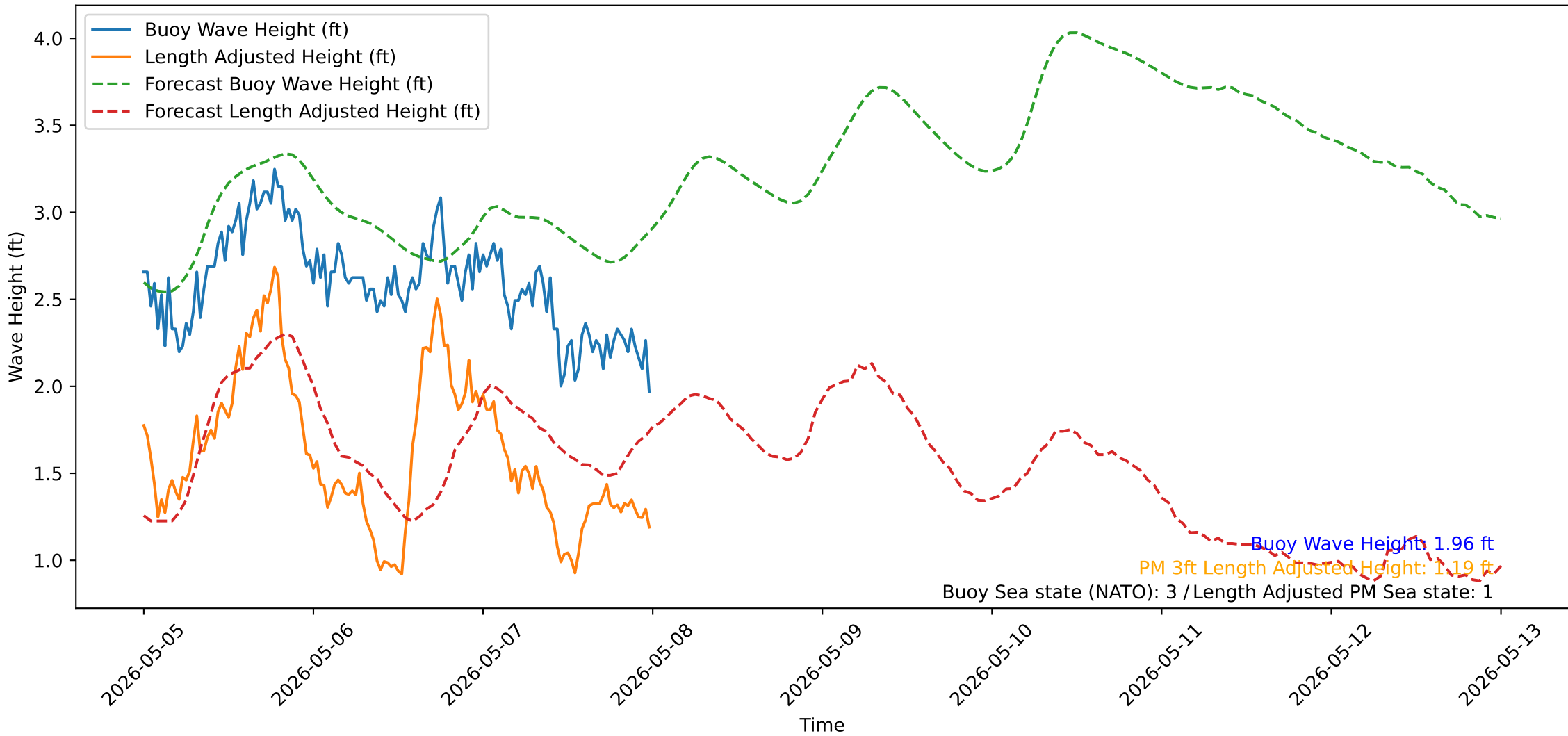
Wave Heights over Time for Oceanside Harbor at 2026-05-08 00:00:31
