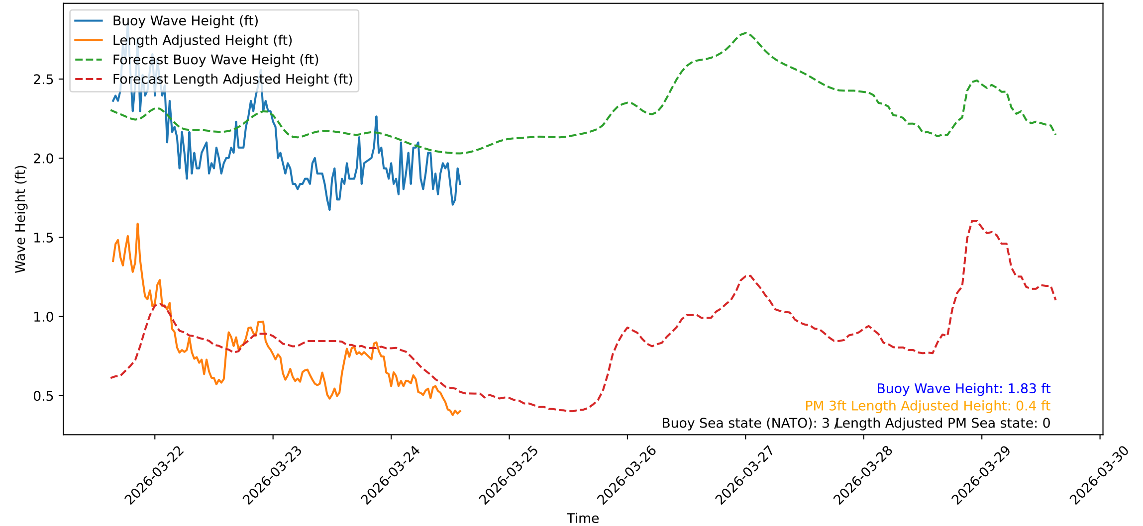
Wave Heights over Time for Red Beach at 2026-03-24 15:10:47
