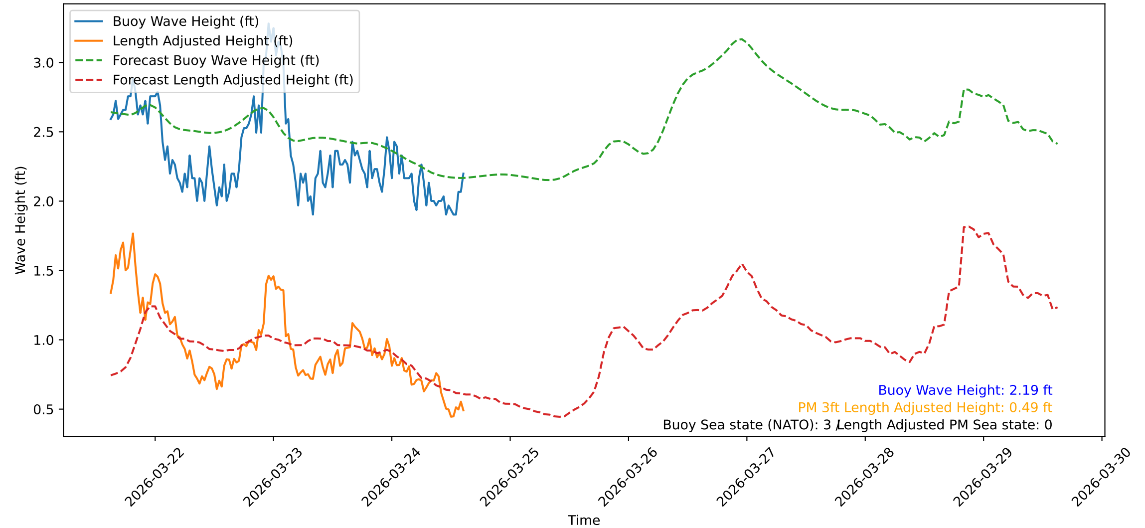
Wave Heights over Time for Green Beach at 2026-03-24 15:11:09
