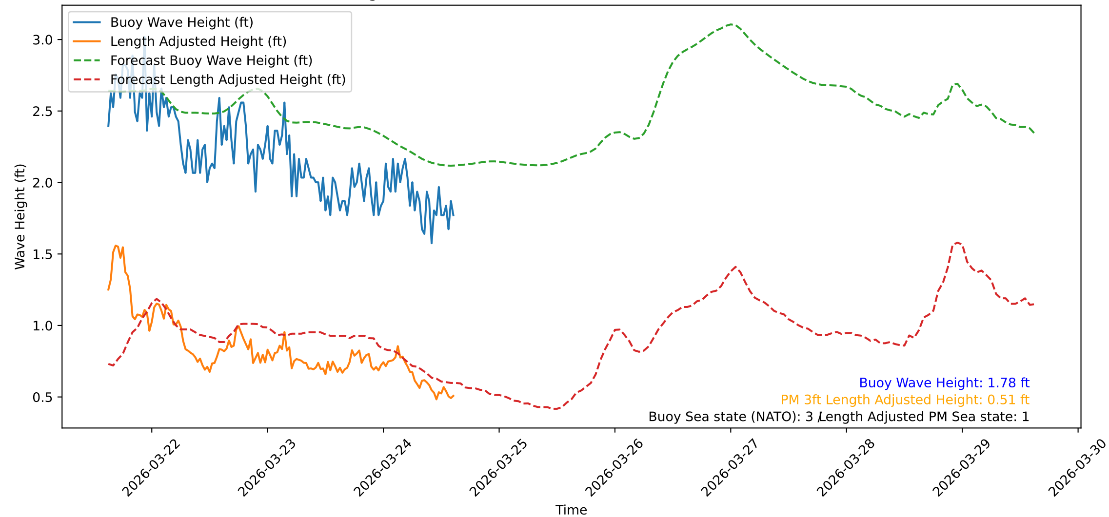
Wave Heights over Time for Oceanside Harbor at 2026-03-24 15:10:31
