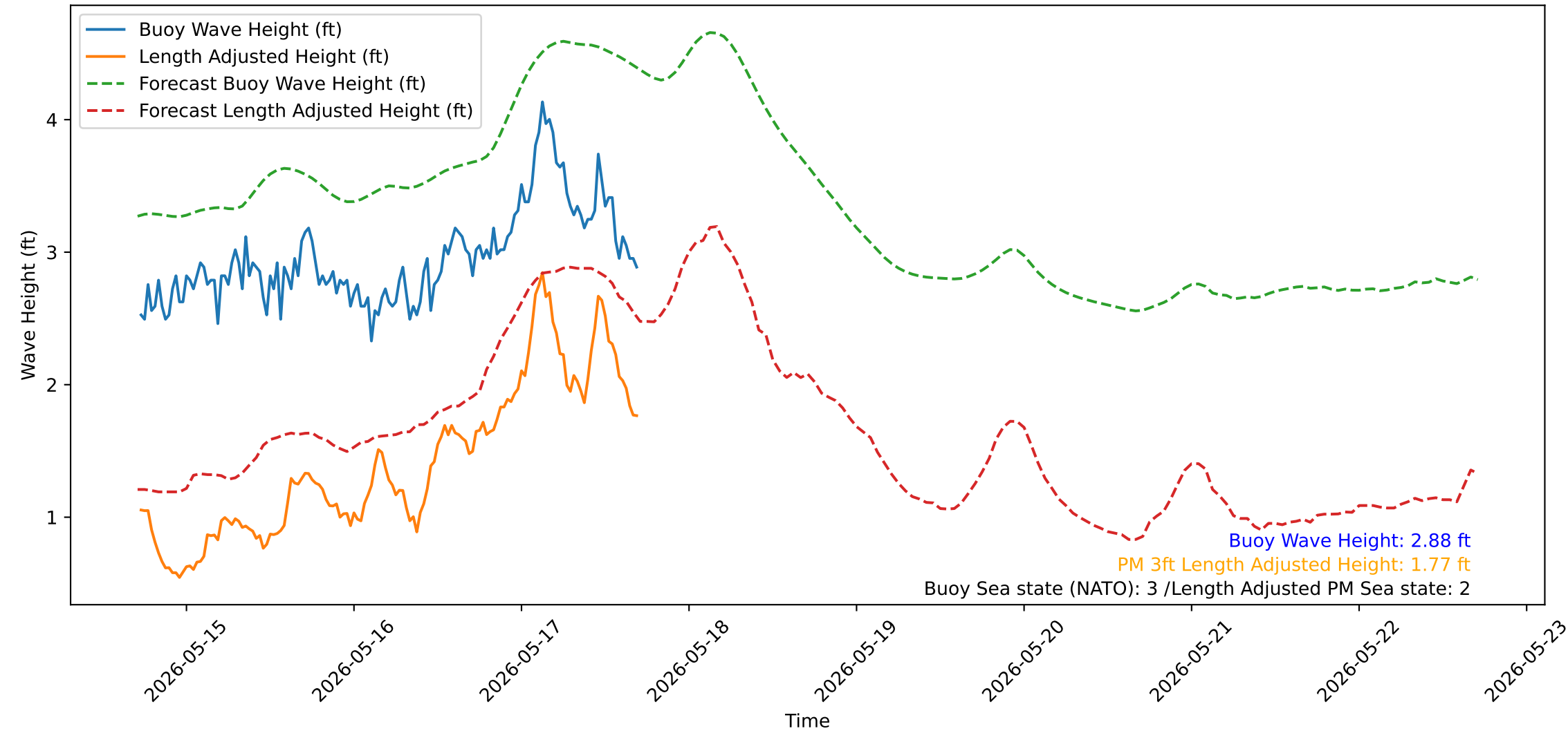
Wave Heights over Time for Red Beach at 2026-05-17 17:10:50
