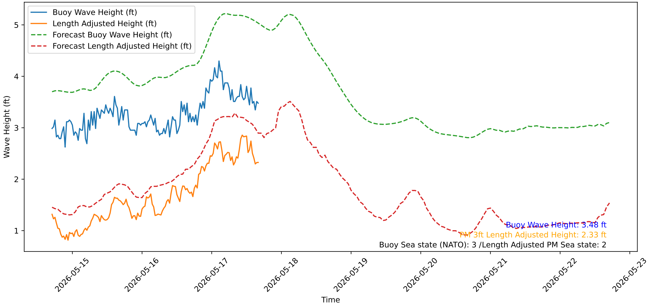
Wave Heights over Time for Oceanside Harbor at 2026-05-17 17:10:31
