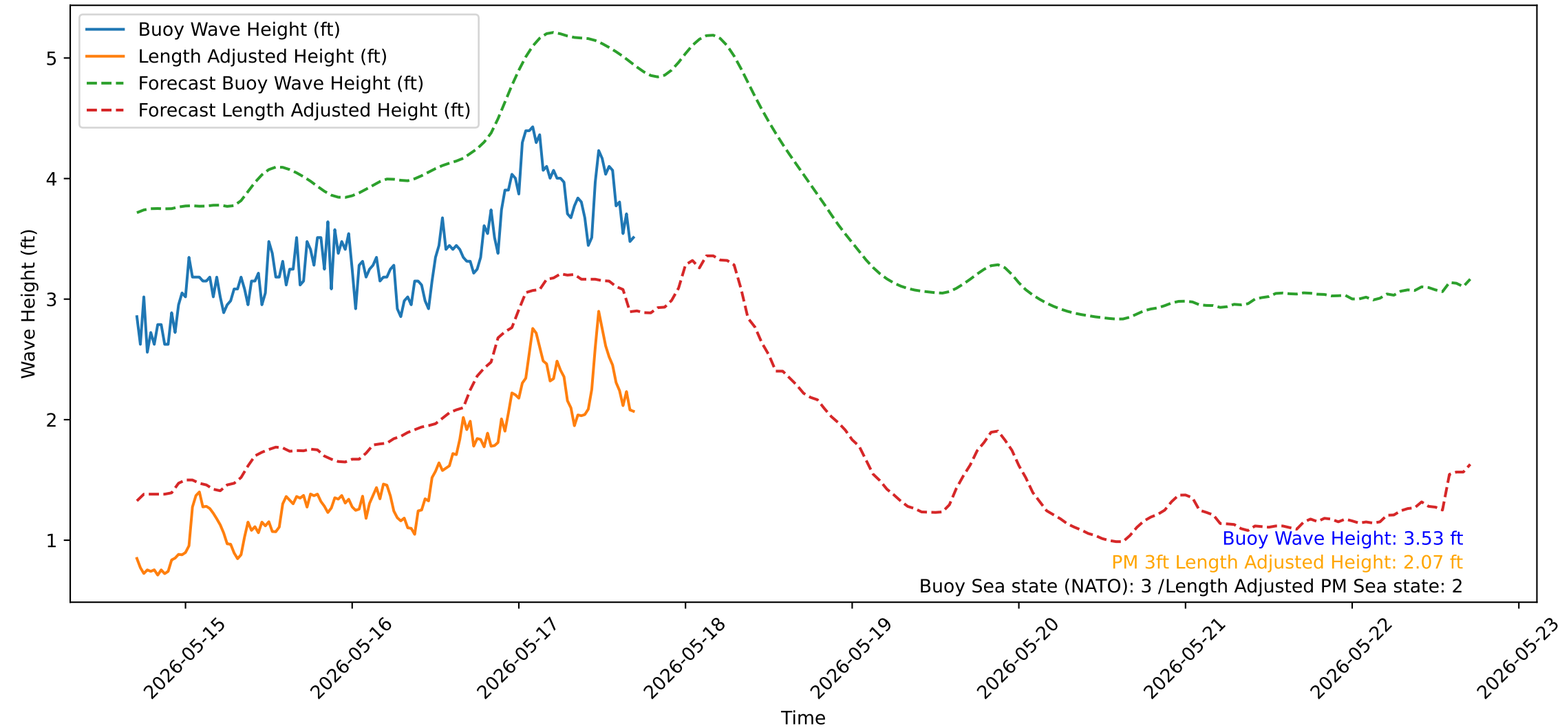
Wave Heights over Time for Green Beach at 2026-05-17 17:11:13
