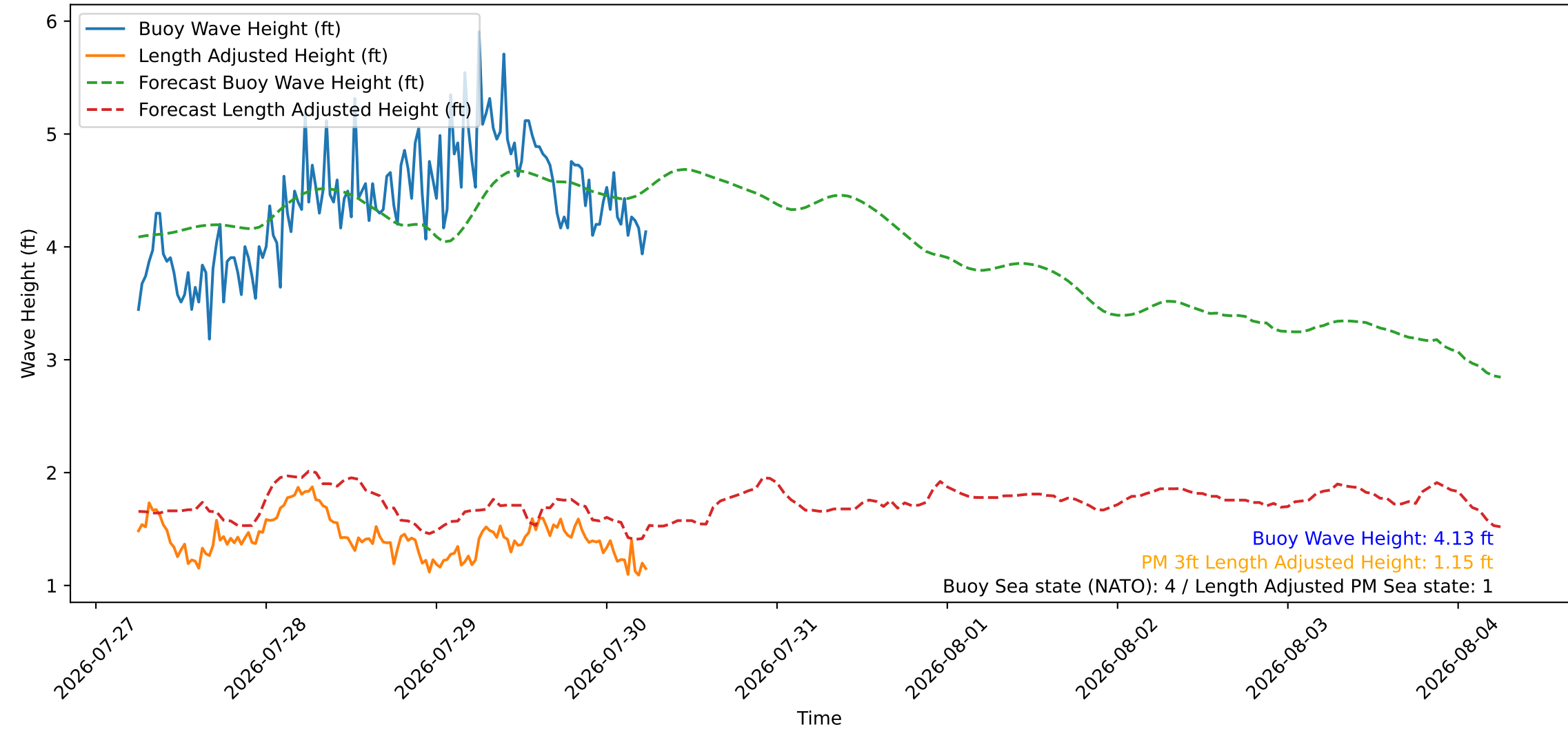
Wave Heights over Time for Oceanside Harbor at 2026-07-30 06:10:26
