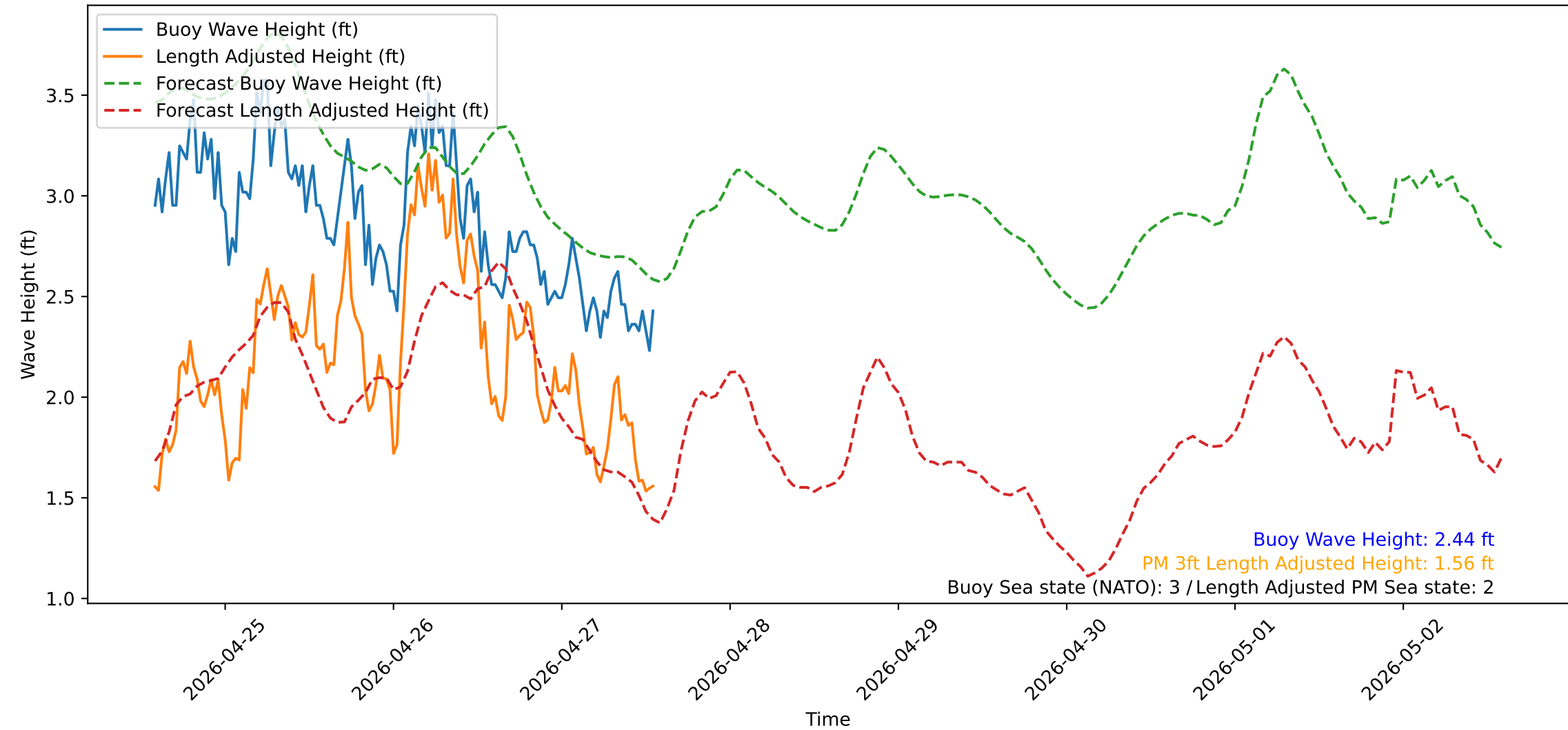
Wave Heights over Time for Green Beach at 2026-04-27 13:51:14
