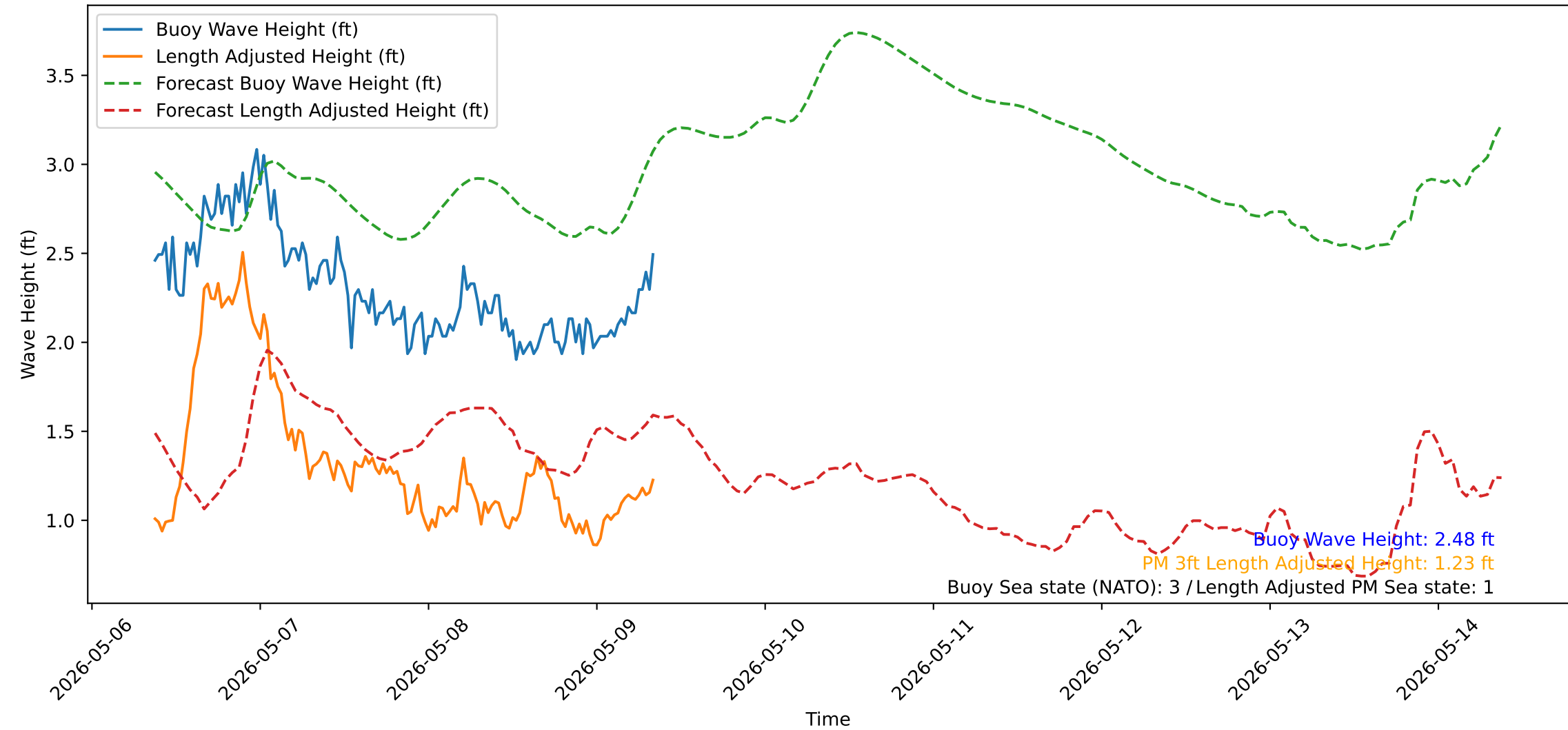
Wave Heights over Time for Red Beach at 2026-05-09 08:40:50
