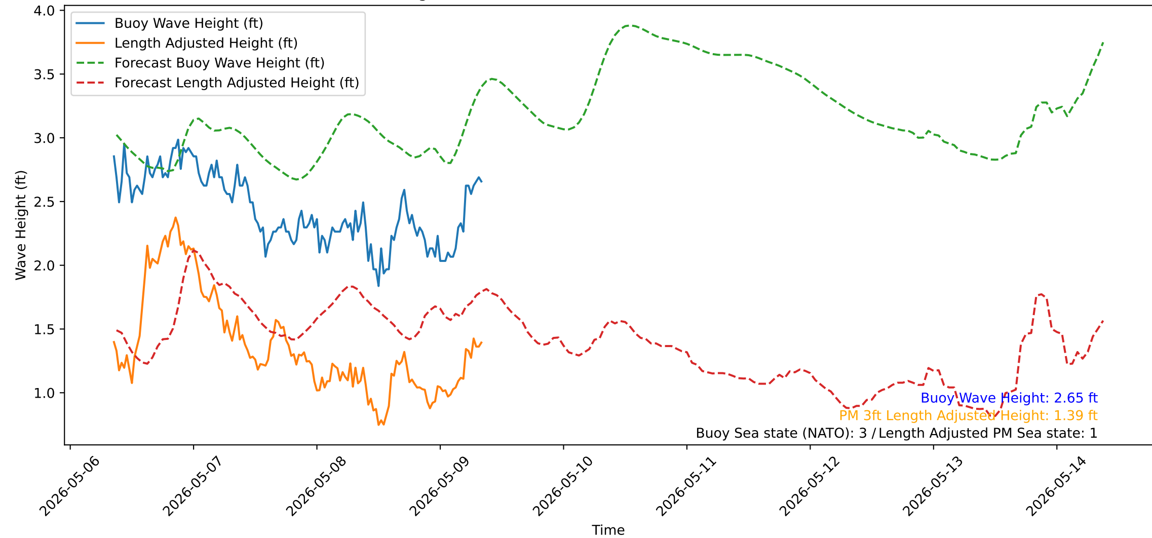
Wave Heights over Time for Green Beach at 2026-05-09 08:41:13
