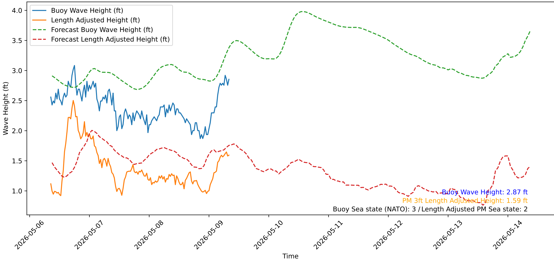
Wave Heights over Time for Oceanside Harbor at 2026-05-09 08:40:31
