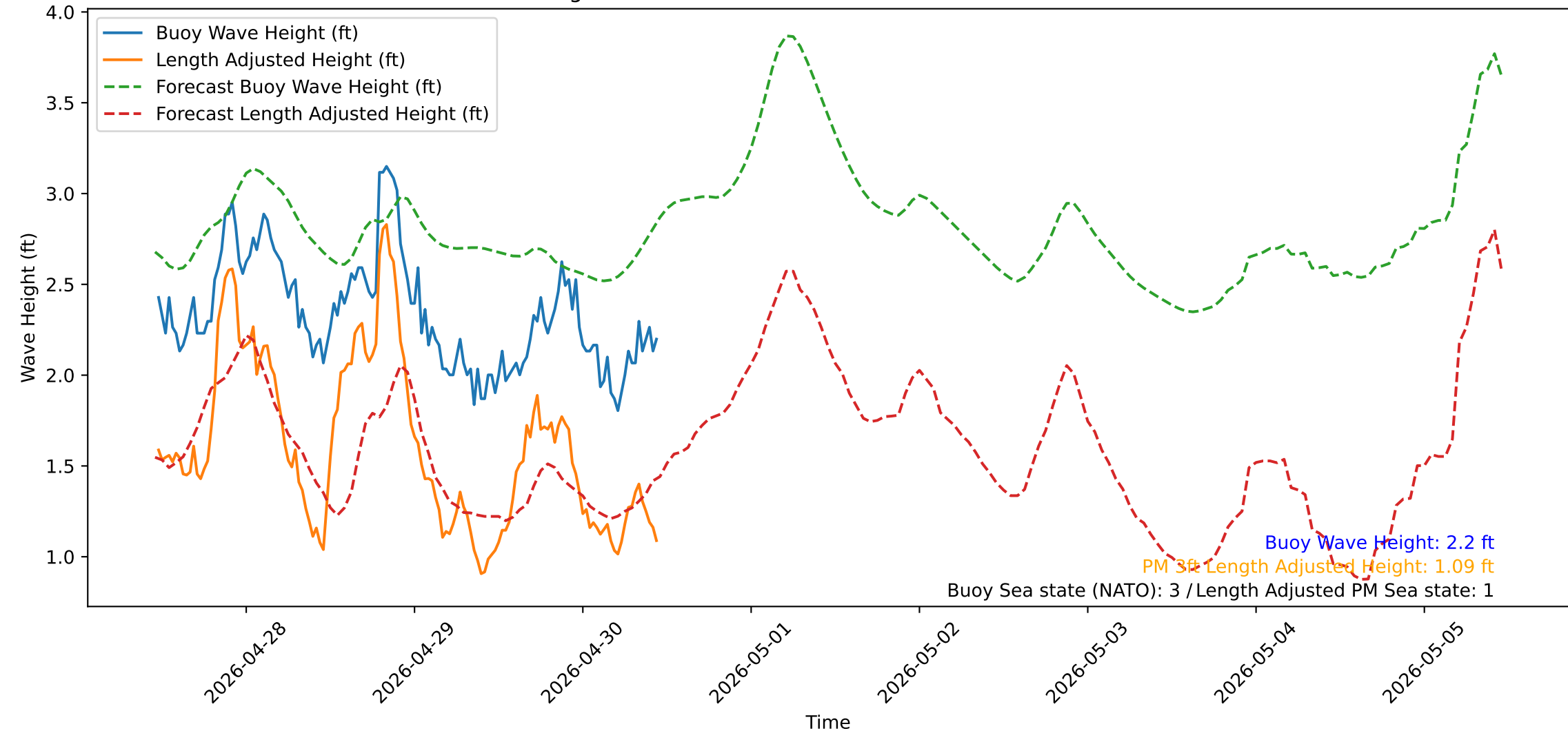
Wave Heights over Time for Green Beach at 2026-04-30 11:21:14
