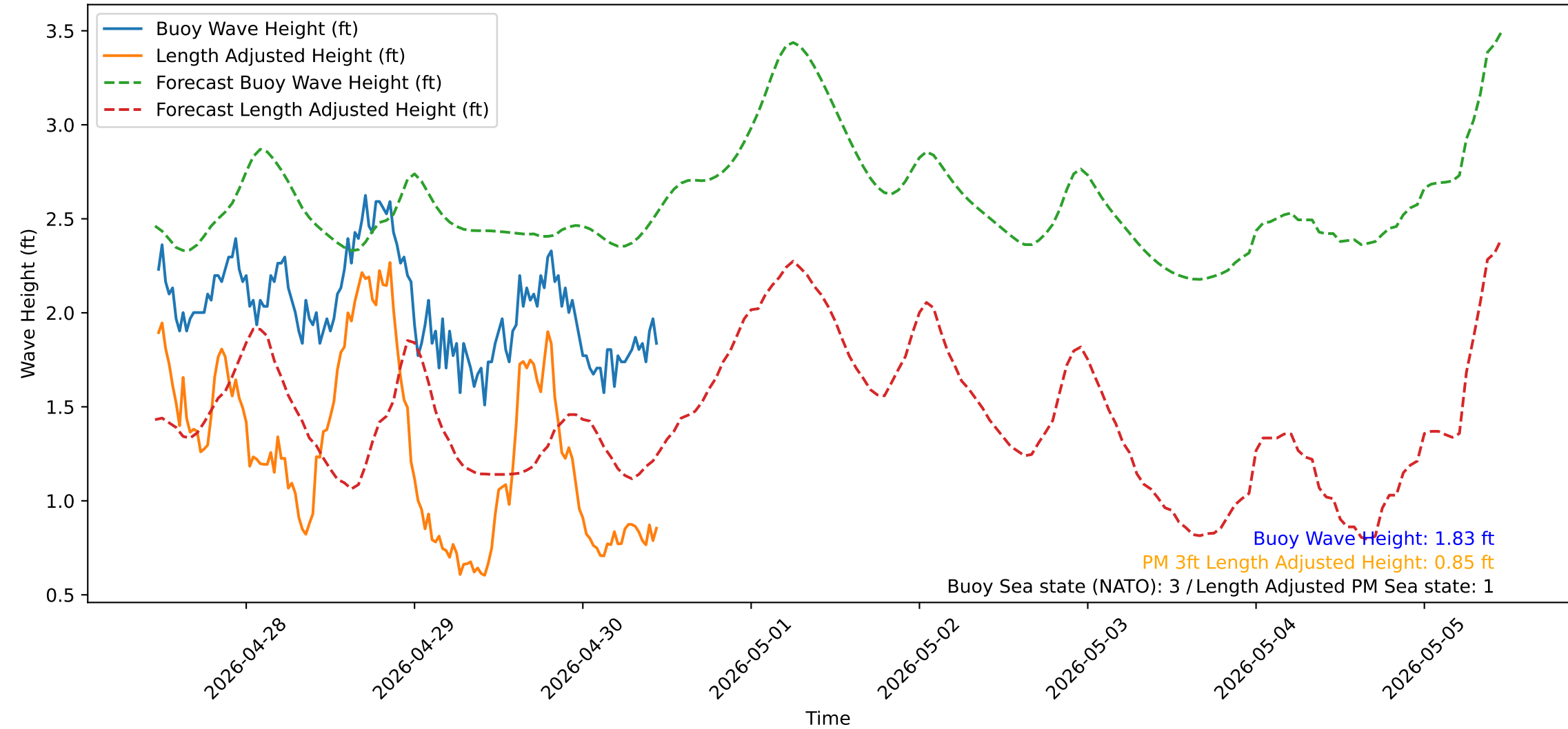
Wave Heights over Time for Red Beach at 2026-04-30 11:20:52
