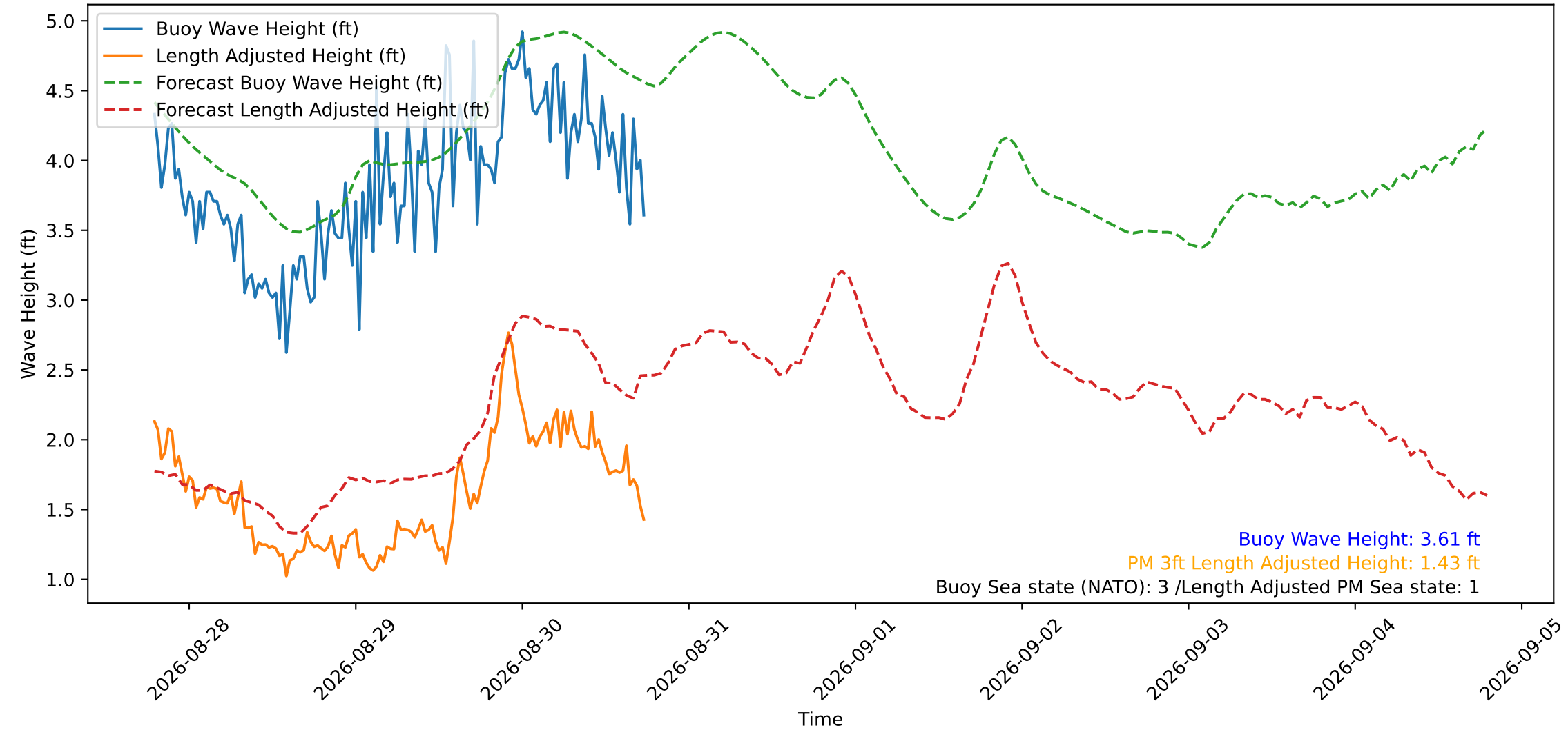
Wave Heights over Time for Green Beach at 2026-08-30 18:31:12
