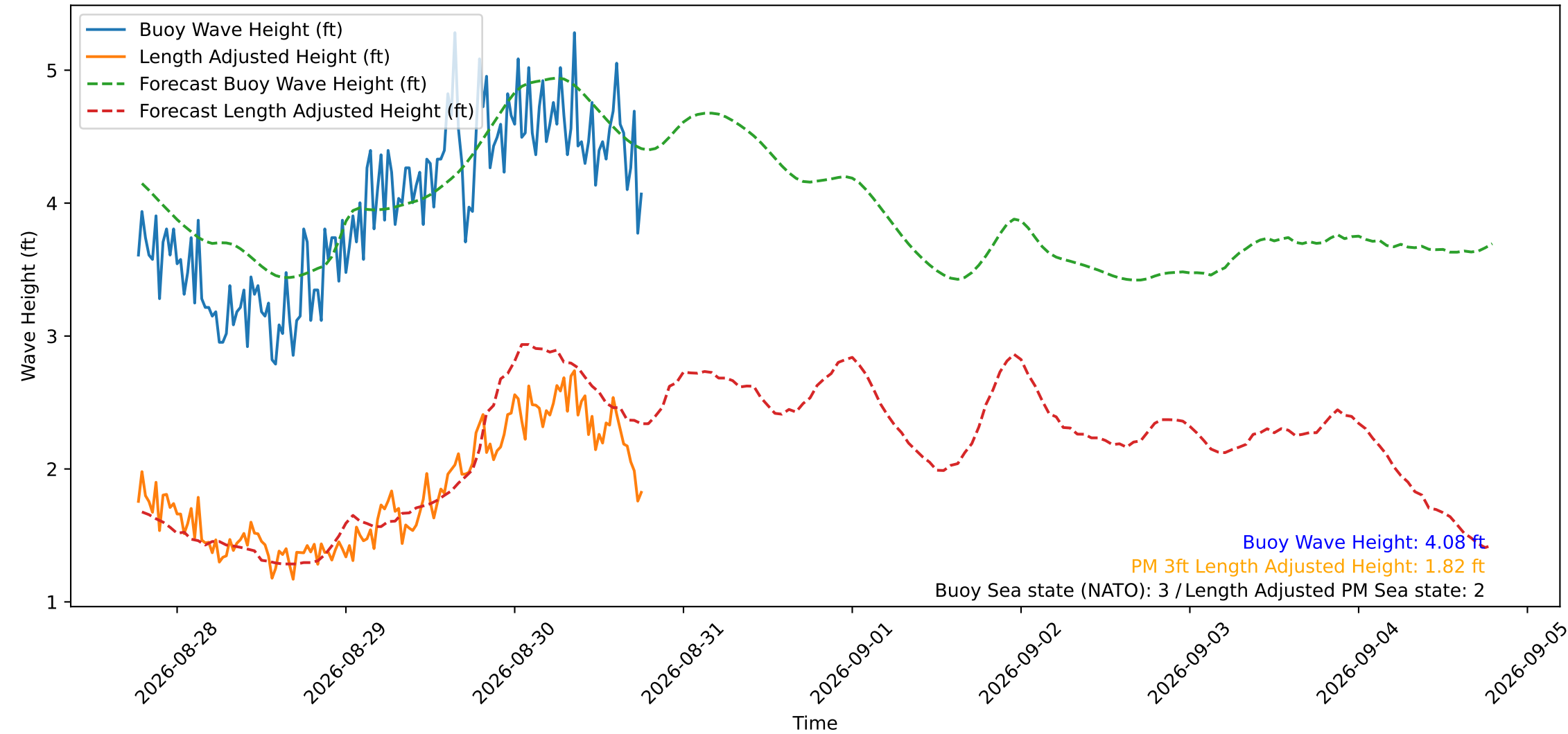
Wave Heights over Time for Oceanside Harbor at 2026-08-30 18:30:29
