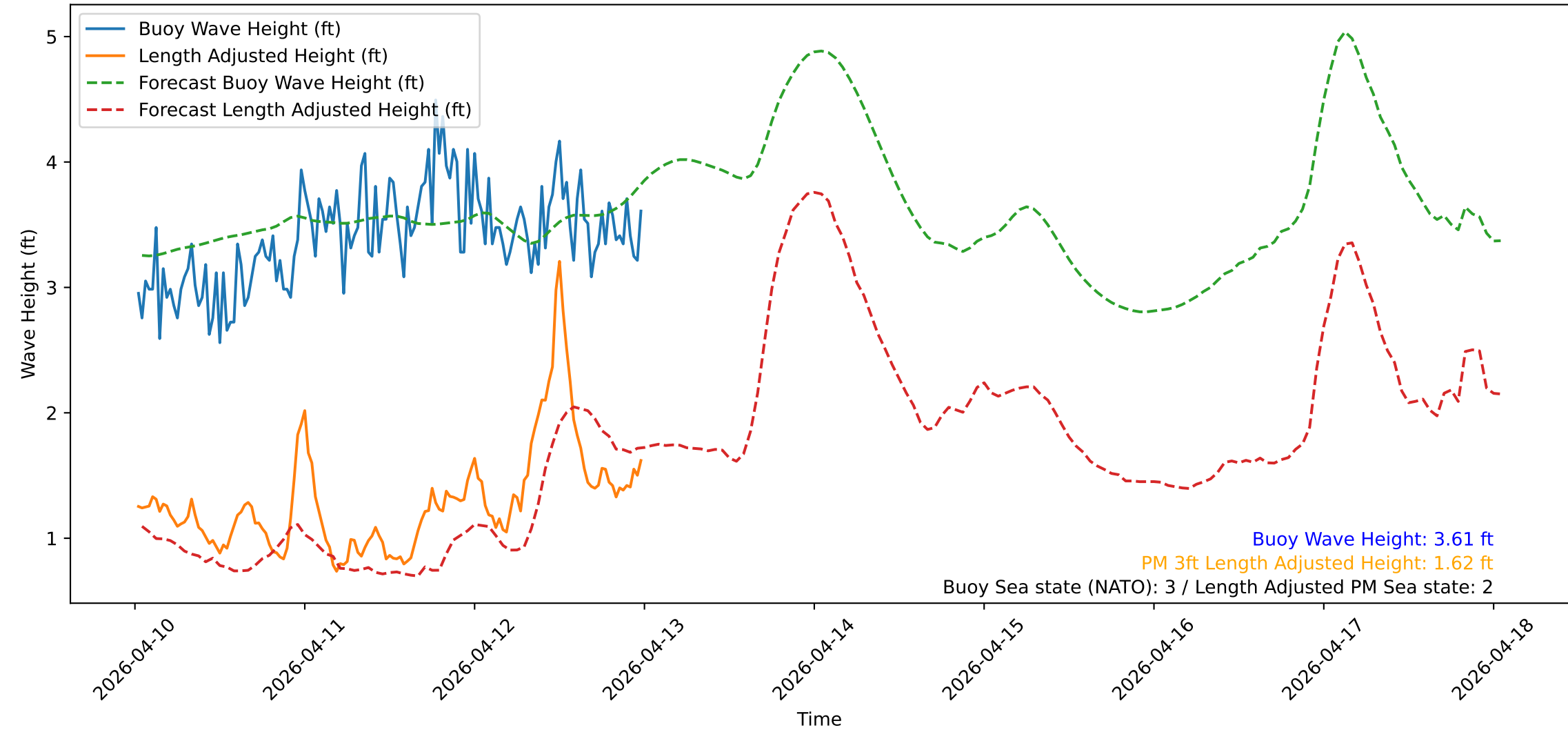
Wave Heights over Time for Green Beach at 2026-04-13 00:31:12
