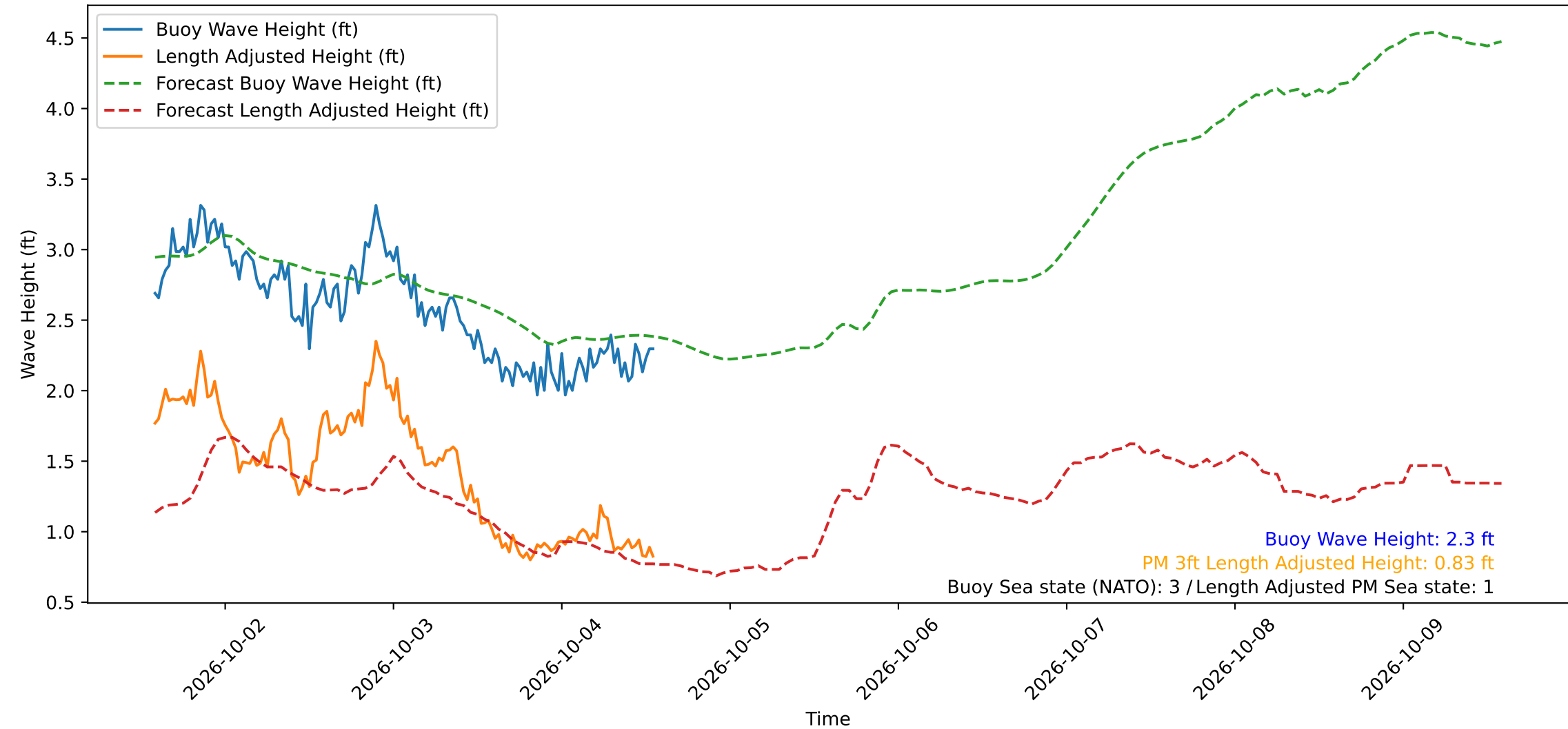
Wave Heights over Time for Oceanside Harbor at 2026-10-04 13:50:29
