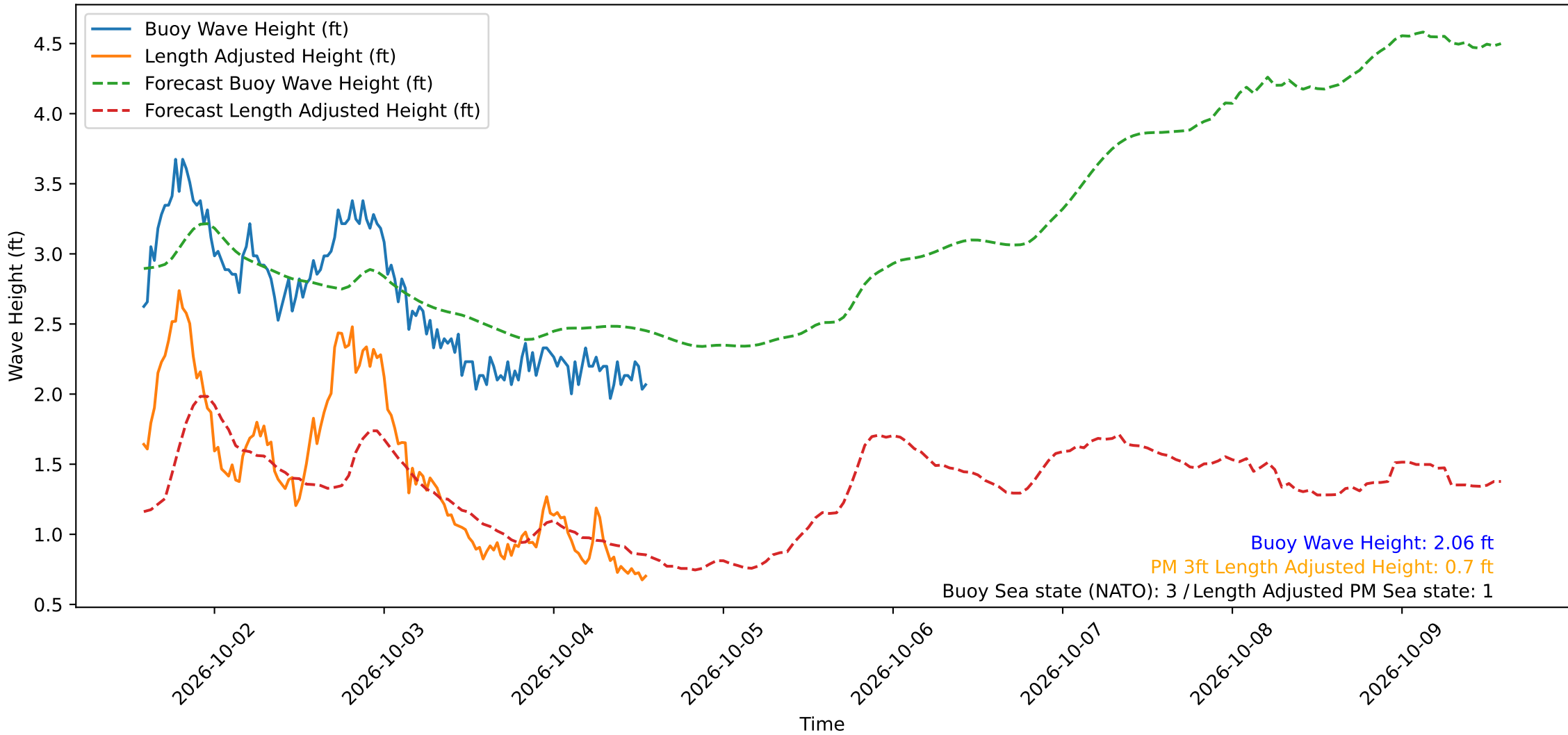
Wave Heights over Time for Green Beach at 2026-10-04 13:51:14
