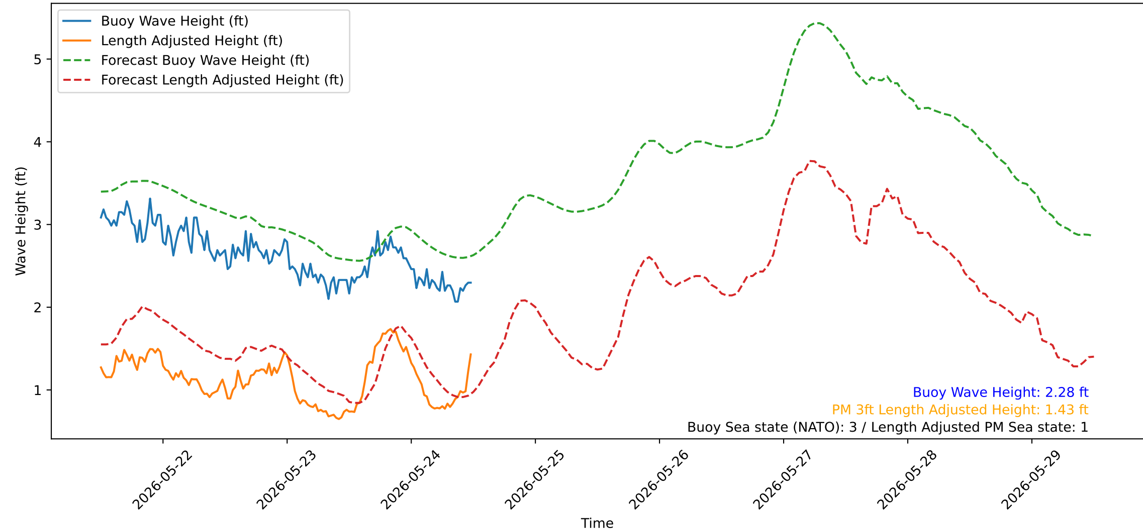
Wave Heights over Time for Green Beach at 2026-05-24 12:11:14
