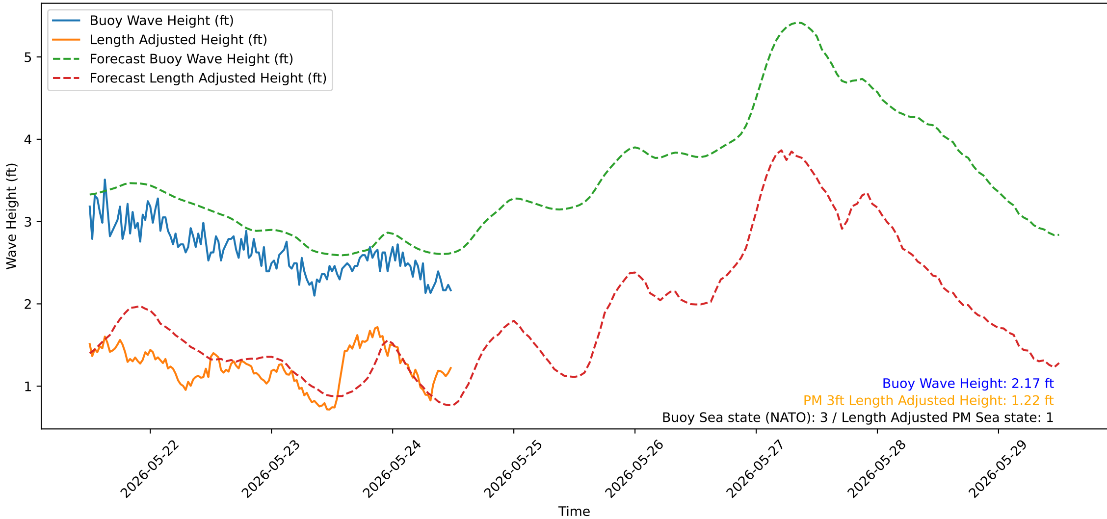
Wave Heights over Time for Oceanside Harbor at 2026-05-24 12:10:31
