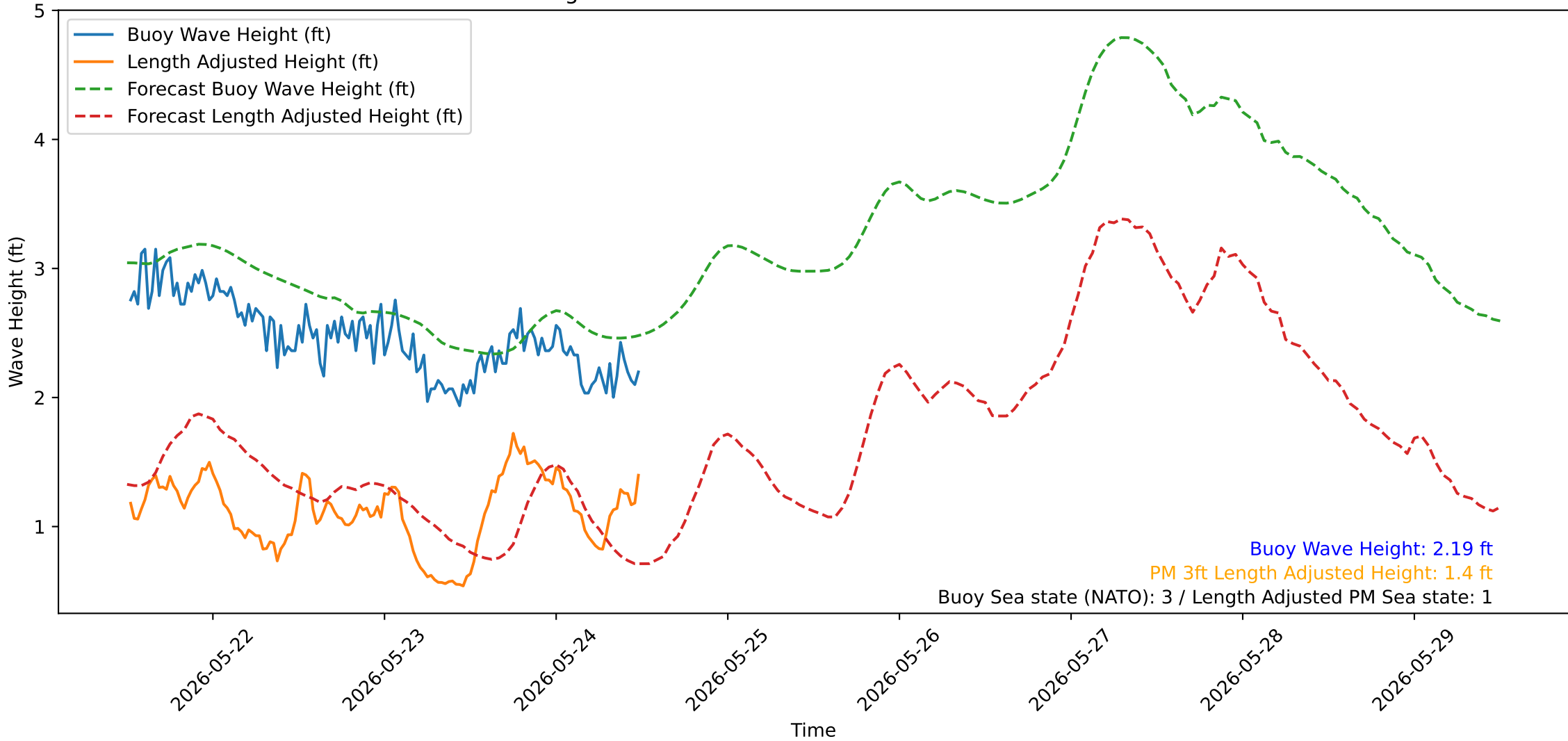
Wave Heights over Time for Red Beach at 2026-05-24 12:10:51
