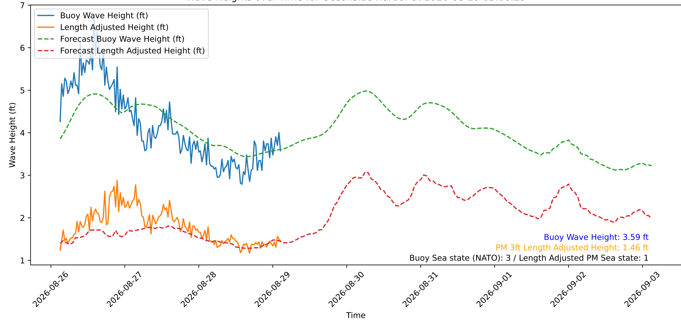
Wave Heights over Time for Oceanside Harbor at 2026-08-29 03:00:29
