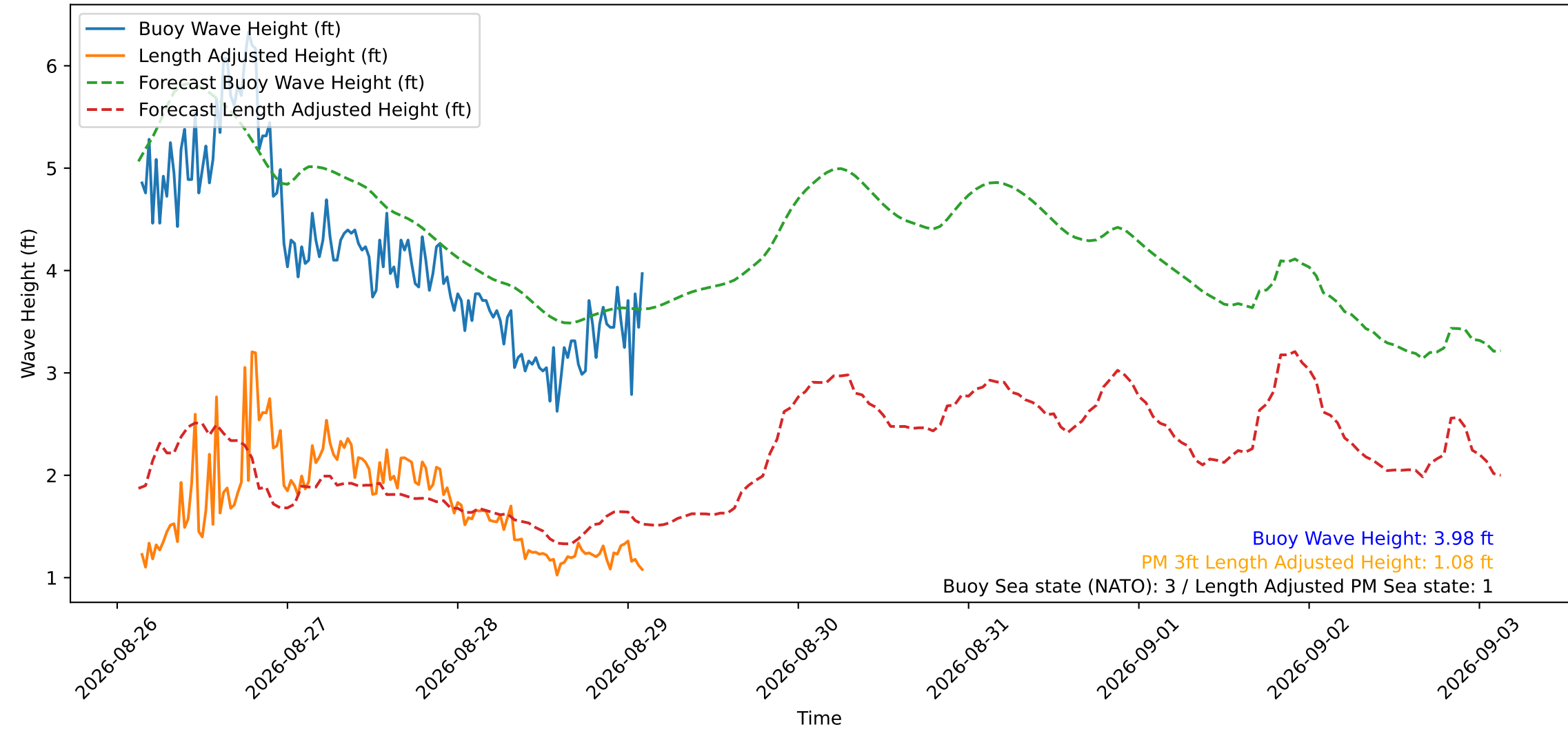
Wave Heights over Time for Green Beach at 2026-08-29 03:01:11
