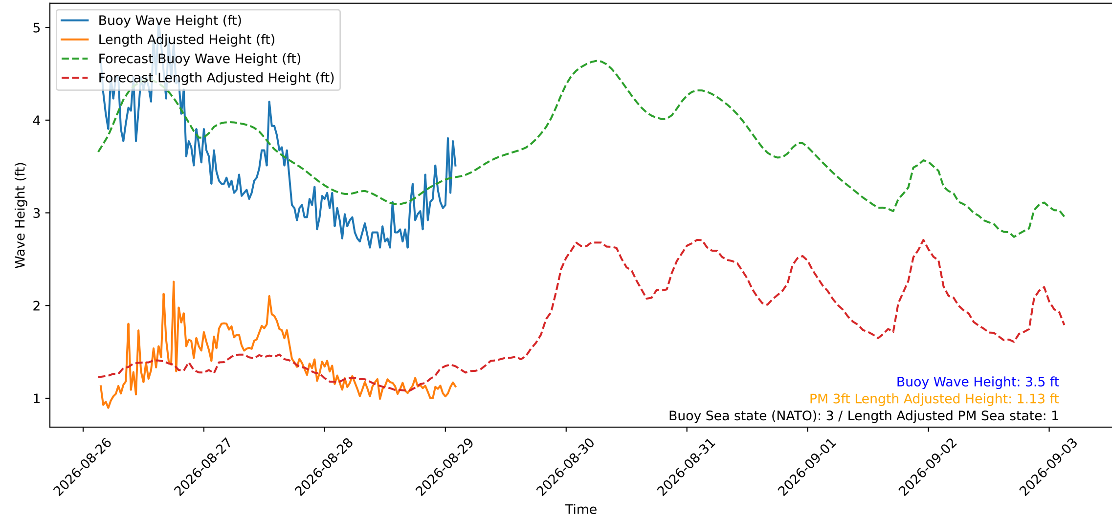
Wave Heights over Time for Red Beach at 2026-08-29 03:00:48
