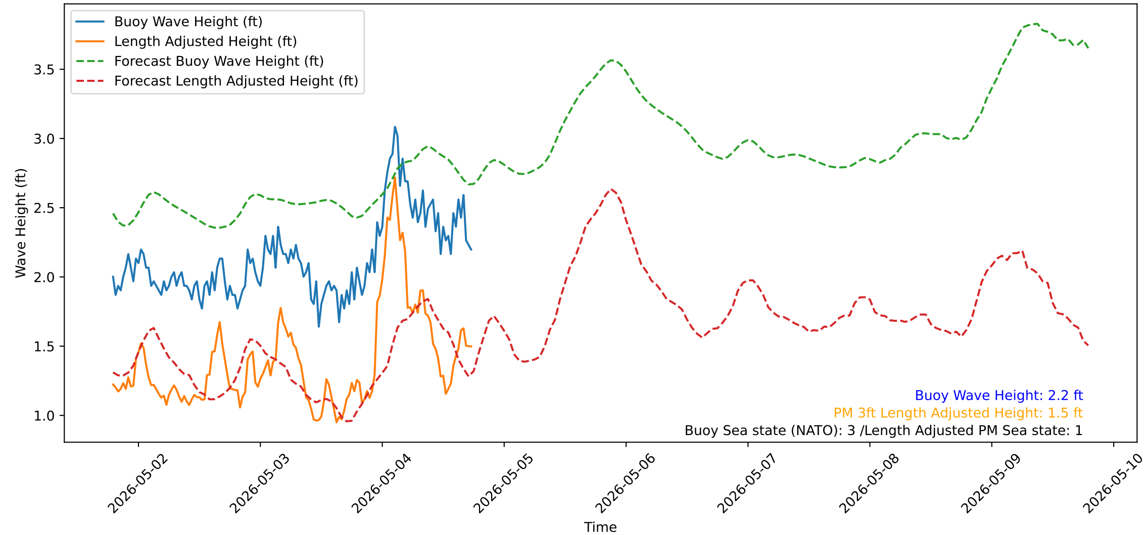
Wave Heights over Time for Oceanside Harbor at 2026-05-04 18:50:31
