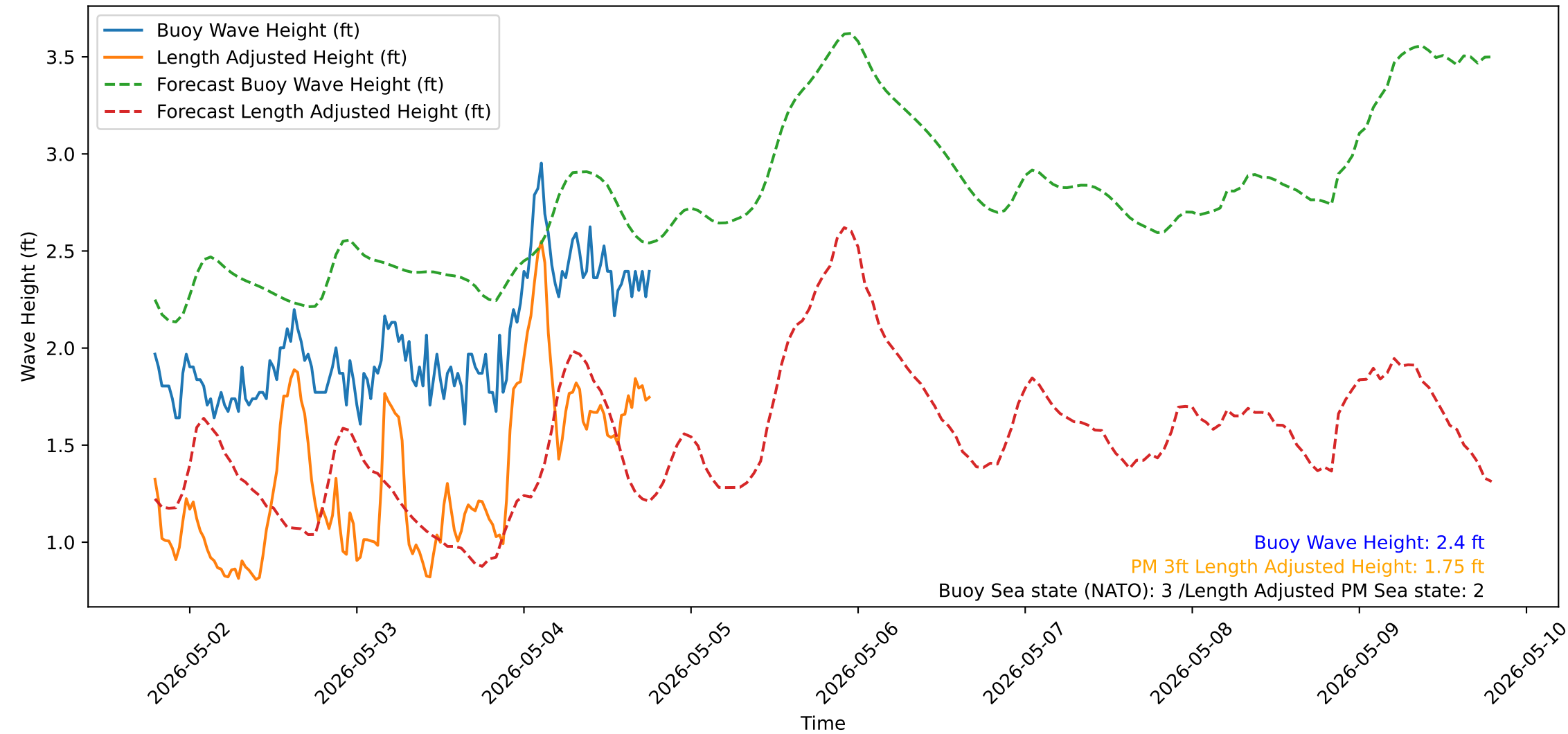
Wave Heights over Time for Red Beach at 2026-05-04 18:50:51
