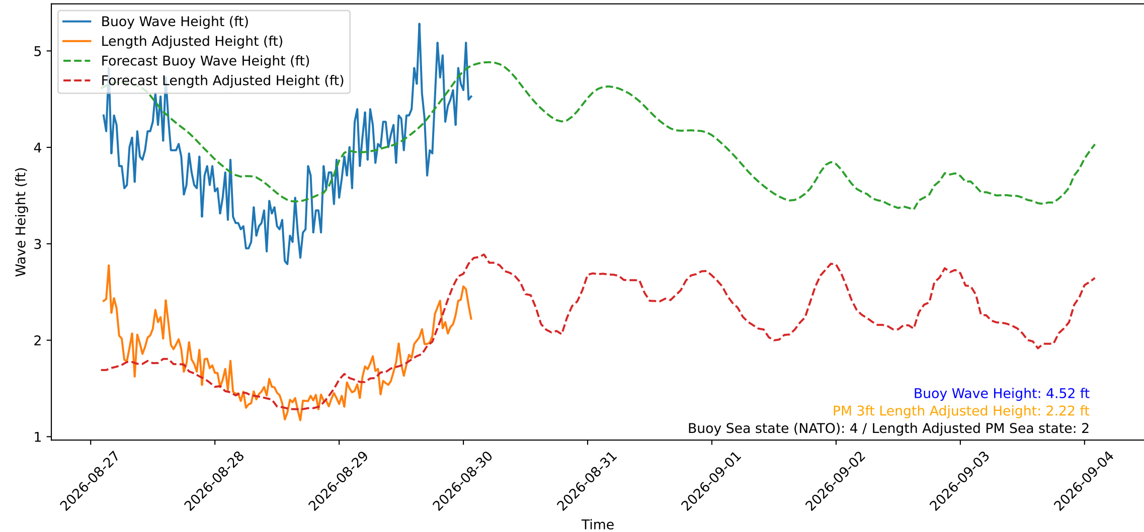
Wave Heights over Time for Oceanside Harbor at 2026-08-30 02:20:29
