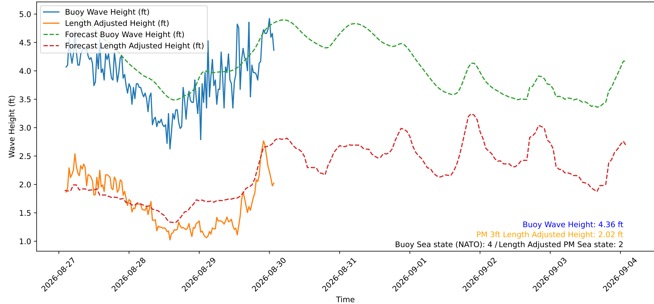
Wave Heights over Time for Green Beach at 2026-08-30 02:21:15
