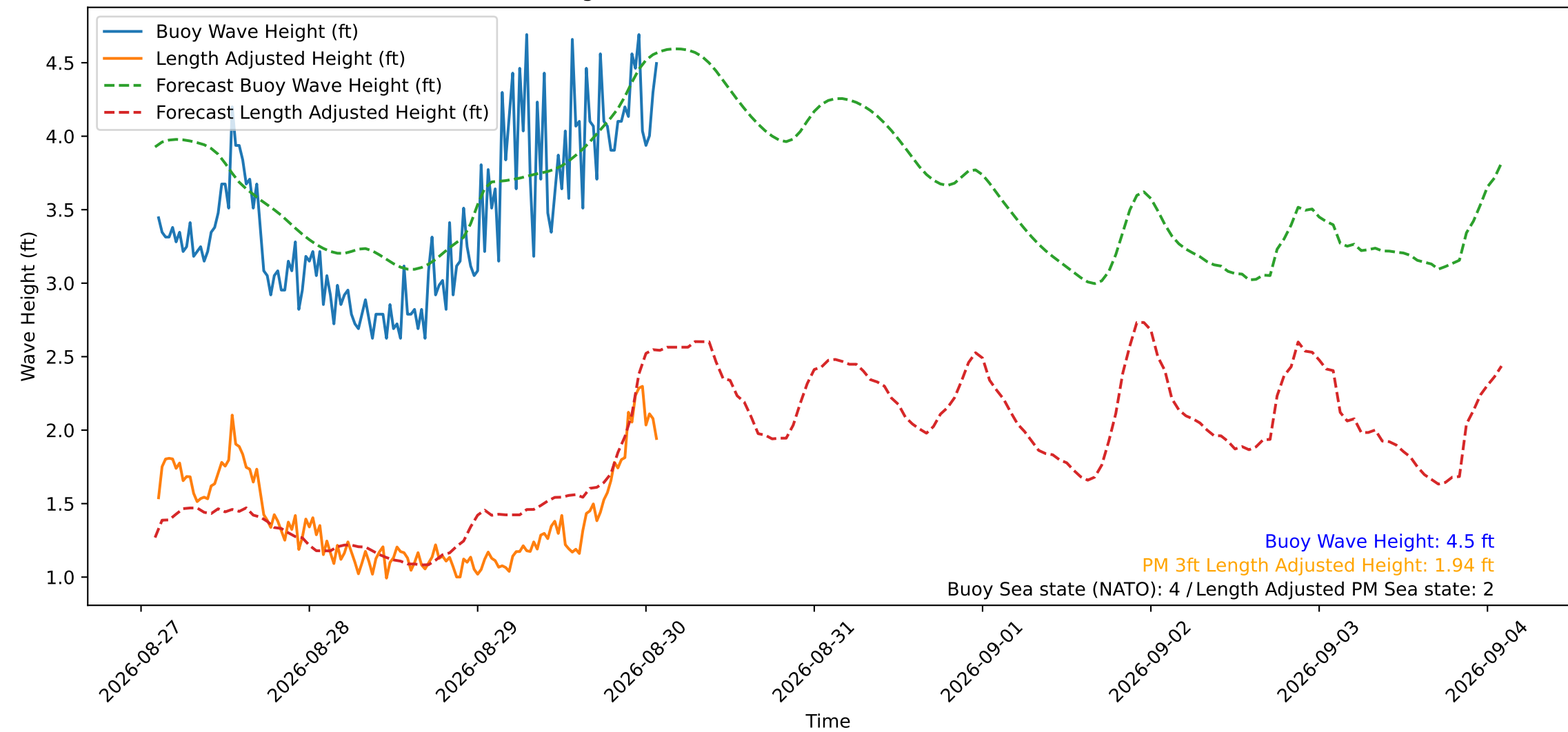
Wave Heights over Time for Red Beach at 2026-08-30 02:20:50
