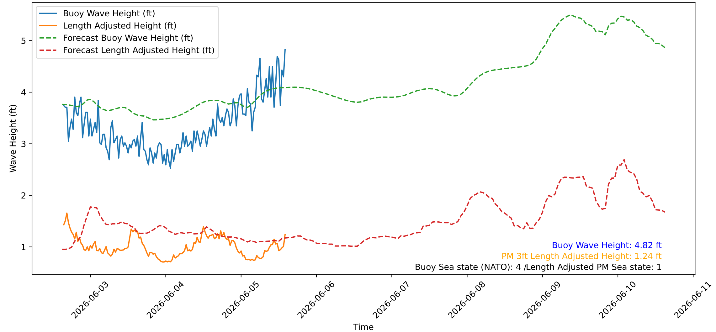
Wave Heights over Time for Red Beach at 2026-06-05 15:00:45
