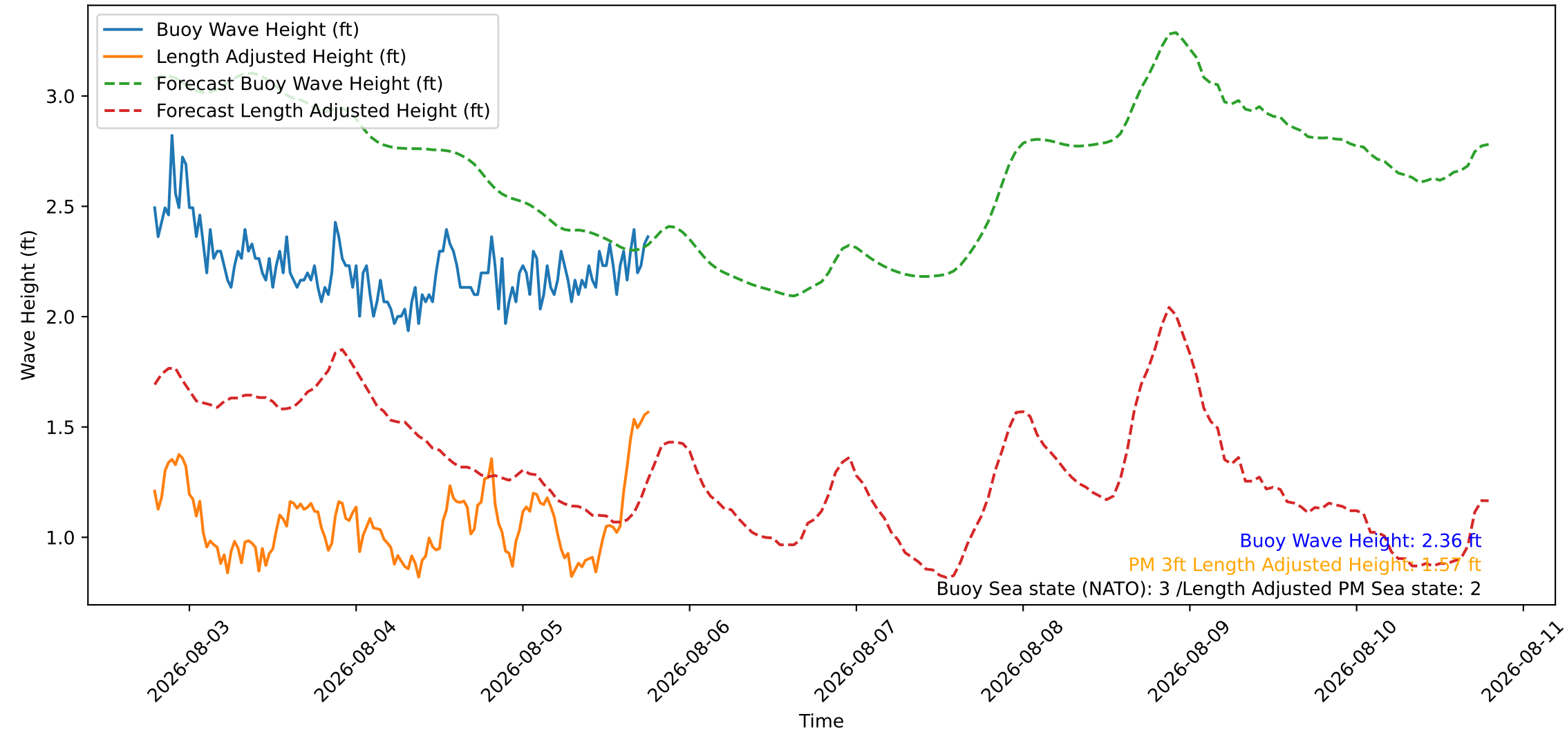
Wave Heights over Time for Green Beach at 2026-08-05 19:01:08
