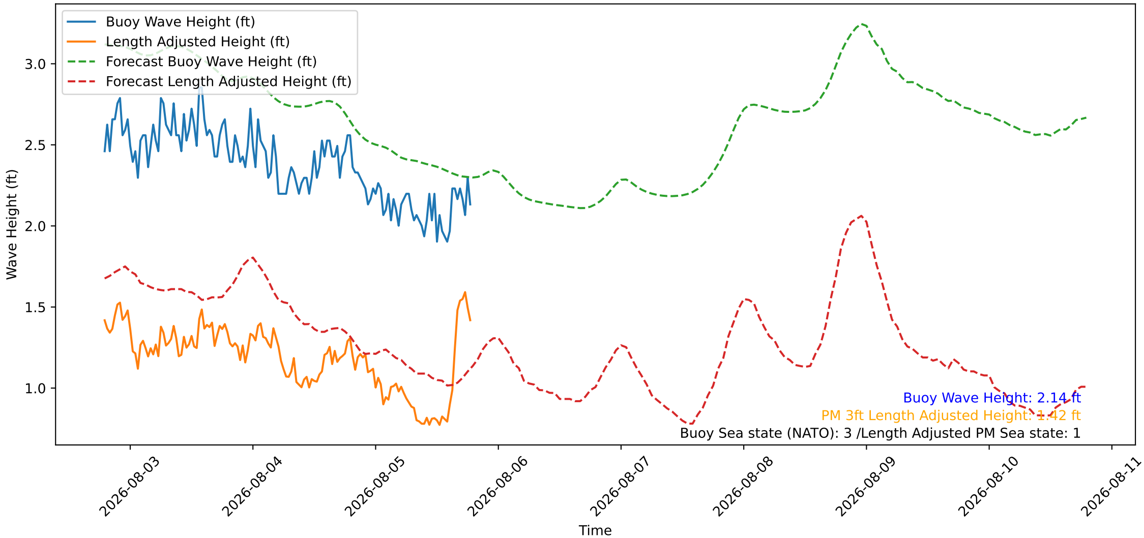
Wave Heights over Time for Oceanside Harbor at 2026-08-05 19:00:26
