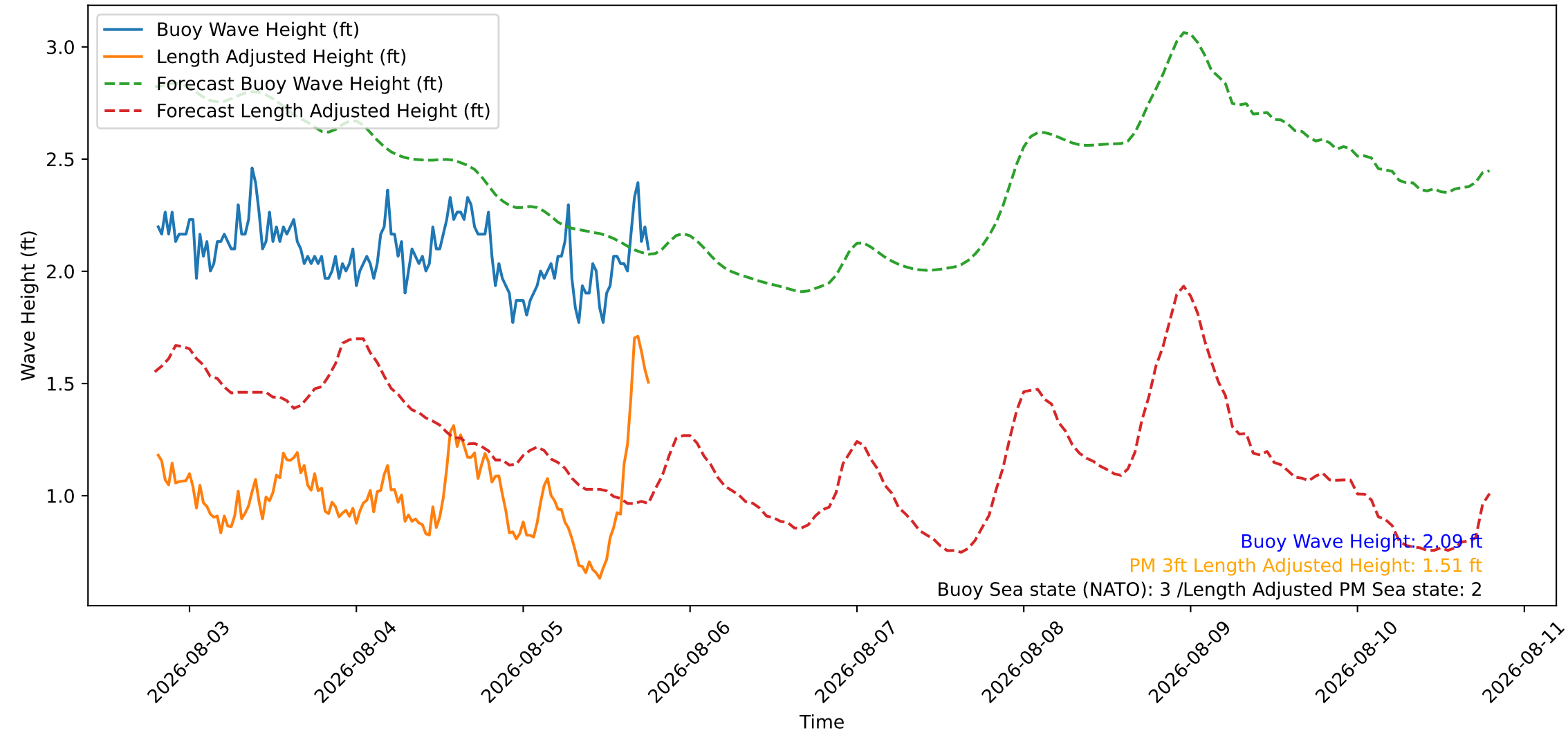
Wave Heights over Time for Red Beach at 2026-08-05 19:00:45
