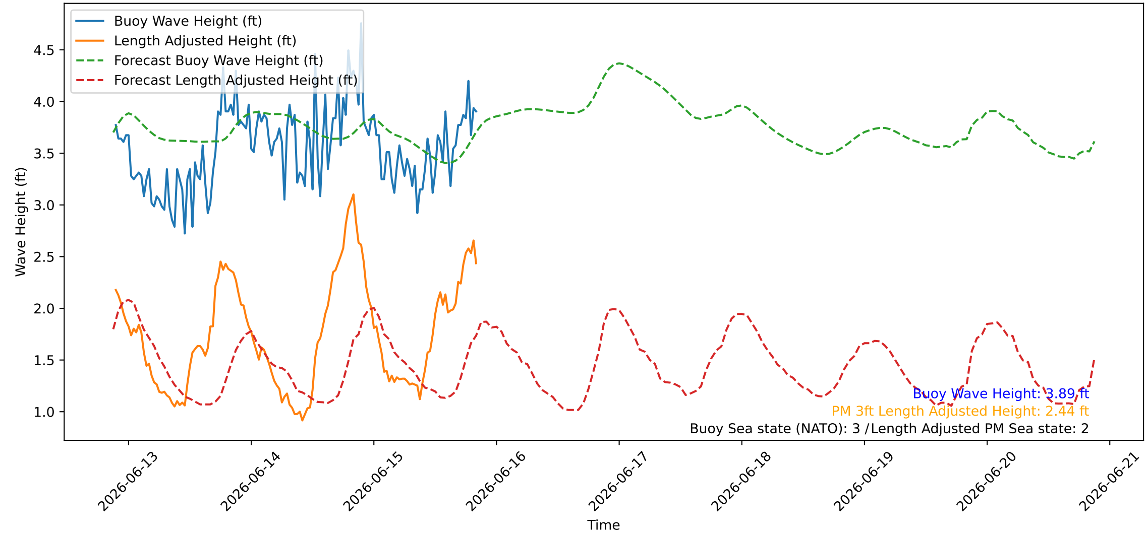
Wave Heights over Time for Red Beach at 2026-06-15 21:00:45
