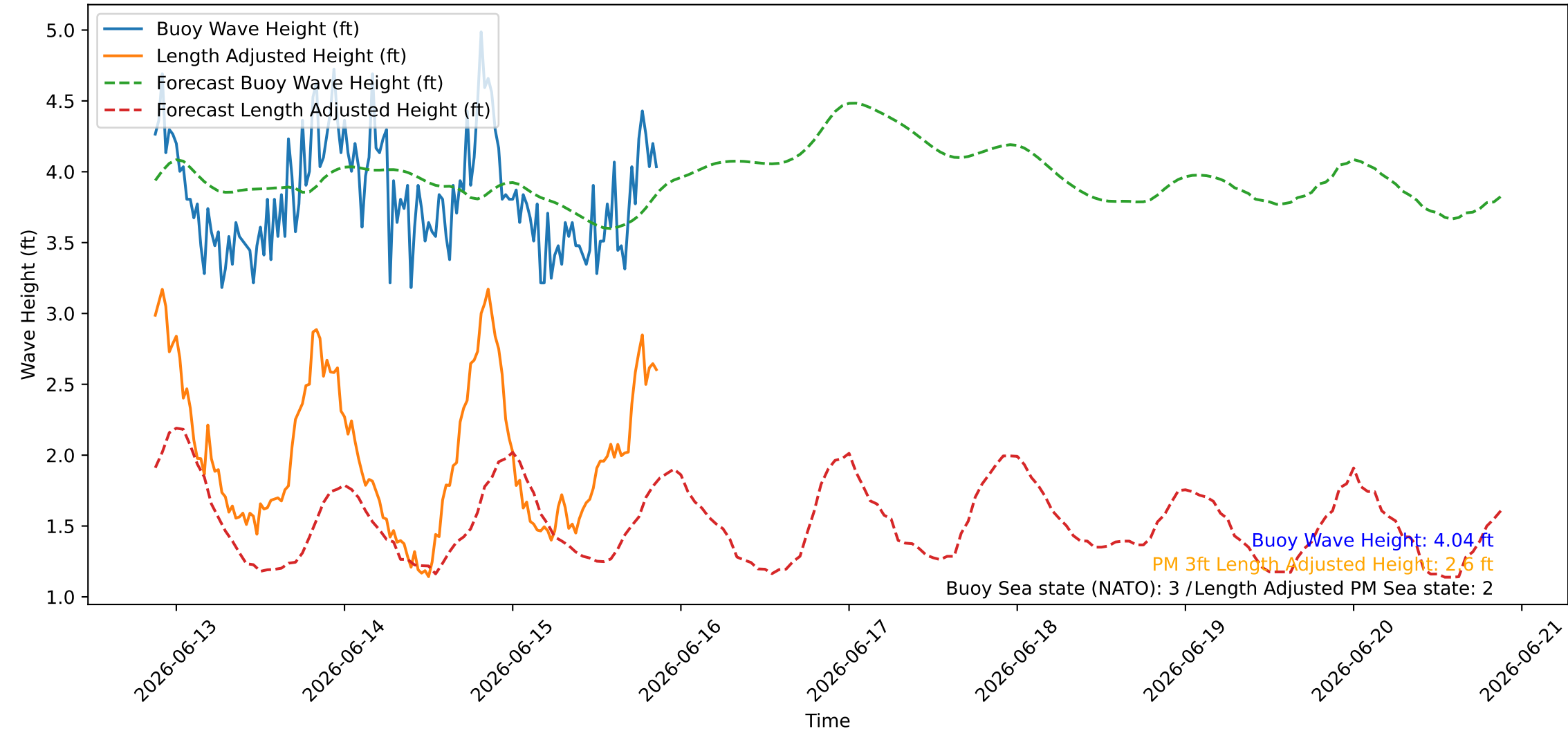
Wave Heights over Time for Oceanside Harbor at 2026-06-15 21:00:26
