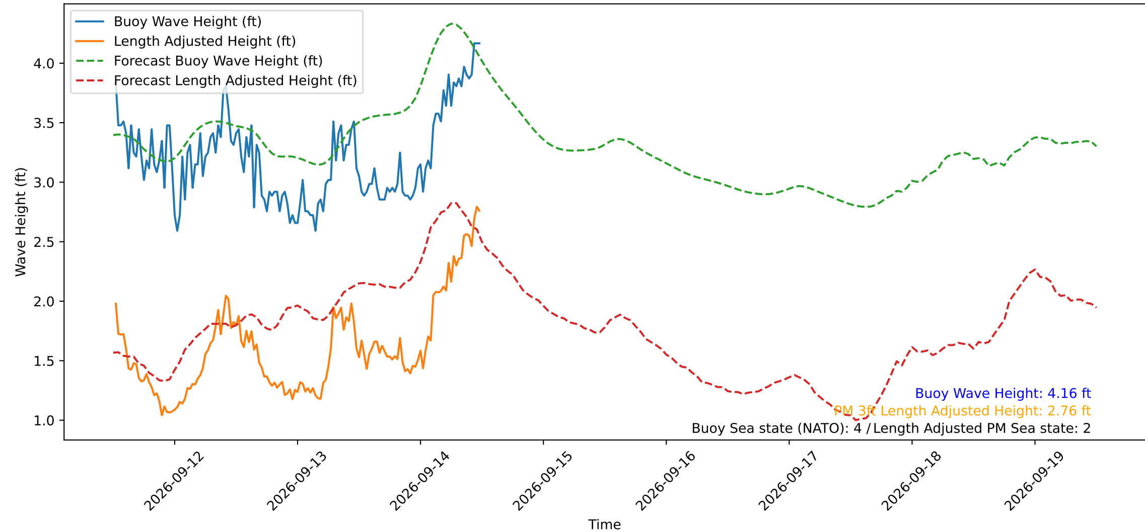
Wave Heights over Time for Oceanside Harbor at 2026-09-14 12:20:31
