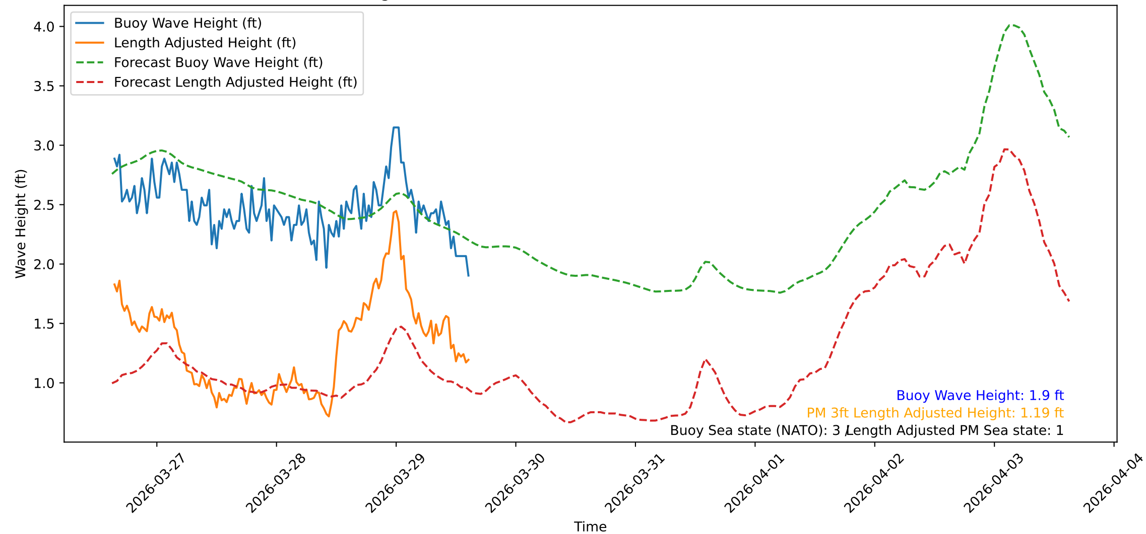
Wave Heights over Time for Oceanside Harbor at 2026-03-29 15:20:31
