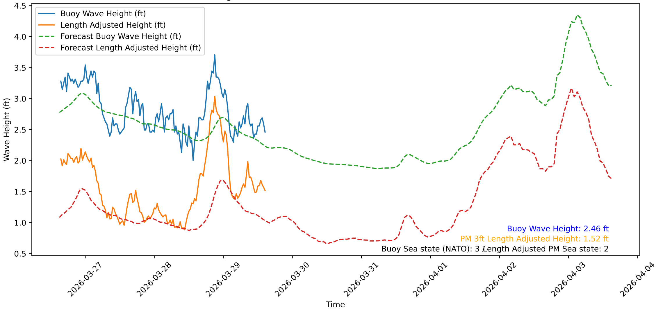
Wave Heights over Time for Green Beach at 2026-03-29 15:21:10
