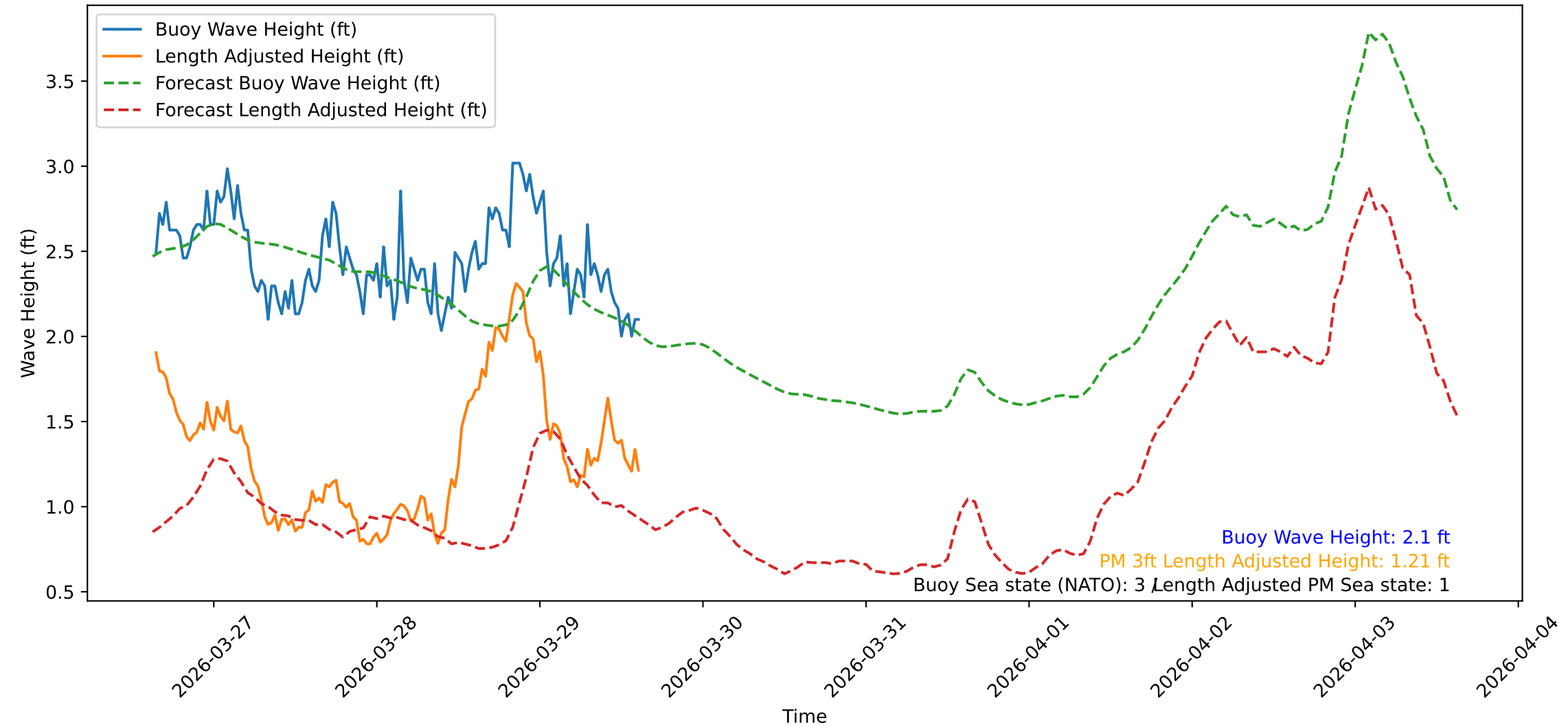
Wave Heights over Time for Red Beach at 2026-03-29 15:20:47
