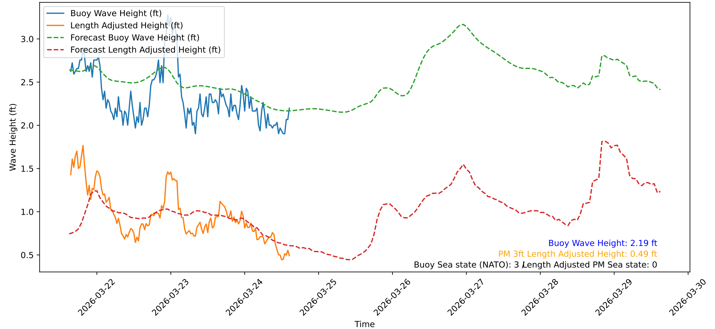
Wave Heights over Time for Green Beach at 2026-03-24 15:21:10
