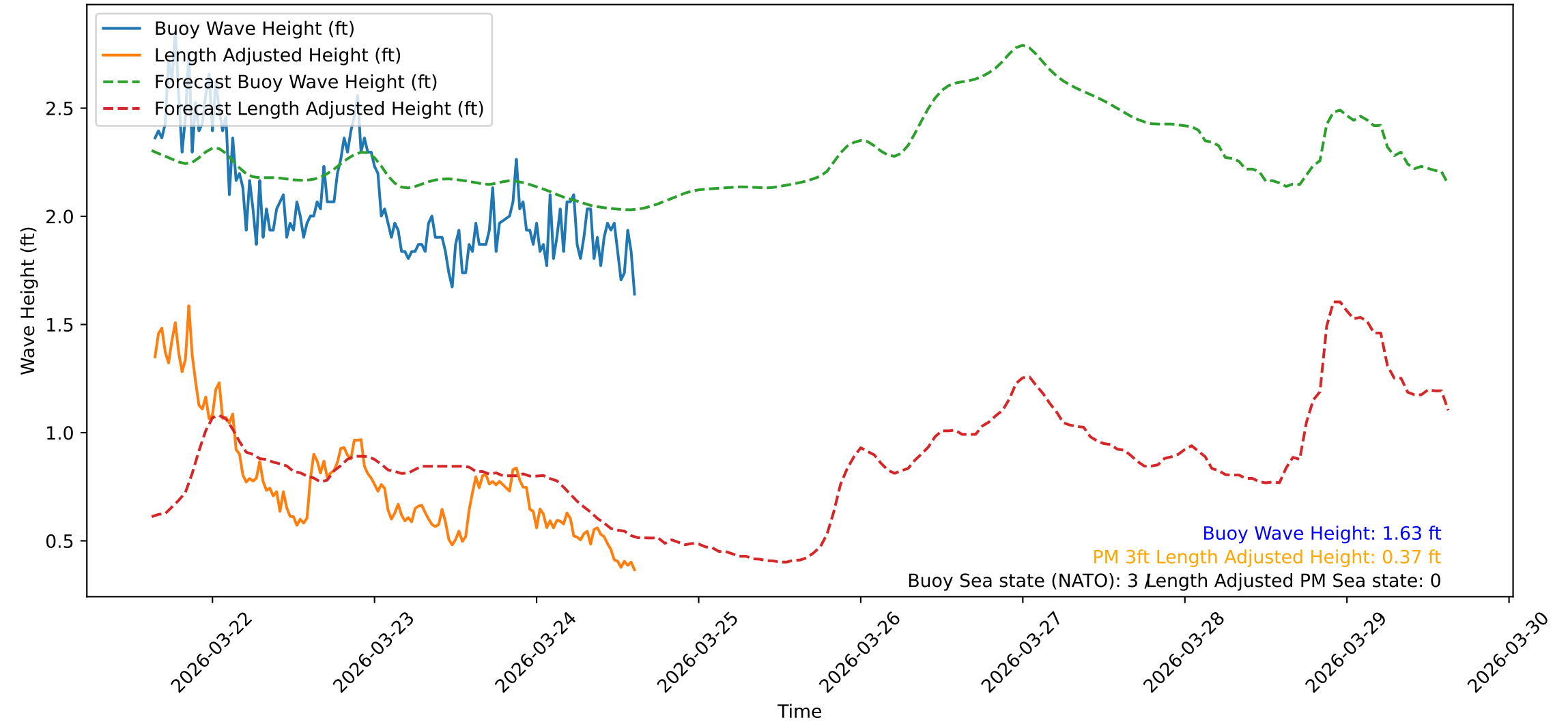
Wave Heights over Time for Red Beach at 2026-03-24 15:20:47
