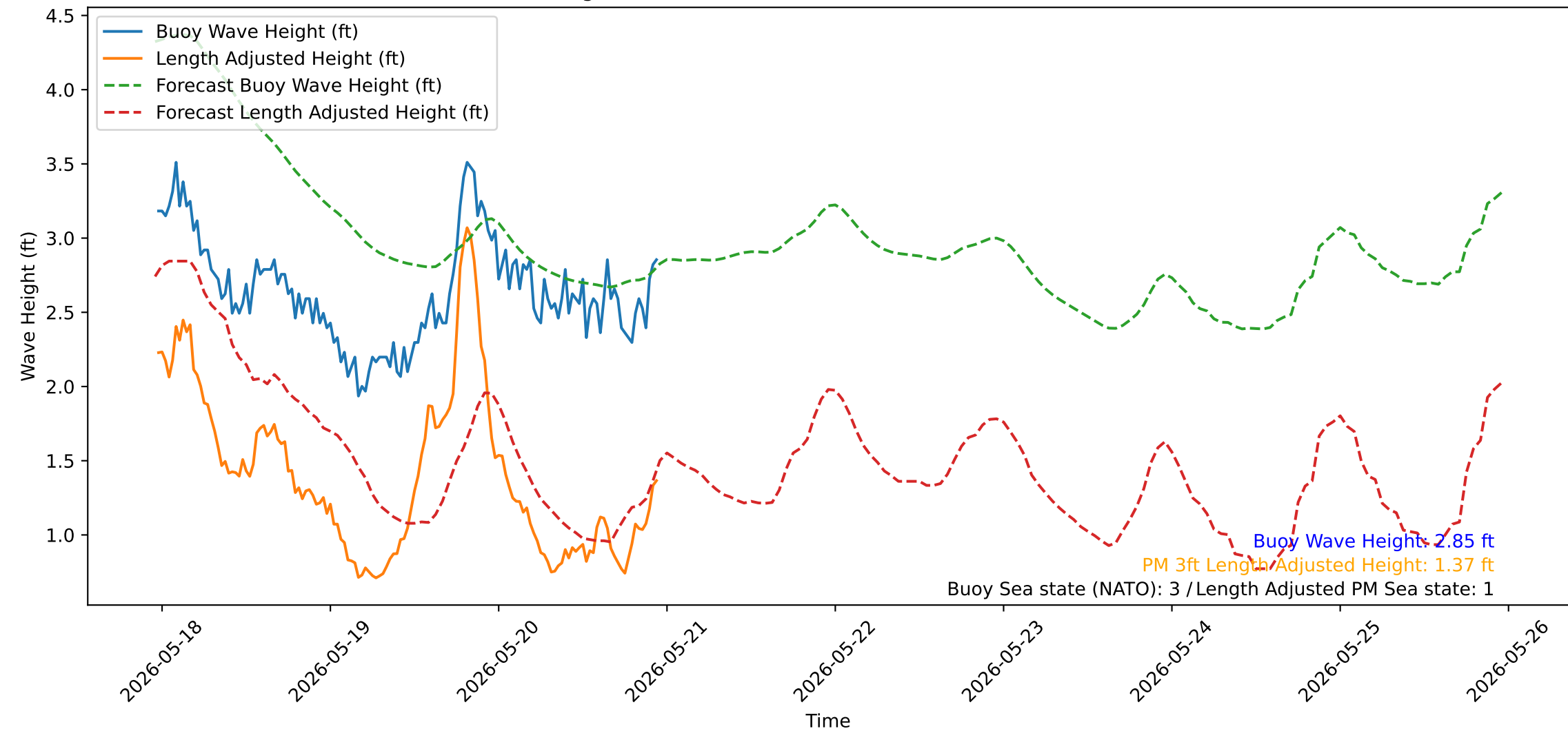
Wave Heights over Time for Red Beach at 2026-05-20 23:20:52
