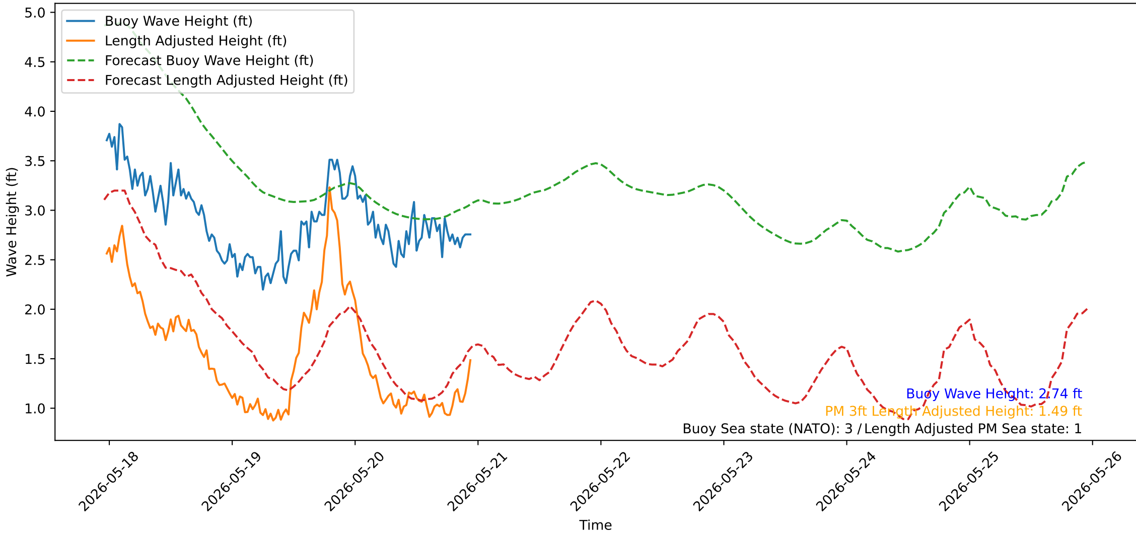
Wave Heights over Time for Oceanside Harbor at 2026-05-20 23:20:32
