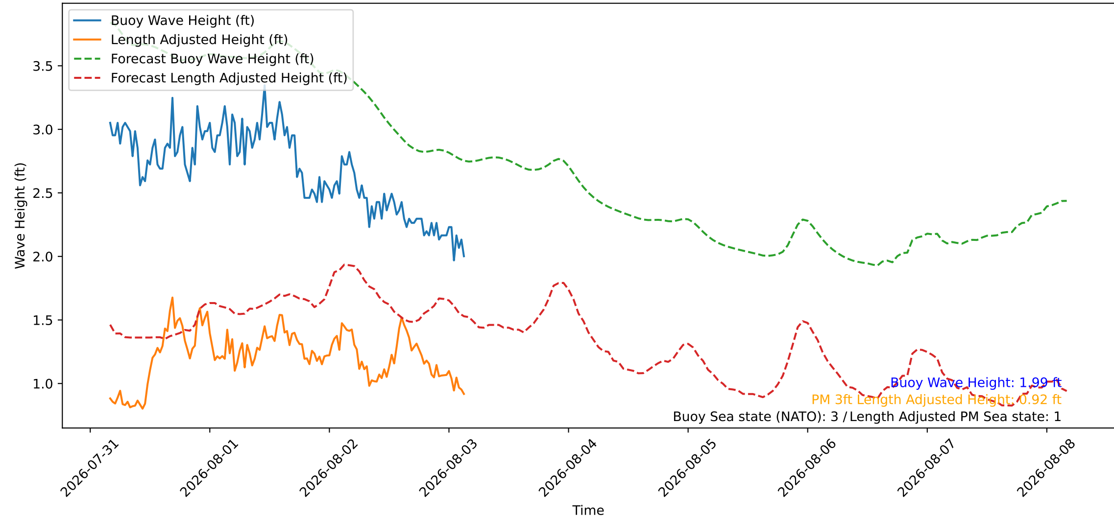
Wave Heights over Time for Red Beach at 2026-08-03 03:50:47
