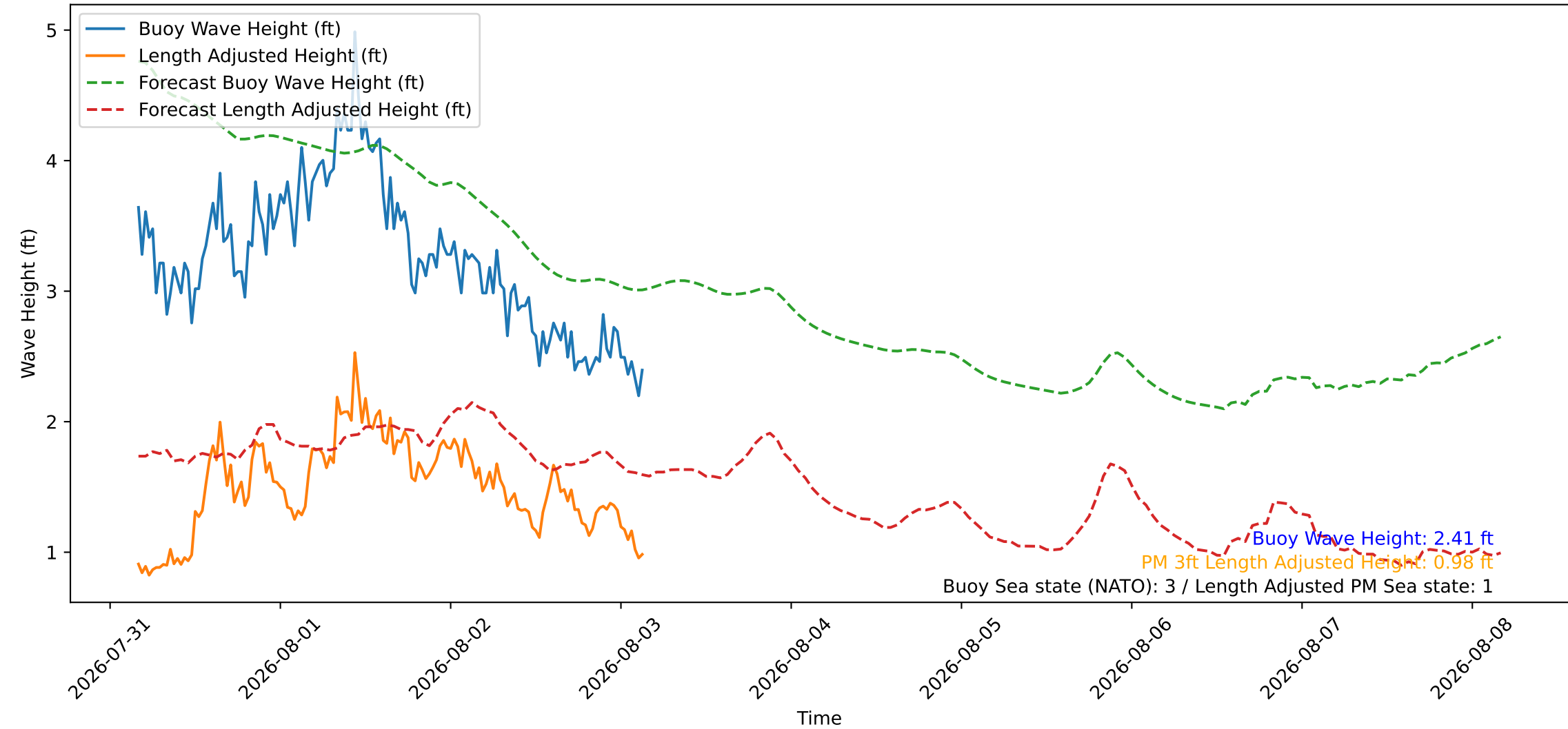
Wave Heights over Time for Green Beach at 2026-08-03 03:51:09
