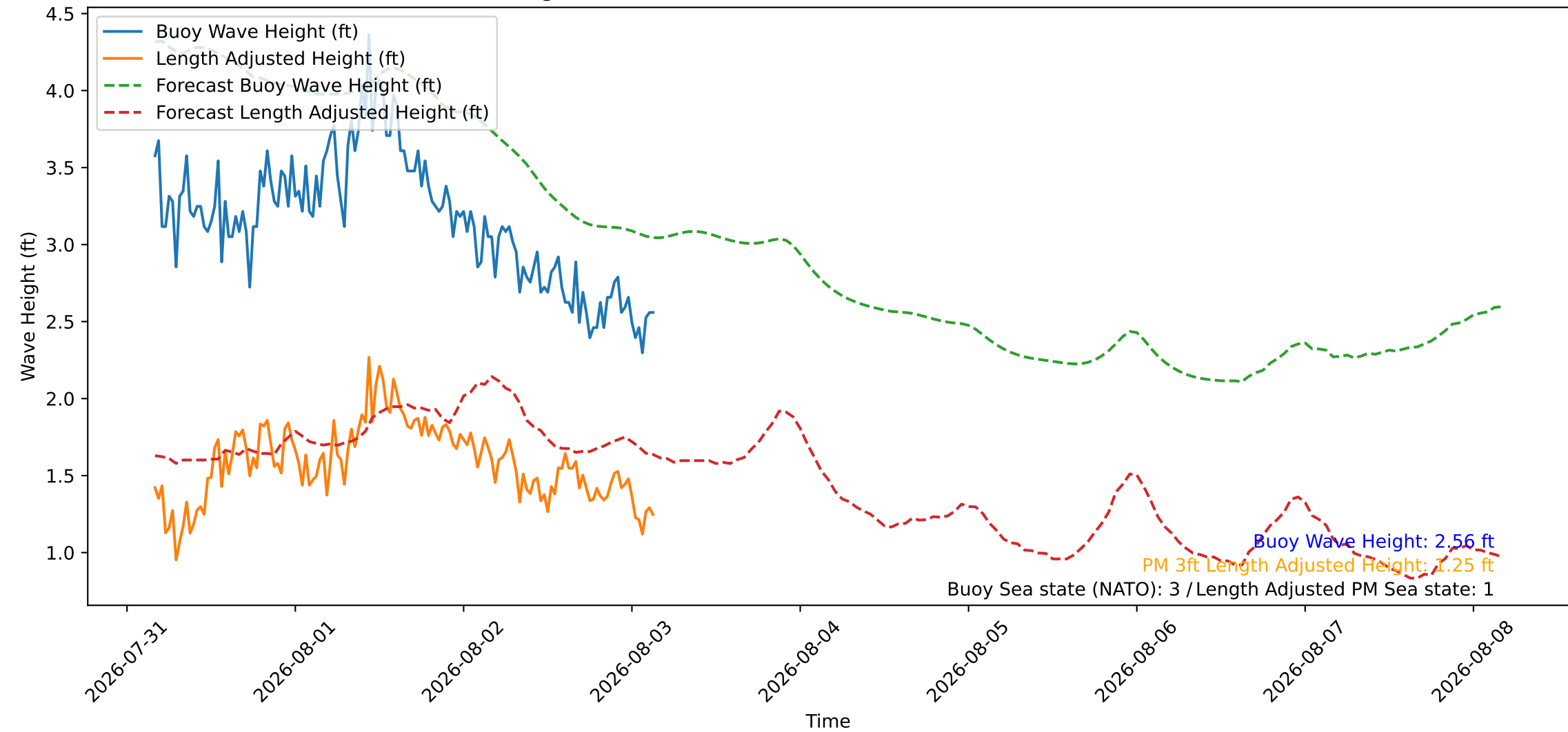
Wave Heights over Time for Oceanside Harbor at 2026-08-03 03:50:26
