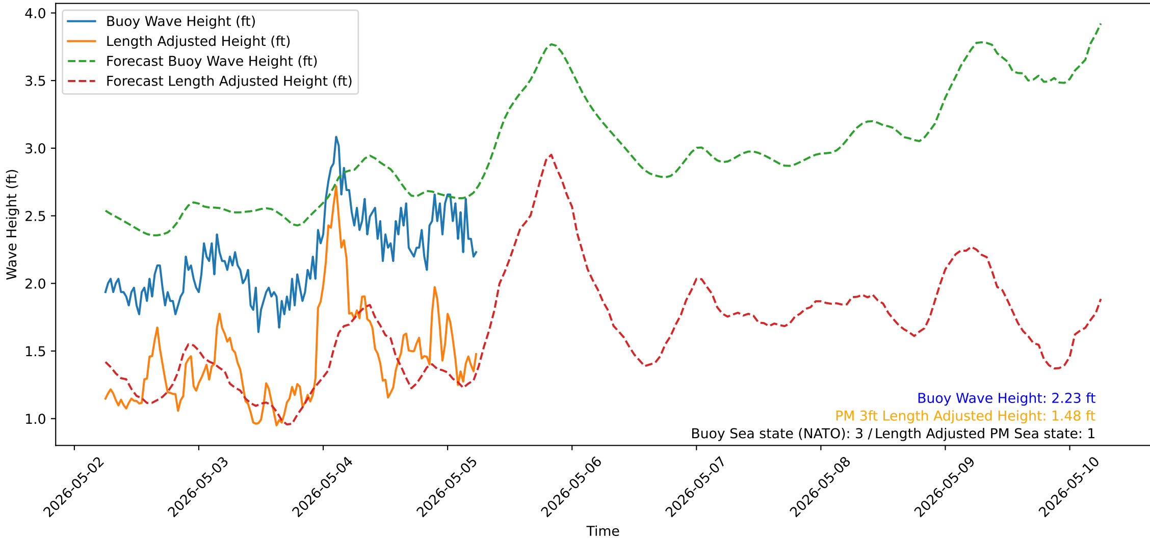
Wave Heights over Time for Oceanside Harbor at 2026-05-05 06:00:31
