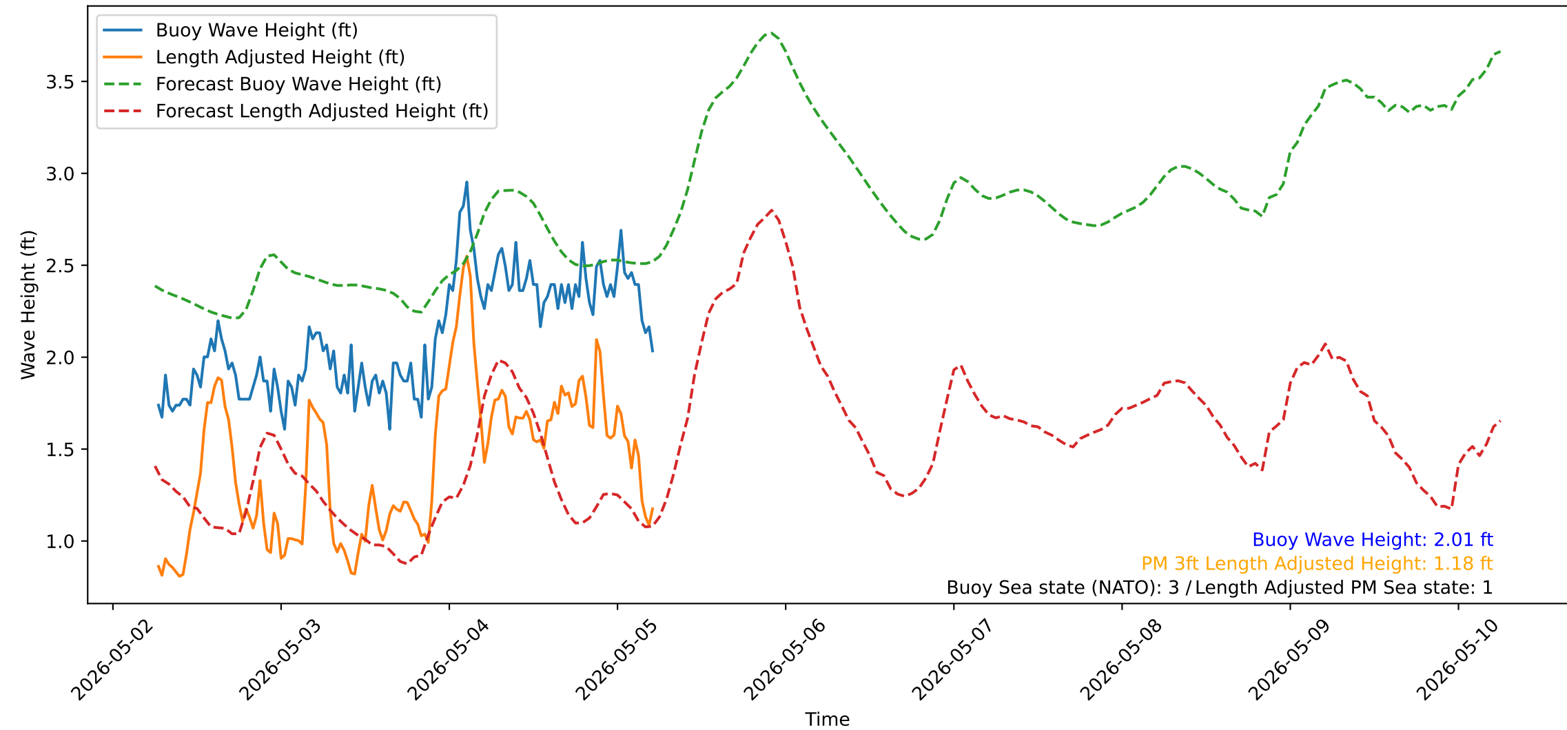
Wave Heights over Time for Red Beach at 2026-05-05 06:00:51
