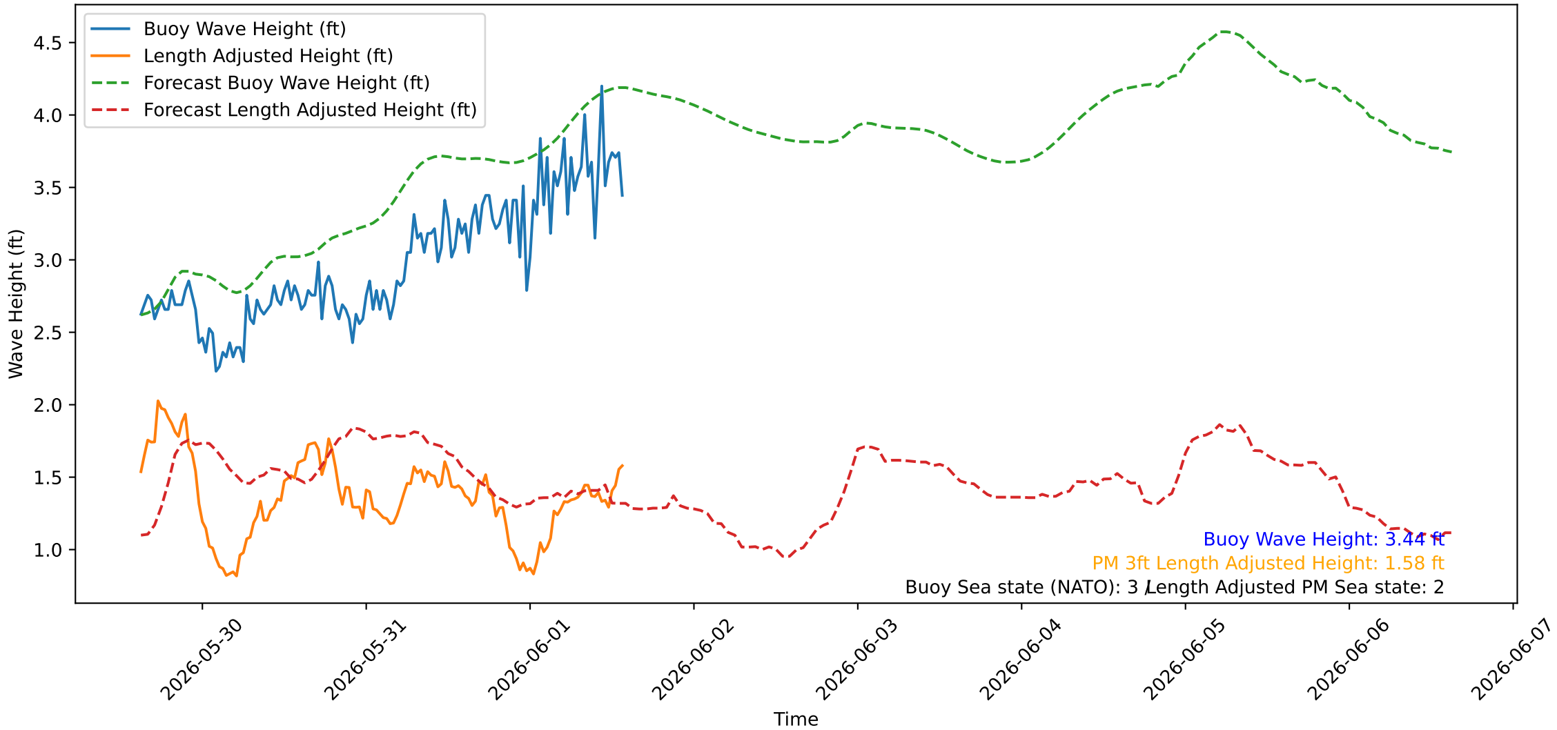
Wave Heights over Time for Red Beach at 2026-06-01 14:40:45
