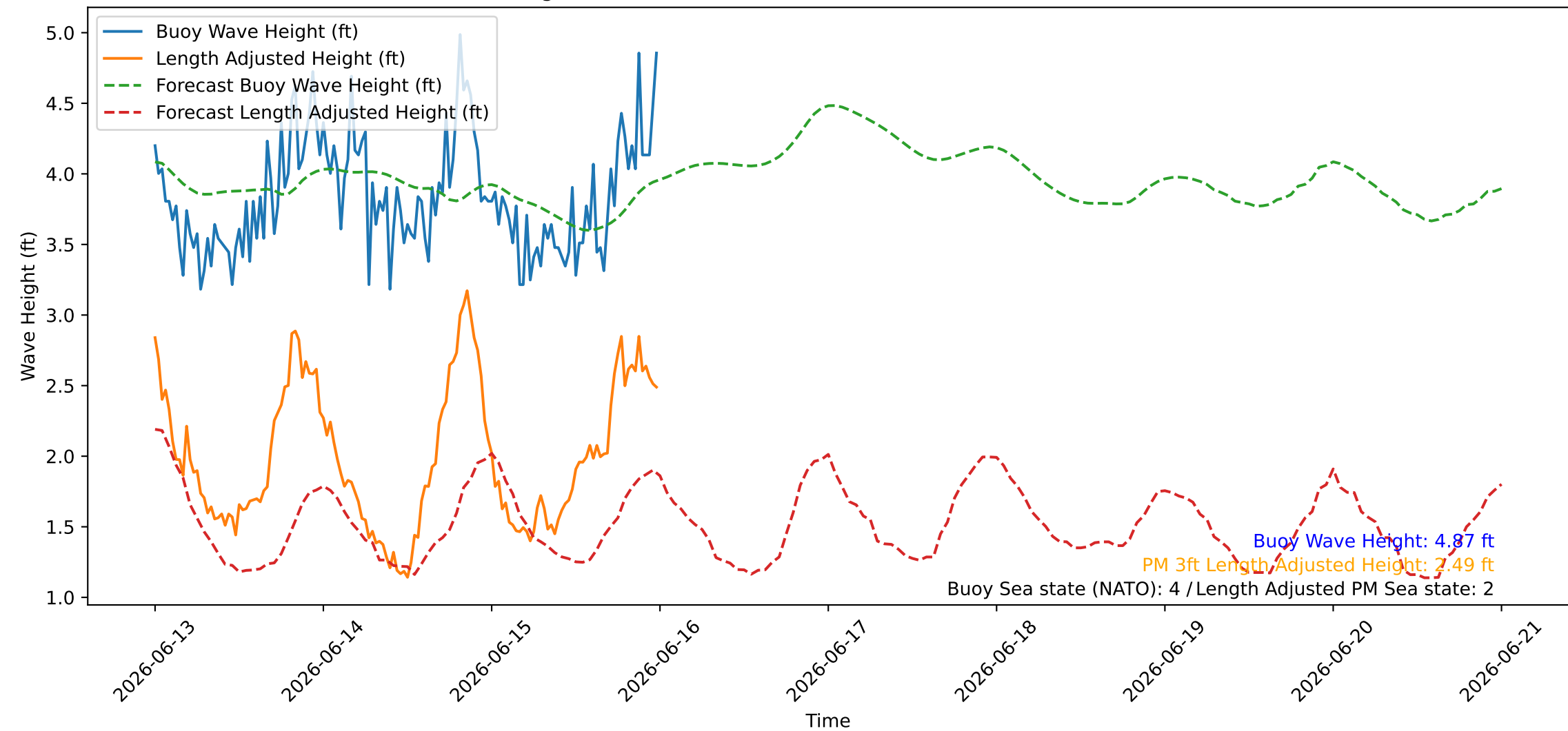
Wave Heights over Time for Oceanside Harbor at 2026-06-16 00:10:25
