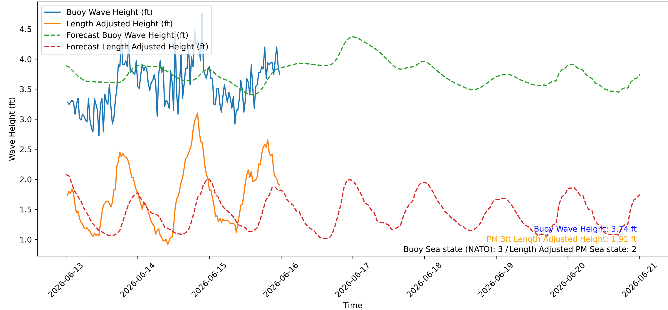
Wave Heights over Time for Red Beach at 2026-06-16 00:10:45
