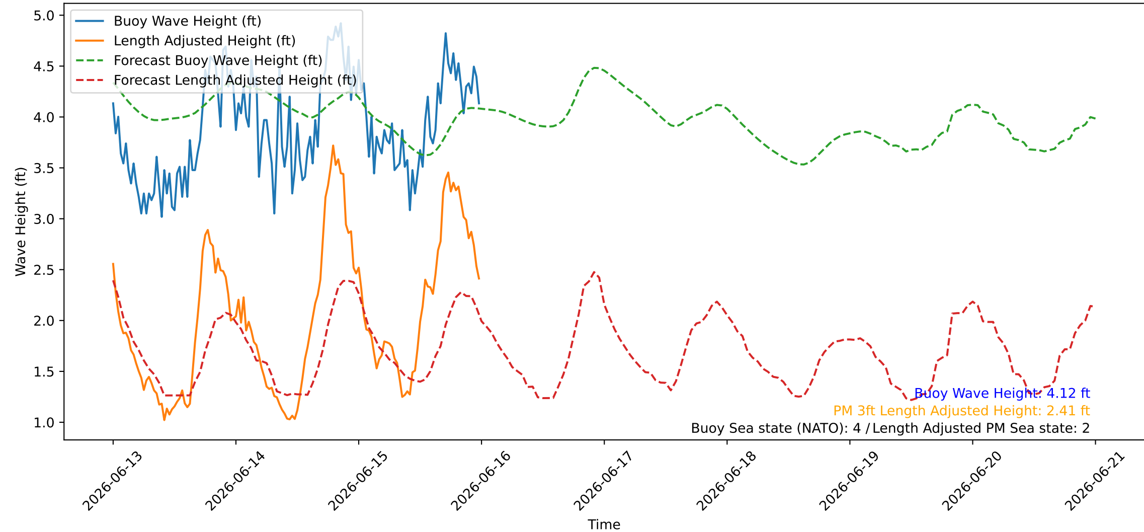
Wave Heights over Time for Green Beach at 2026-06-16 00:11:07
