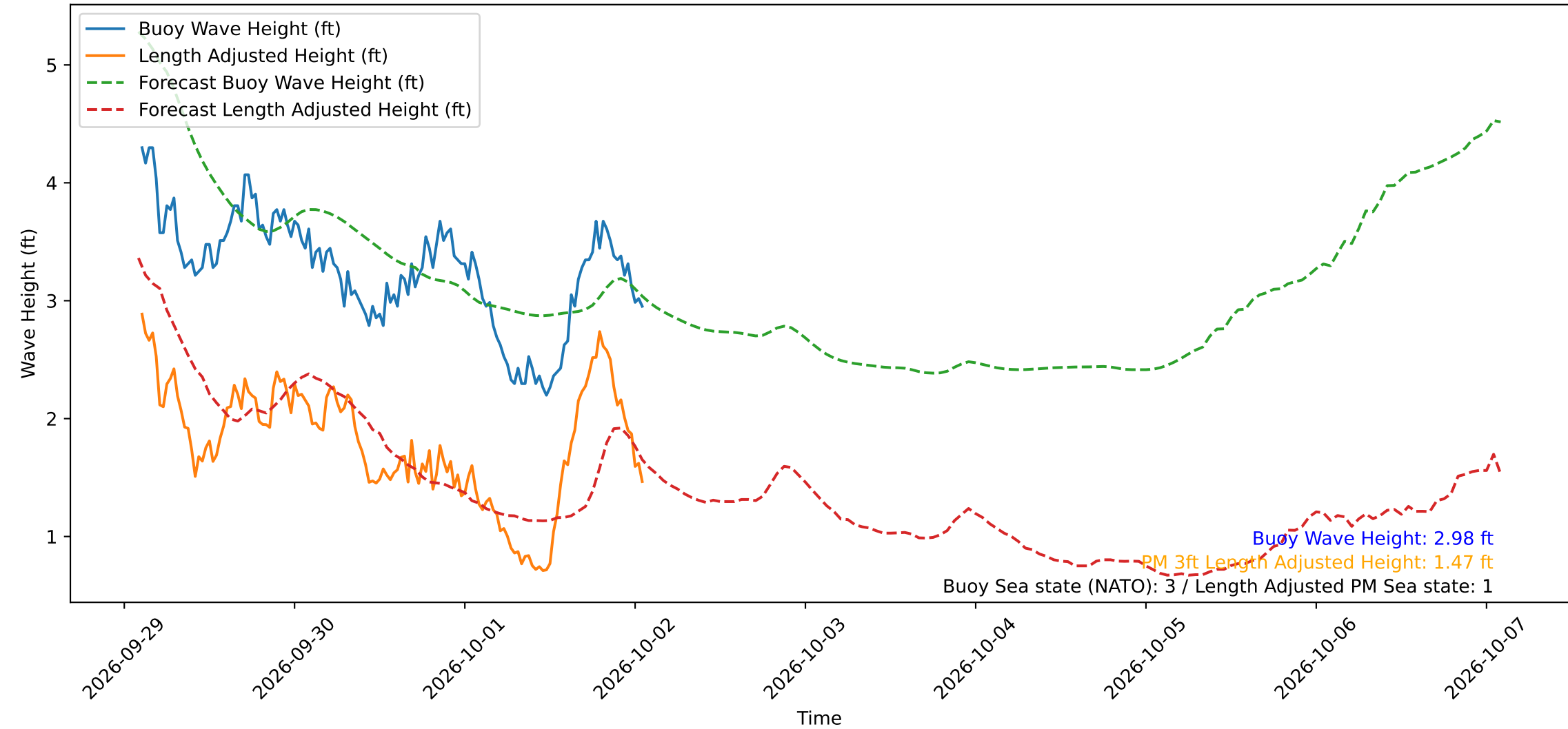
Wave Heights over Time for Green Beach at 2026-10-02 02:01:12
