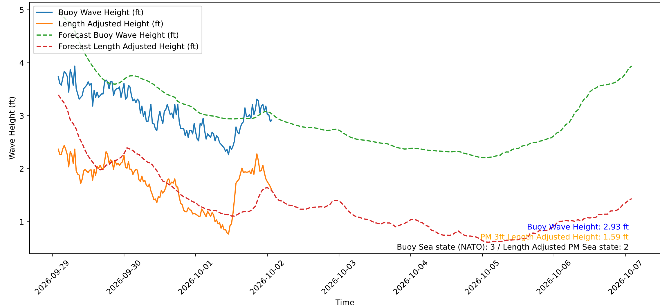
Wave Heights over Time for Oceanside Harbor at 2026-10-02 02:00:30
