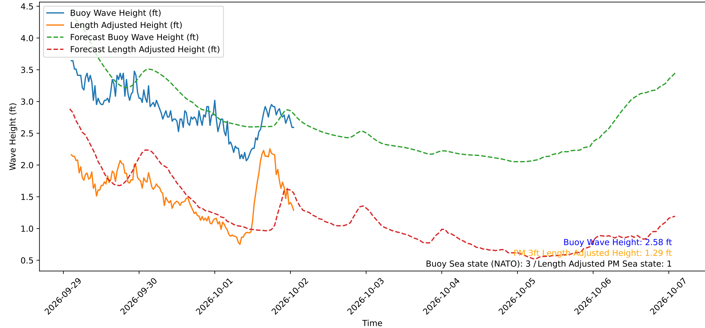
Wave Heights over Time for Red Beach at 2026-10-02 02:00:49
