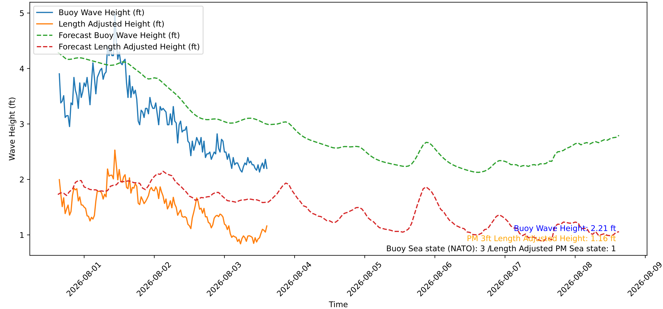
Wave Heights over Time for Green Beach at 2026-08-03 15:21:10
