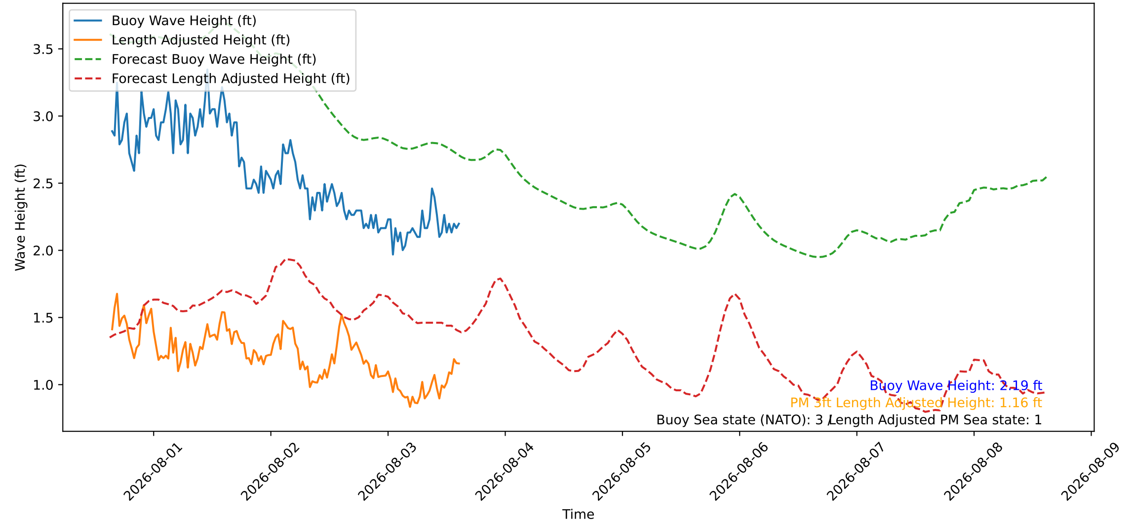
Wave Heights over Time for Red Beach at 2026-08-03 15:20:47
