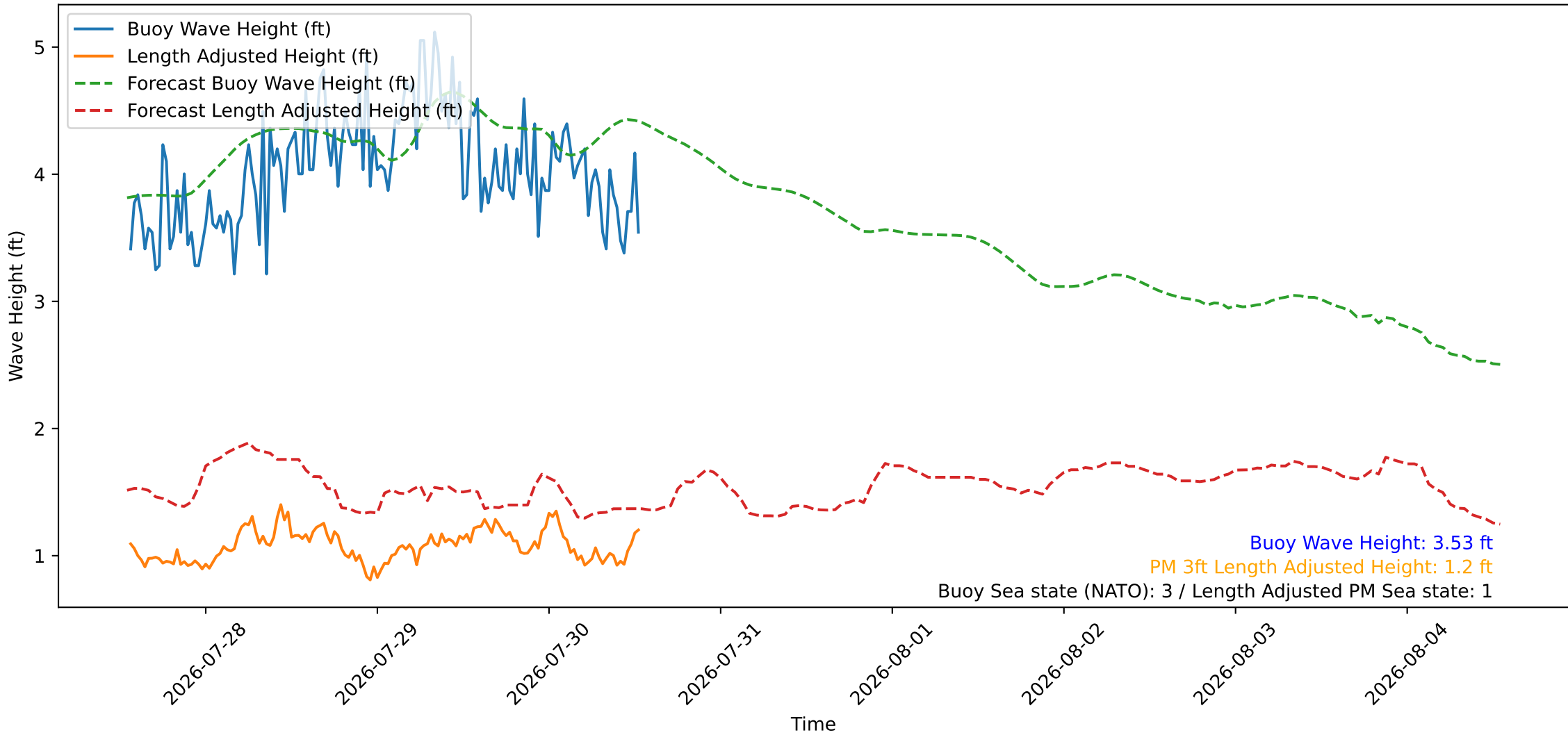
Wave Heights over Time for Red Beach at 2026-07-30 13:10:45
