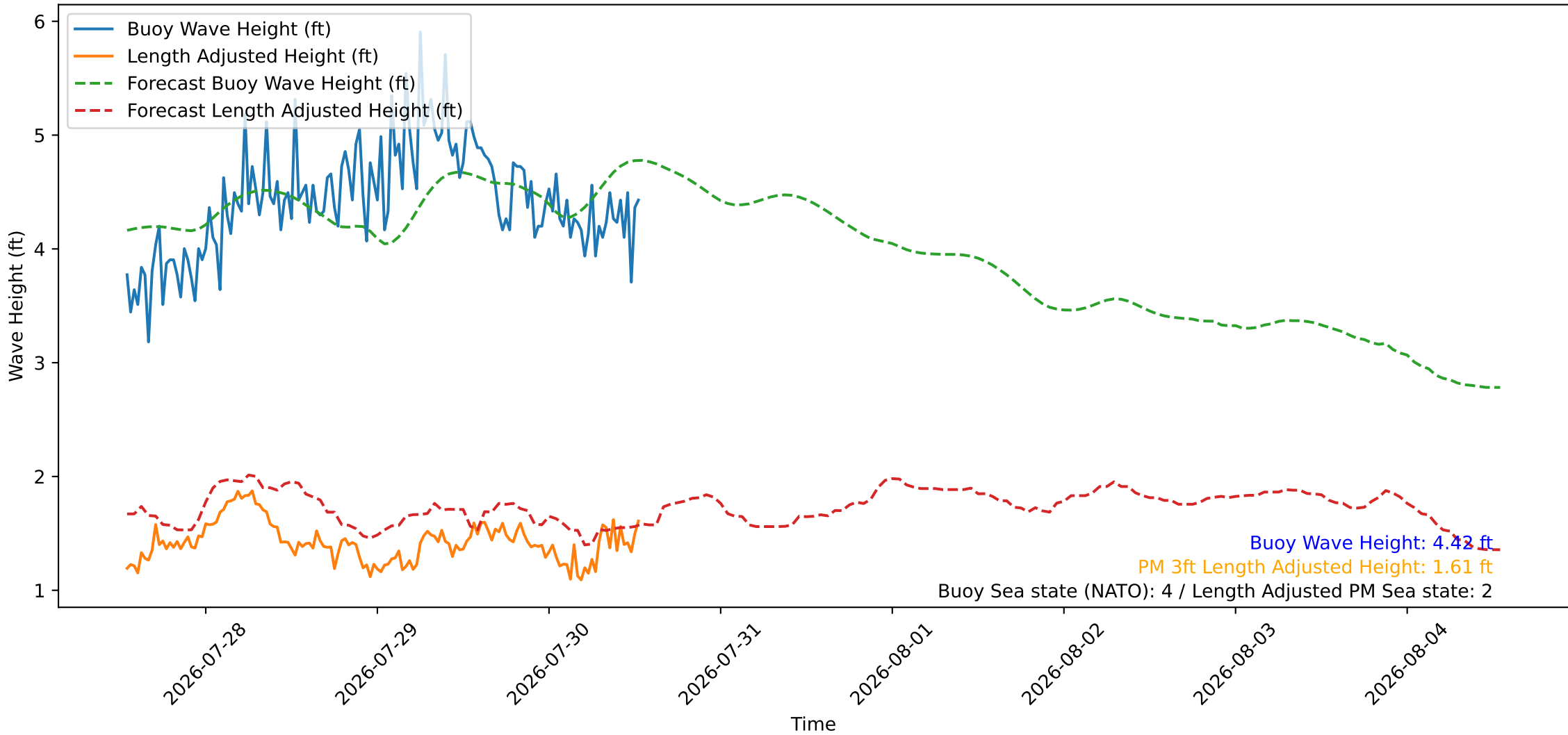
Wave Heights over Time for Oceanside Harbor at 2026-07-30 13:10:26
