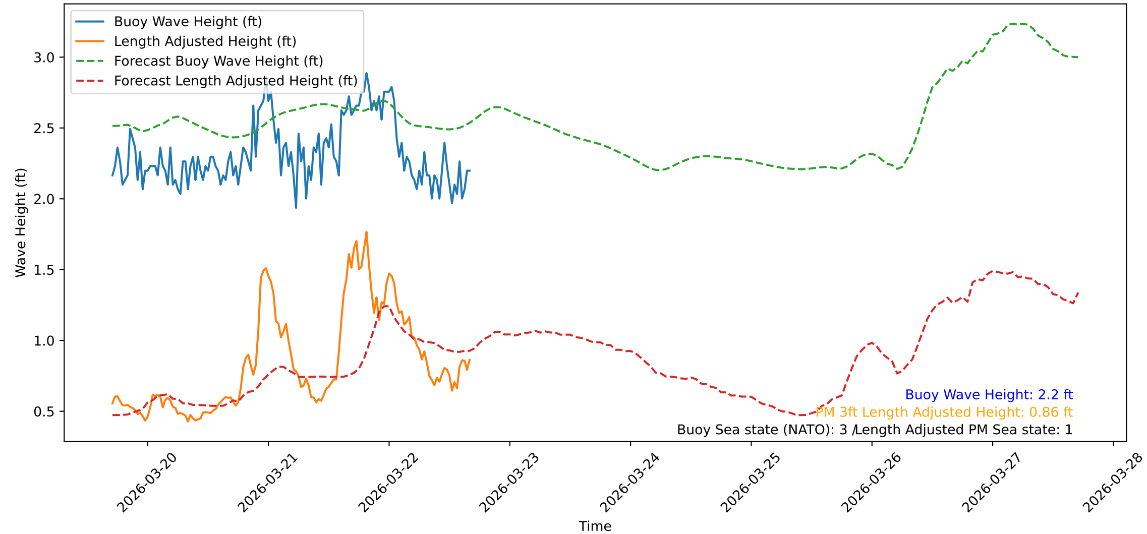
Wave Heights over Time for Green Beach at 2026-03-22 17:01:09
