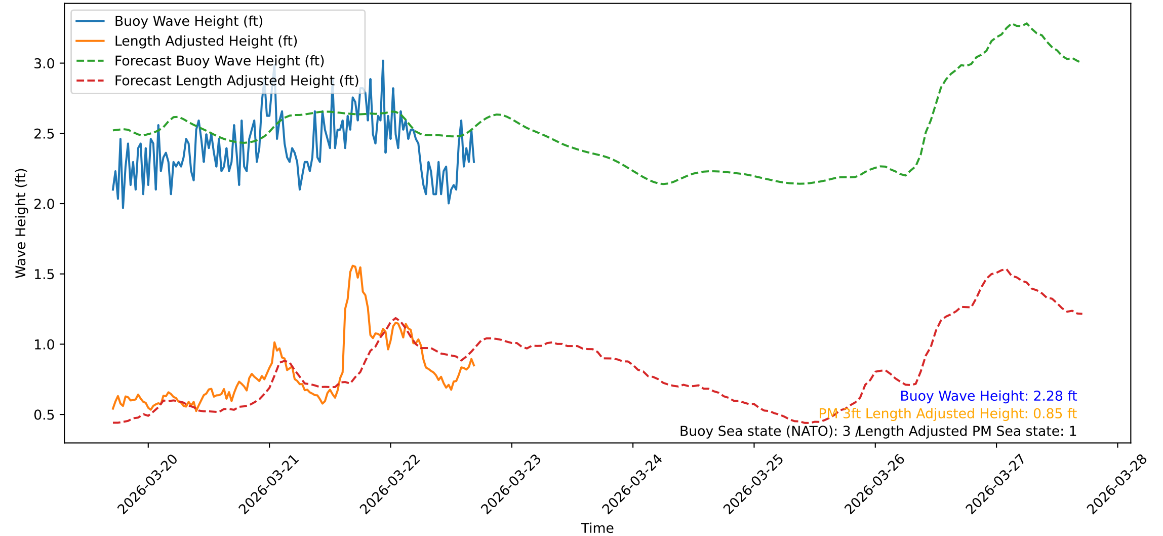
Wave Heights over Time for Oceanside Harbor at 2026-03-22 17:00:31
