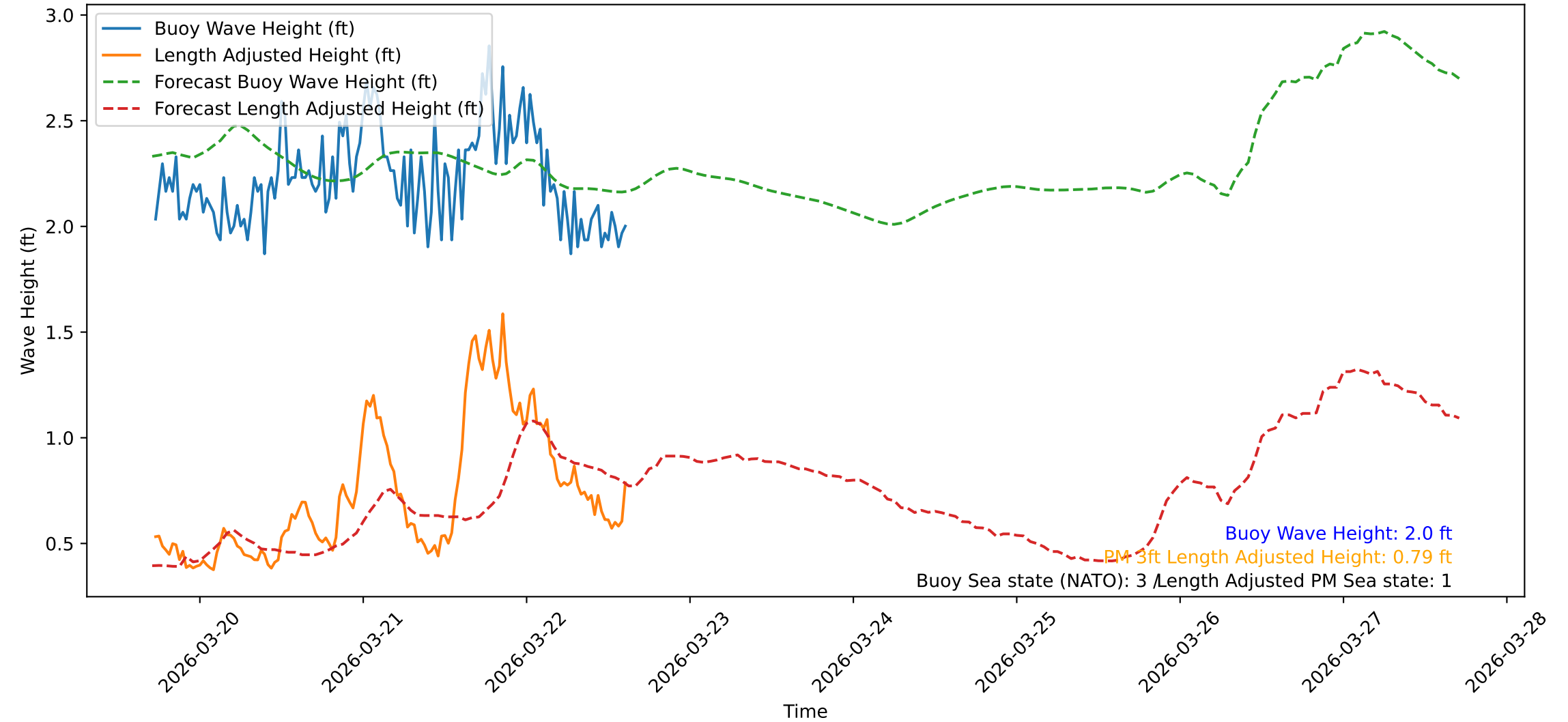
Wave Heights over Time for Red Beach at 2026-03-22 17:00:47
