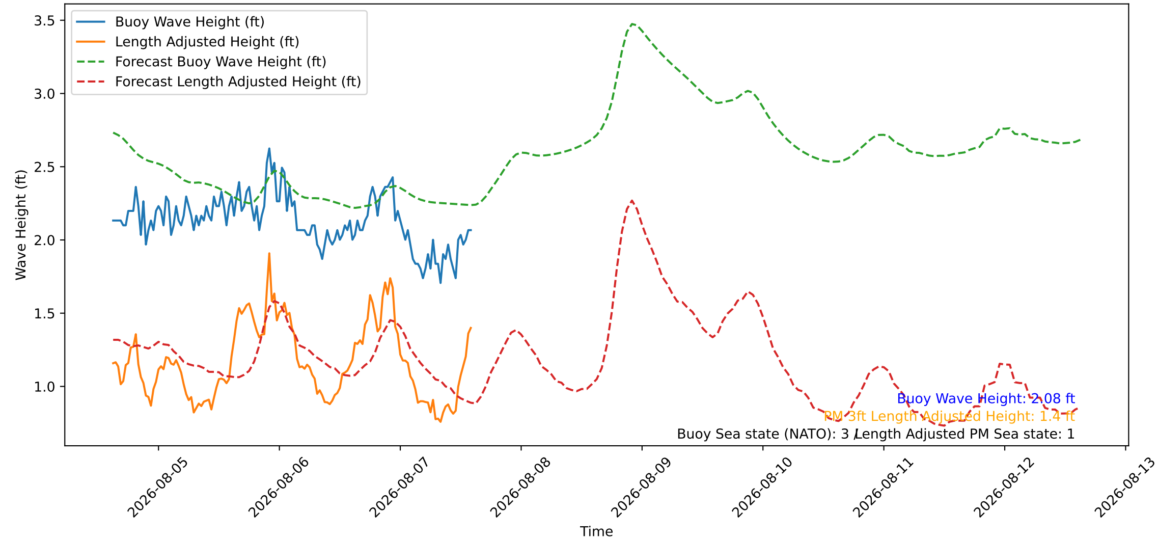
Wave Heights over Time for Green Beach at 2026-08-07 14:51:09
