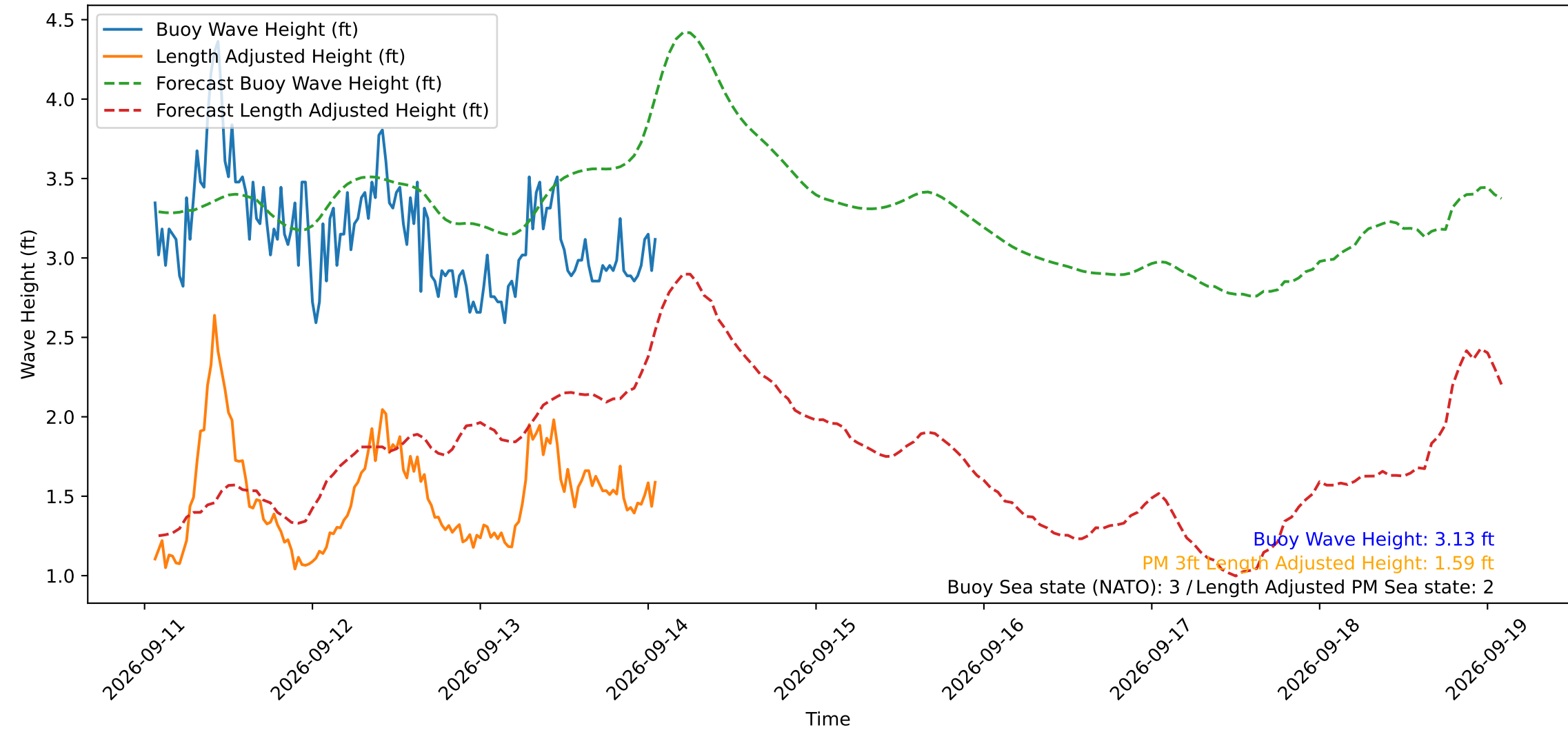
Wave Heights over Time for Oceanside Harbor at 2026-09-14 01:40:29
