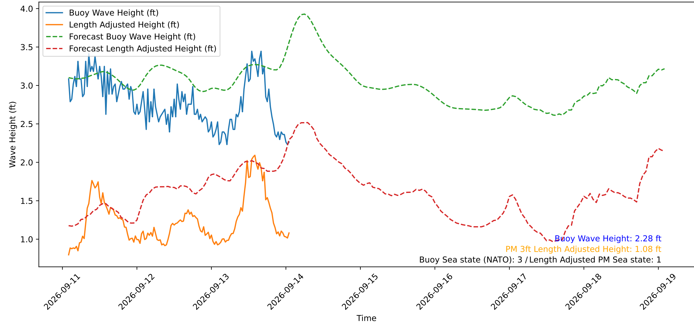
Wave Heights over Time for Red Beach at 2026-09-14 01:40:49
